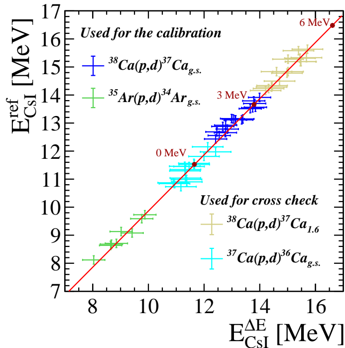
Figure 3.15: E_{CsI}^{Ref} vs. E_{CsI}^{\Delta E} scatter plot for CsI 16 of telescope 1. The data points from the ^{38}Ca(p,d)^{37}Ca_{g.s.} (blue), ^{35}Ar(p,d)^{34}Ar_{g.s.} (green), ^{37}Ca(p,d)^{36}Ca_{g.s.} (cyan) and ^{38}Ca(p,d)^{37}Ca_{1.6} MeV (yellow) reactions are shown. The linear fit (red curve) was done using the ^{38}Ca(p,d)^{37}Ca_{g.s.} and the ^{35}Ar(p,d)^{34}Ar_{g.s.} reactions. A linear fit describes well the data points from 0 to 6 MeV in excitation energy (written in red) in ^{36}Ca ( R^2 = 0.992 ).
