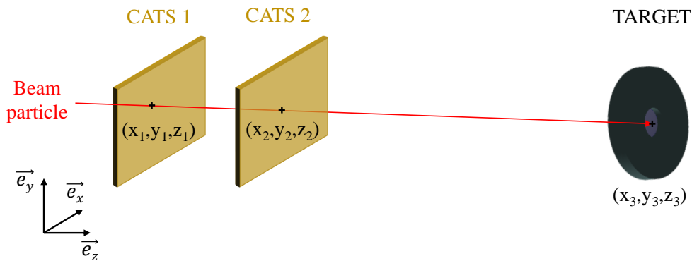
Figure 3.3: Scheme of the trajectory reconstruction of a beam particle with CATS.
