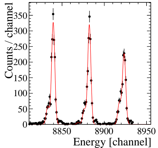
Figure 3.8: Raw energy spectra of one strip of one DSSD. This spectra was obtained after applying the data treatment presented in Section. 2.3 and keeping only multiplicity 1. The red line shows the fit of the three alpha peaks and their satellites.
