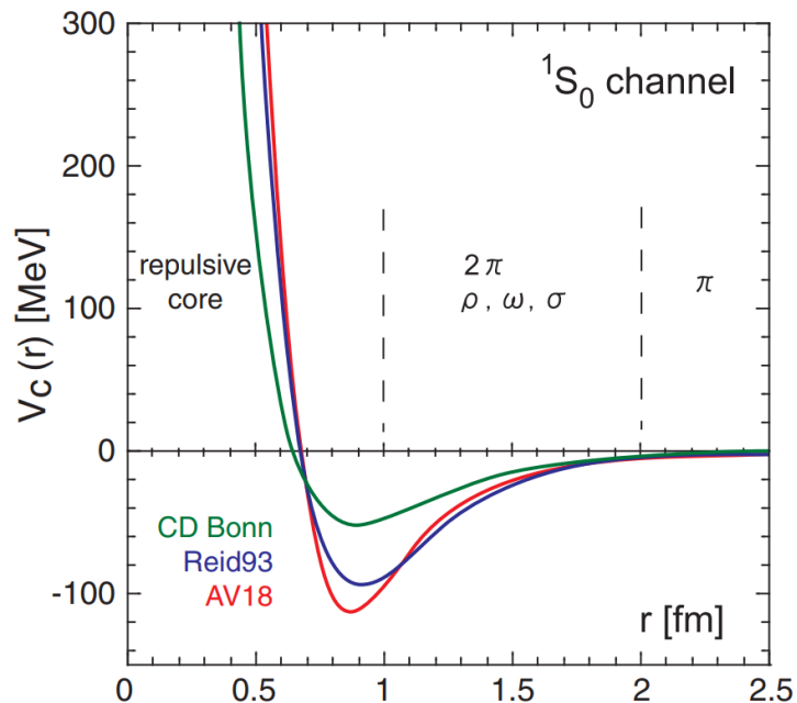
Figure 1.1: Three examples of NN interactions in the ^1S_0 channel. Figure from from Ref. [4].
