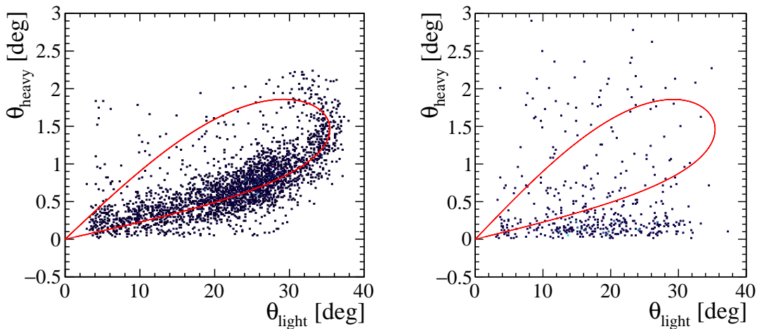
Figure 4.5: Correlation plots between the angle of the light particle \theta_{light} and the heavy outgoing particle \theta_{heavy} in the laboratory frame. Those plots are shown for the filled target (left) and for the empty target (right). In both plots, the theoretical line for the ^{37}\text{Ca}(p,d)^{36}\text{Ca} reaction is shown.
