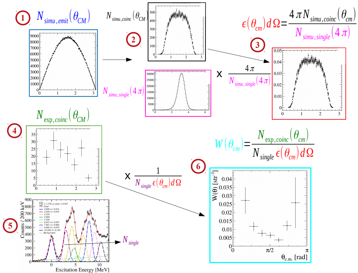
Figure 7.3: Method of extraction of the angular correlation function W(\theta_{cm}) . See text for details.
