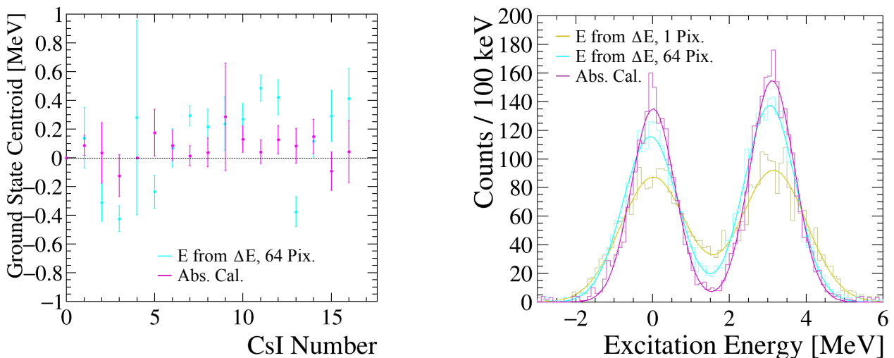
Figure 3.16: Left: Position of the centroid of the ground state peak in the excitation energy spectra of ^{36}Ca as a function of the CsI number obtained using two different calibration. Right: Excitation energy spectra of ^{36}Ca obtained with the "E from \Delta E " method with 1 pixel (yellow), 64 pixels (blue) and after the absolute calibration (purple).
