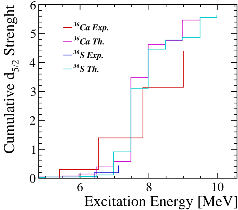
Figure 5.7: Cumulative d_{5/2} strength of ^{36}\text{Ca} and ^{36}\text{S} . Experimental results are compared to SM calculations.
