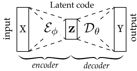
Figure 7.11: Encoder-Decoder architecture. The input x are first encoded to a latent representation z , which is then decoded to the output y .
