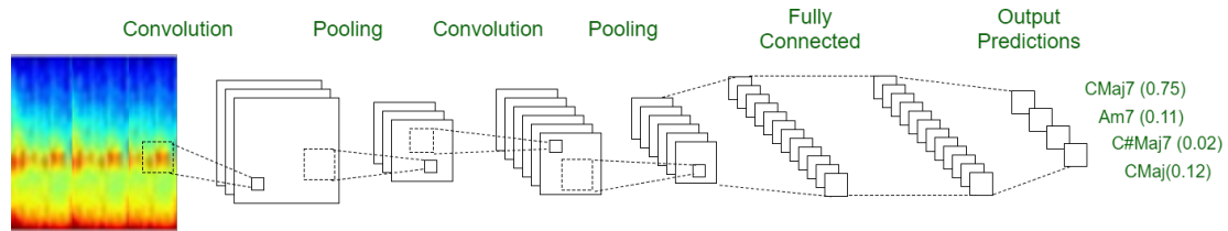
Figure 7.14: Example of a convolutional neural network for a task of ACE.
