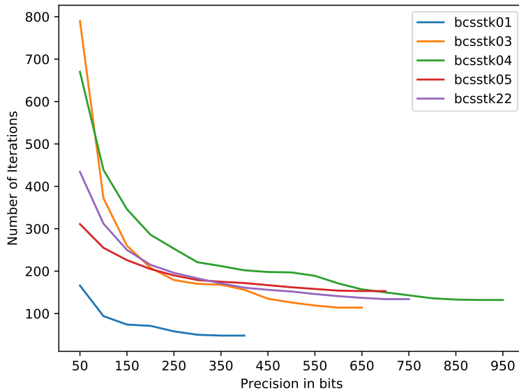
Figure 2.5: When applied on different MatrixMarket [24, 86] matrices, the number of iterations for the conjugate gradient (CG) algorithm decreases when precision augments. This experiment aims to show the usage of variable precision in a real-life application.
