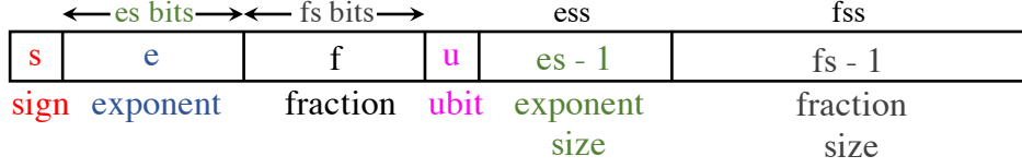
(a) Gustafson's Universal NUMBER (UNUM) Format
