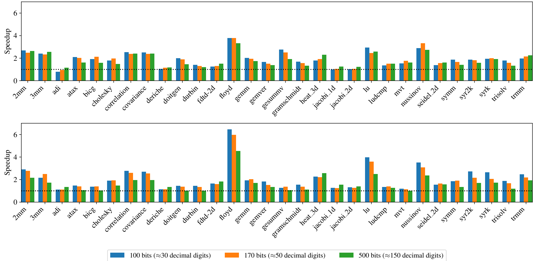
Figure 6.3: Speedup of vfloat<mpfr, ...> over the Boost library for multi-precision for the Polybench benchmark suite. vfloat<mpfr, ...> applications were compiled with optimization level -O1 and Boost with -O3 . The execution time reference taken are the best between compilations with and without Polly. Results are shown for two different machines: an Intel Xeon E5-2637v3 with 128GB of RAM (M1), and an Intel Xeon Gold 5220 with 96 GB of RAM (M2), respectively. Y-axes are shown with the same limit to ease comparisons between results in the two machines.
