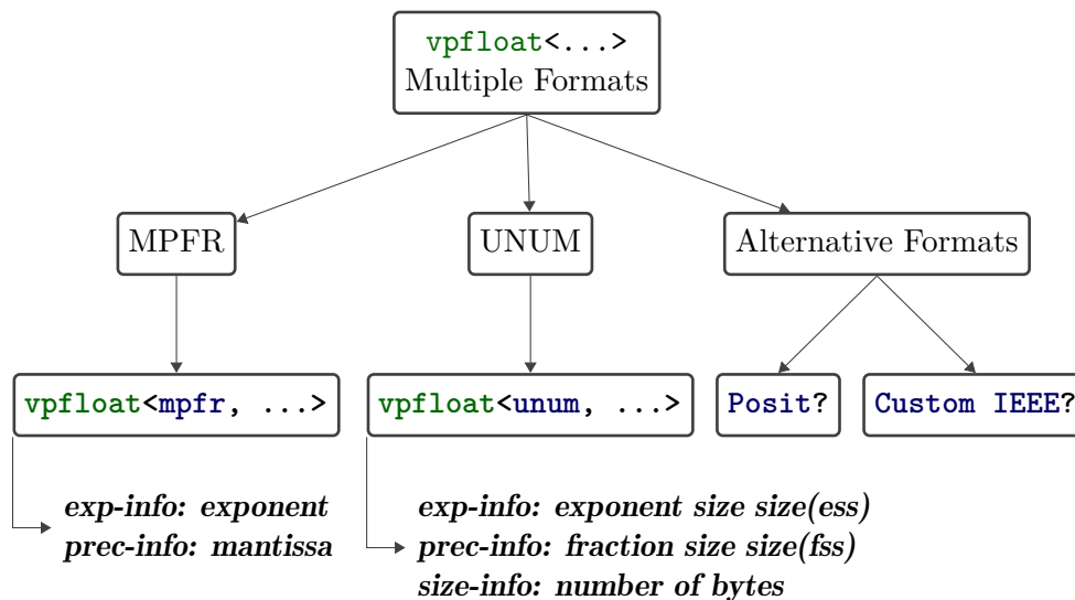
Figure 4.2: Summary of vpfloat multi-format schemes.
