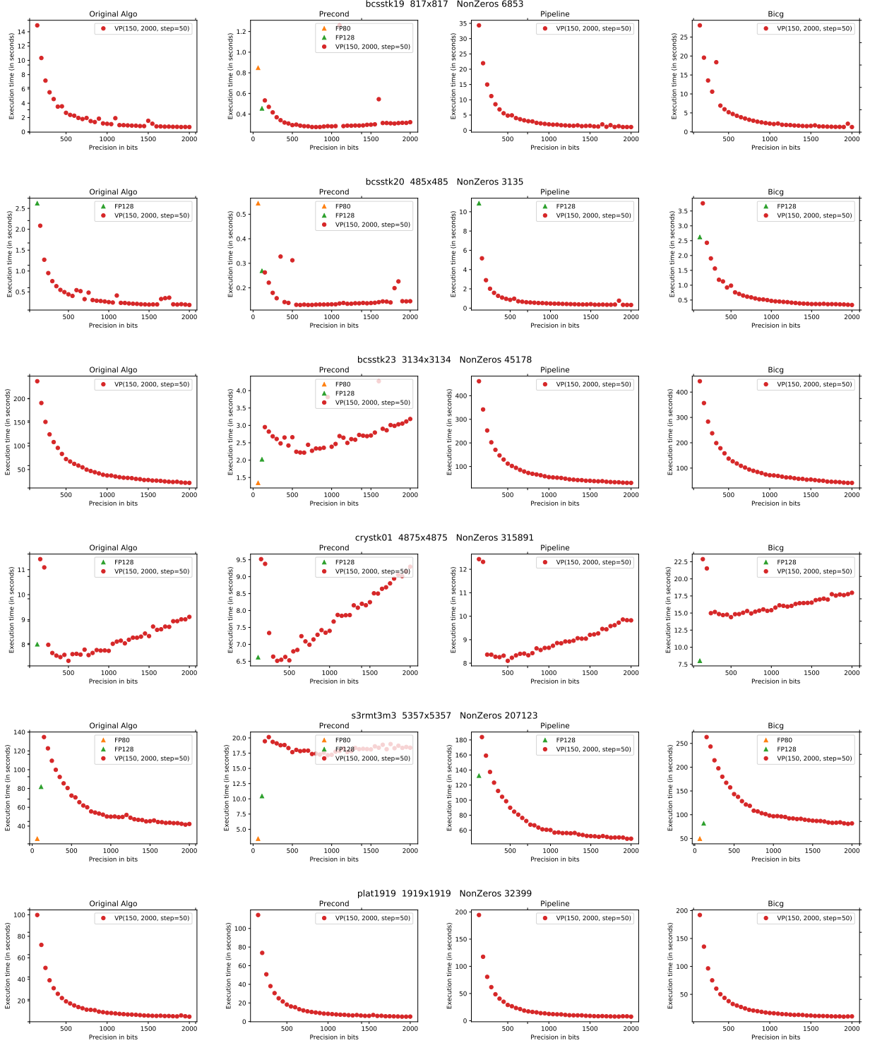
Figure 6.9: Execution time for CG variants with multiple formats with matrices bcsstk19 , bcsstk20 , bcsstk23 , crystk01 , s3rmt3m3 , and plat1919 from matrix market [24, 86]. Graph lines represent different matrices, and graph columns correspond to variants (from left to right: original CG, preconditioned CG, pipelined CG, BiCG). A missing type in a graph implies the algorithm did not converge. Results for double are not displayed.
