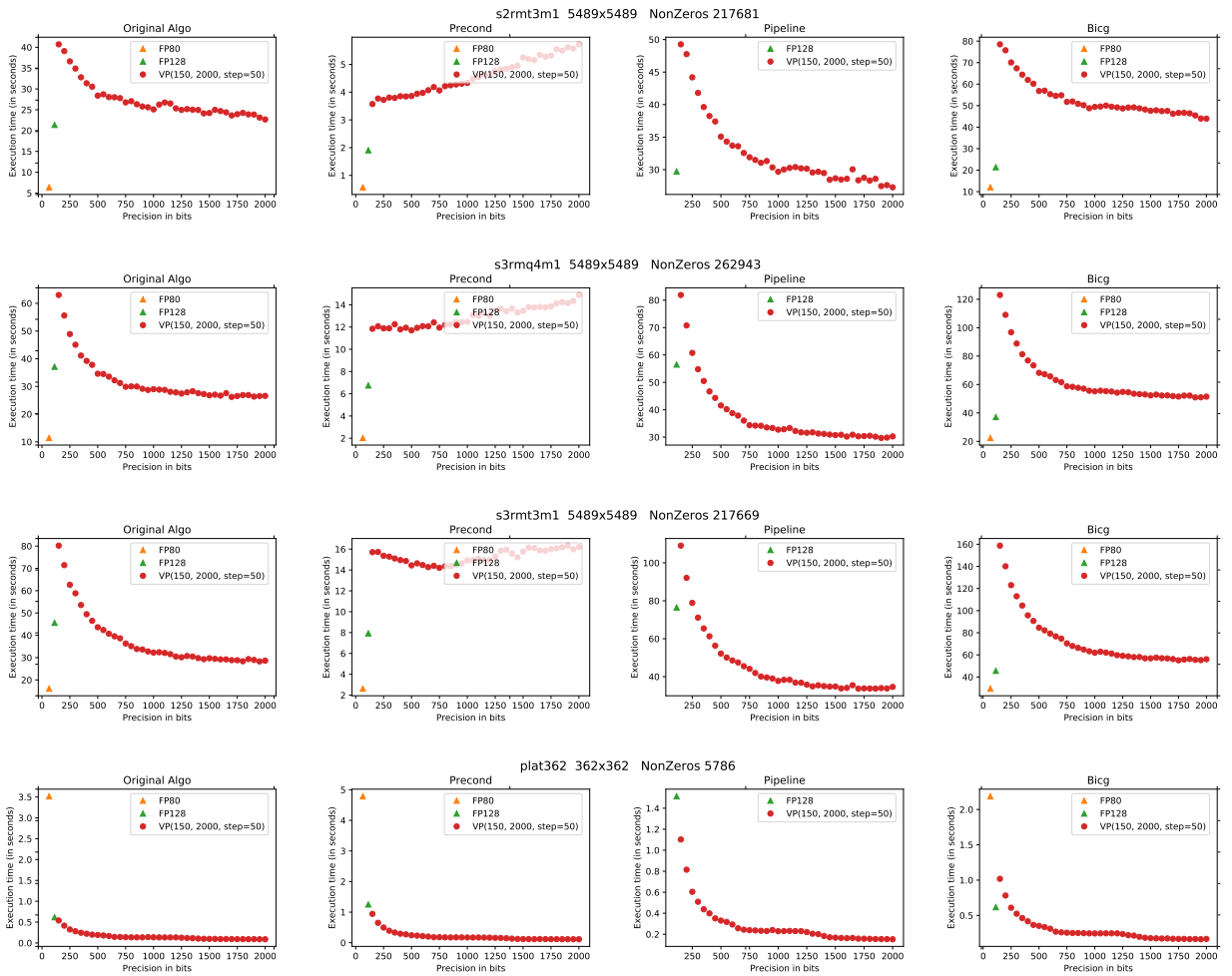
Figure B.5: Execution time for CG variants with multiple formats with matrices s2rmt3m1 , s3rmq4m1 , s3rmt3m1 , and plat362 from matrix market [24, 86]. Graph lines represent different matrices, and graph columns correspond to variants (from left to right: original CG, precond CG, pipelined CG, BiCG). A missing type in a graph implies the algorithm did not converge. Results for double are not displayed.
