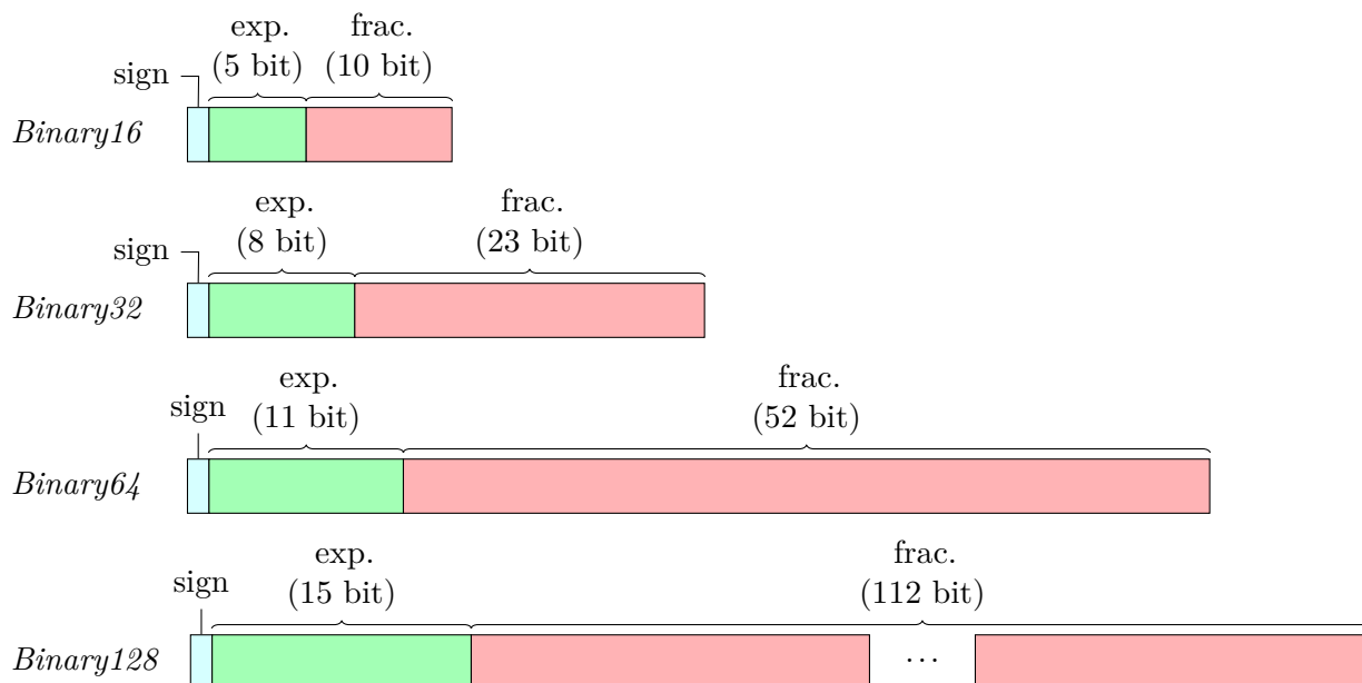
Figure 2.1: IEEE Formats (officially known as binary16 , binary32 , binary64 , and binary128 as defined by the standard).
