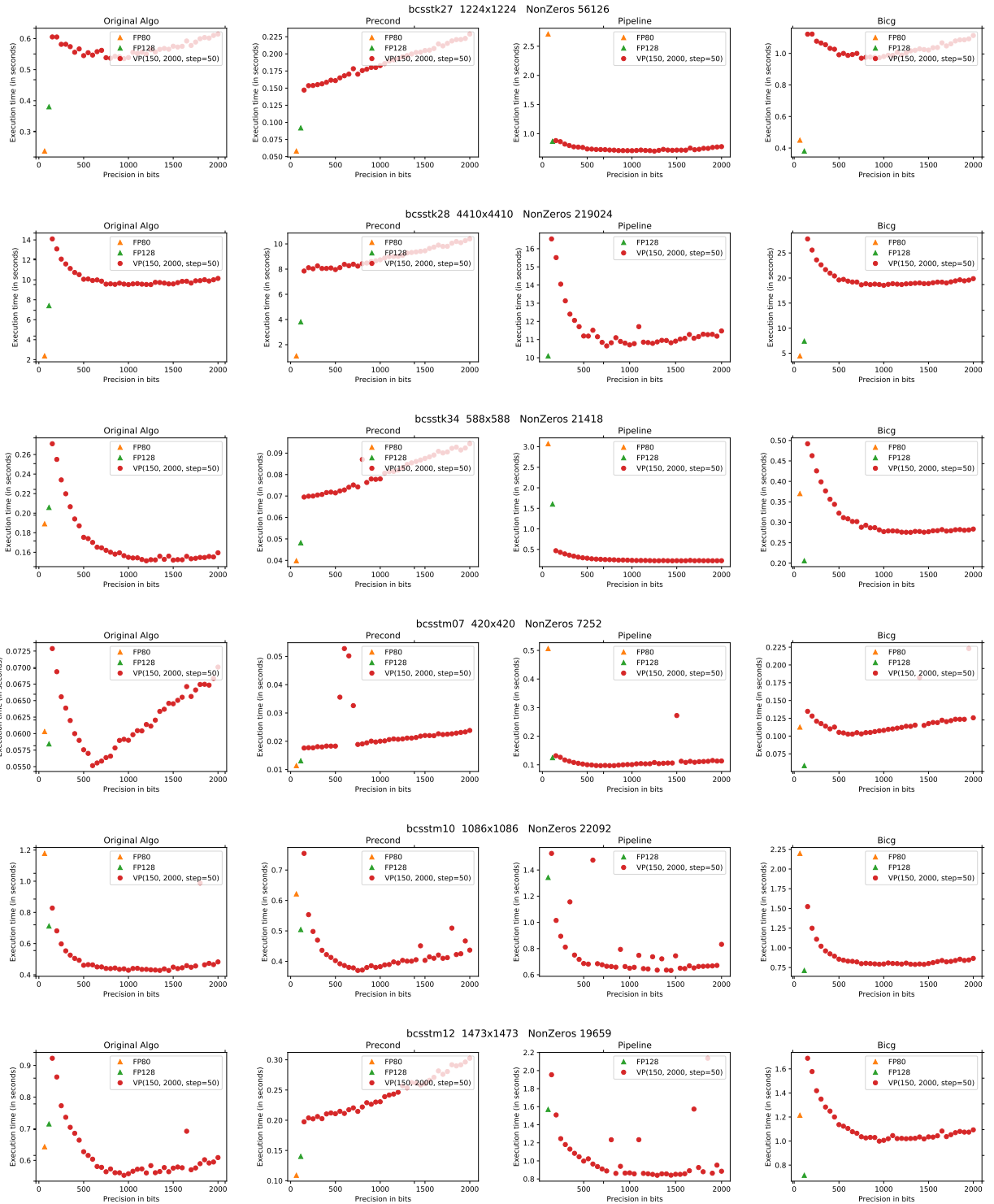
Figure B.3: Execution time for CG variants with multiple formats with matrices bcsstk27 , bcsstk28 , bcsstk34 , bcsstm07 , bcsstm10 , and bcsstm12 from matrix market [24, 86]. Graph lines represent different matrices, and graph columns correspond to variants (from left to right: original CG, precond CG, pipelined CG, BiCG). A missing type in a graph implies the algorithm did not converge. Results for double are not displayed.
