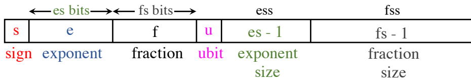
Figure 2.2: The Universal NUMBER (UNUM) Format
