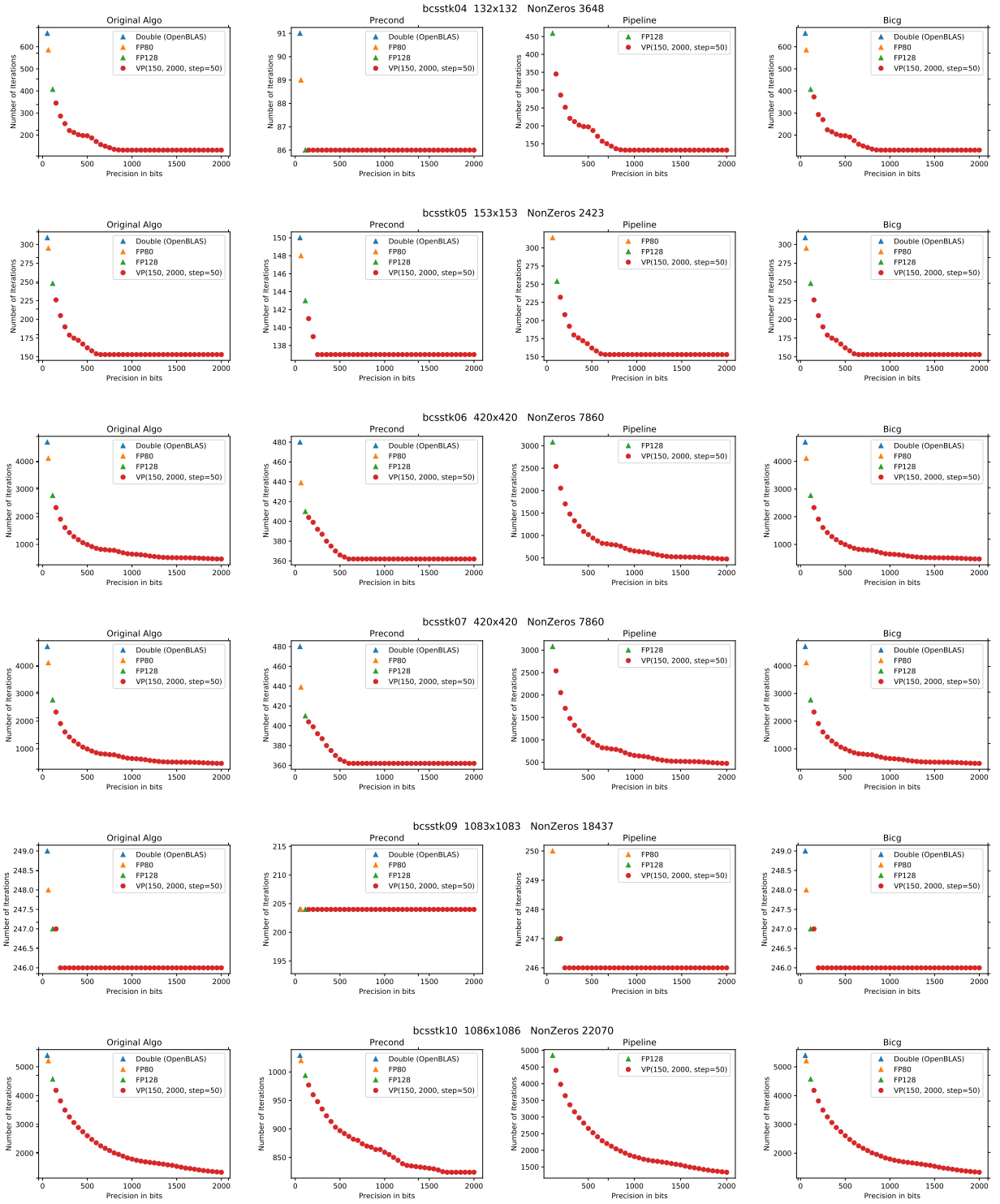
Figure A.1: CG variants with multiple formats with matrices bcstkt04 , bcstkt05 , bcstkt06 , bcstkt07 , bcstkt09 , and bcstkt10 from matrix market [24, 86]. Graph lines represent different matrices, and graph columns correspond to variants (from left to right: original CG, precond CG, pipelined CG, BiCG). Y-axes show the number of iterations needed to converge for precision in bits between 150 and 2000 with a \text{step}=50 . A missing type in a graph implies the algorithm did not converge.
