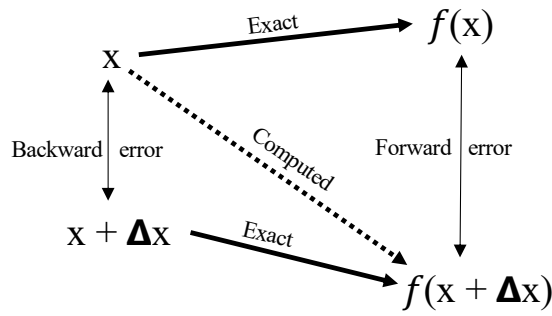
(a) Backward and forward errors [64]
