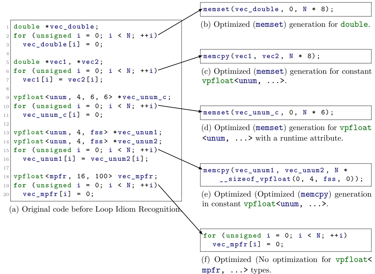
Listing 5.4: Loop idiom recognition pass for different types: double (5.4b, 5.4c), vfloat<unum, ...> (5.4d, 5.4e), and vfloat<mpfr, ...> (5.4f).
