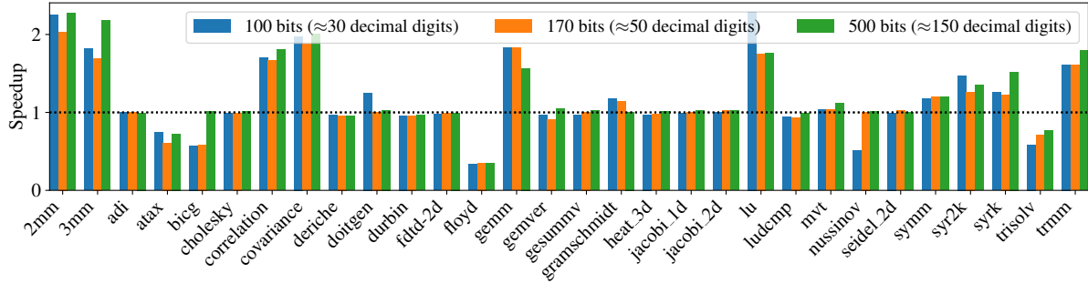
Figure 6.1: Speedup of Polly’s loop nest optimizer in Polybench compiled for vpfloat<mpfr, ...> types.
