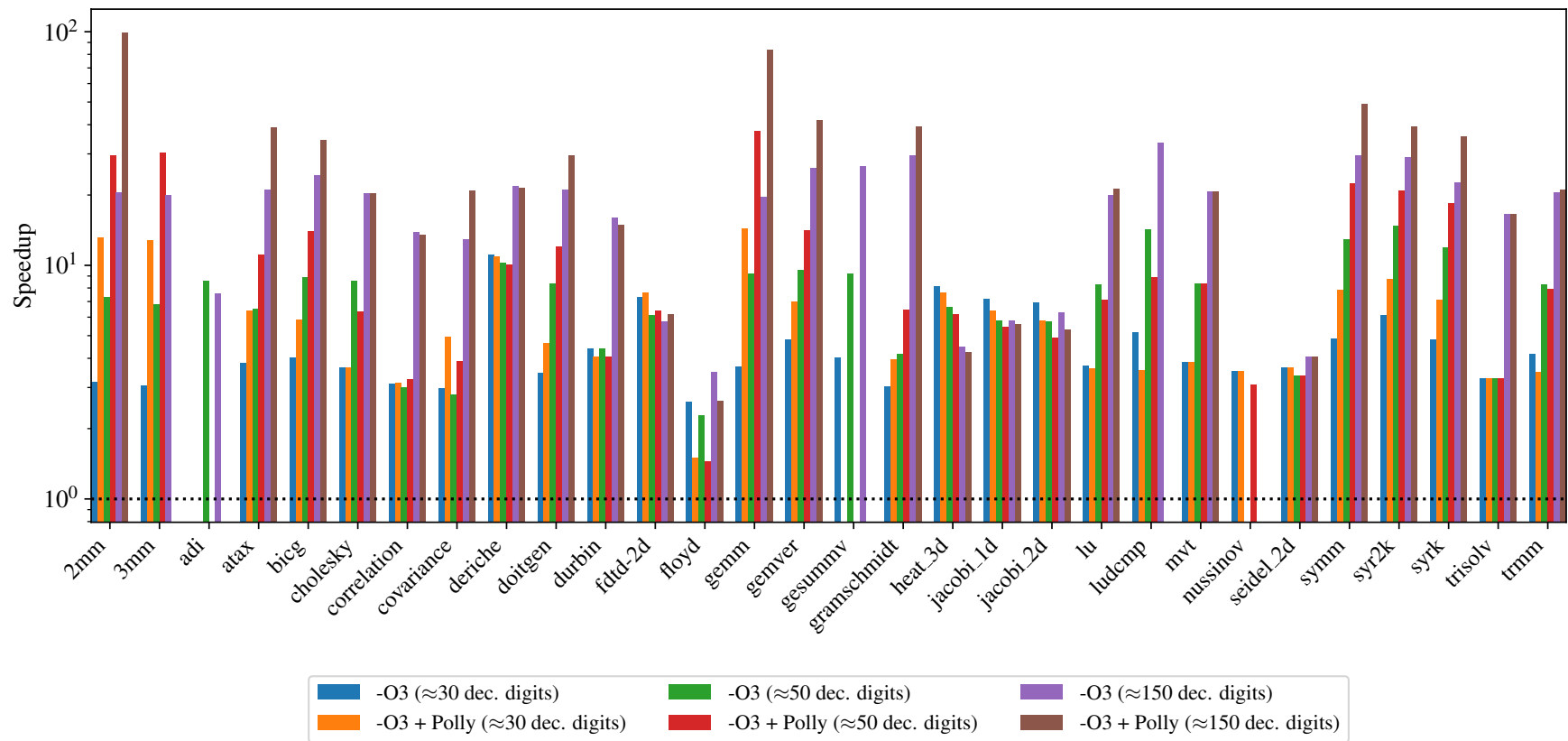
Figure 6.5: Speedup of vpfloat<unum, ...> over vpfloat<mpfr, ...> on the PolyBench suite
