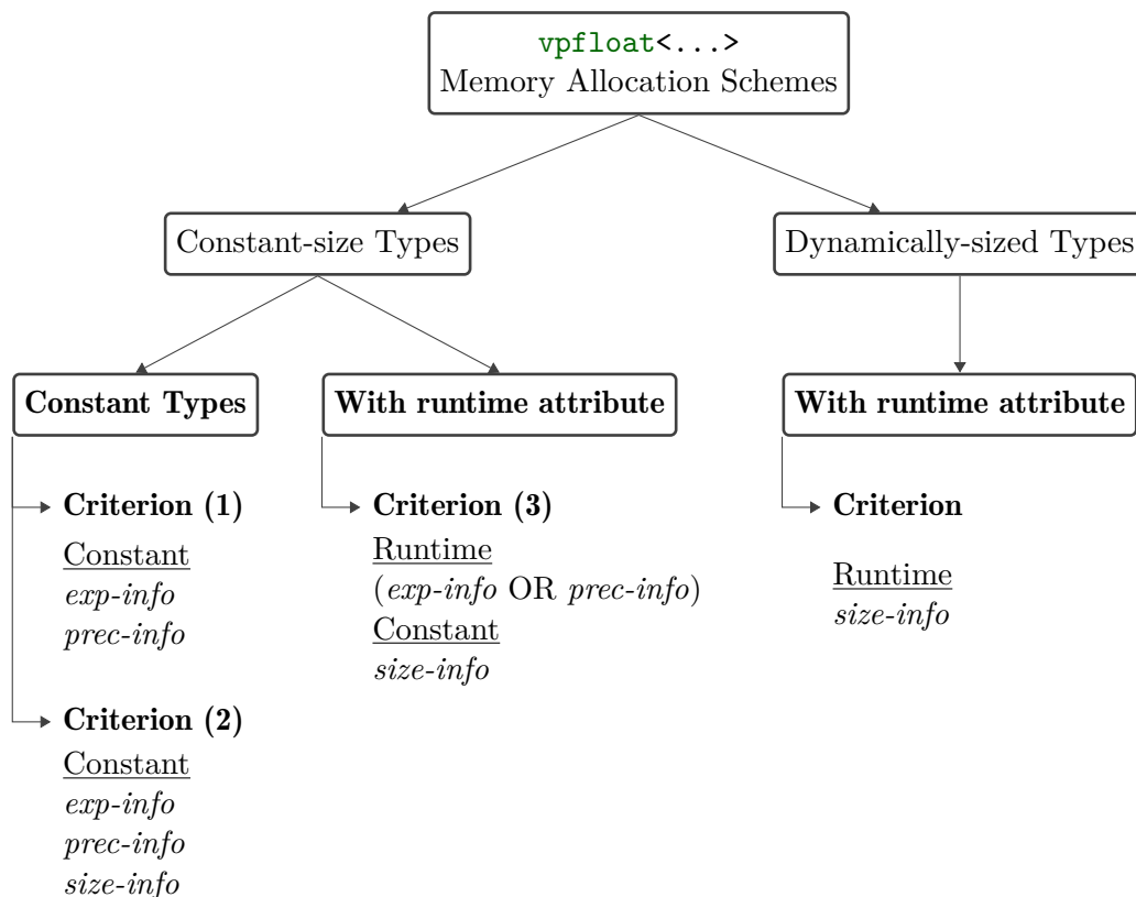
Figure 4.3: Memory Allocation Schemes for Constant-Size and Dynamically-Sized Types
