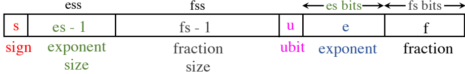
(b) Universal NUMBER (UNUM) Format as defined by Bocco et al. [21, 23].
