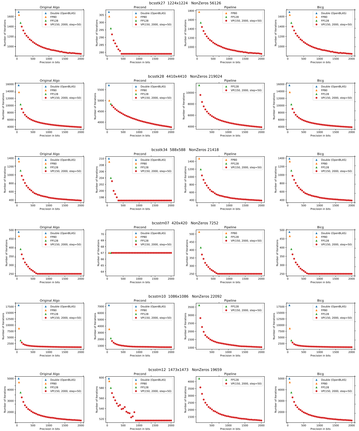
Figure A.3: CG variants with multiple formats with matrices bcsstk27 , bcsstk28 , bcsstk34 , bcsstm07 , bcsstm10 , and bcsstm12 from matrix market [24, 86]. Graph lines represent different matrices, and graph columns correspond to variants (from left to right: original CG, precond CG, pipelined CG, BiCG). Y-axes show the number of iterations needed to converge for precision in bits between 150 and 2000 with a \text{step}=50 . A missing type in a graph implies the algorithm did not converge.
