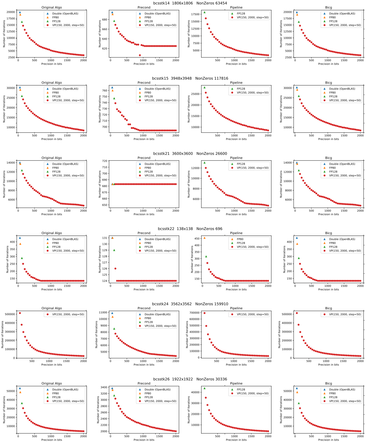
Figure A.2: CG variants with multiple formats with matrices bcsstk14 , bcsstk15 , bcsstk21 , bcsstk22 , bcsstk24 , and bcsstk26 from matrix market [24, 86]. Graph lines represent different matrices, and graph columns correspond to variants (from left to right: original CG, precond CG, pipelined CG, BiCG). Y-axes show the number of iterations needed to converge for precision in bits between 150 and 2000 with a step=50 . A missing type in a graph implies the algorithm did not converge.
