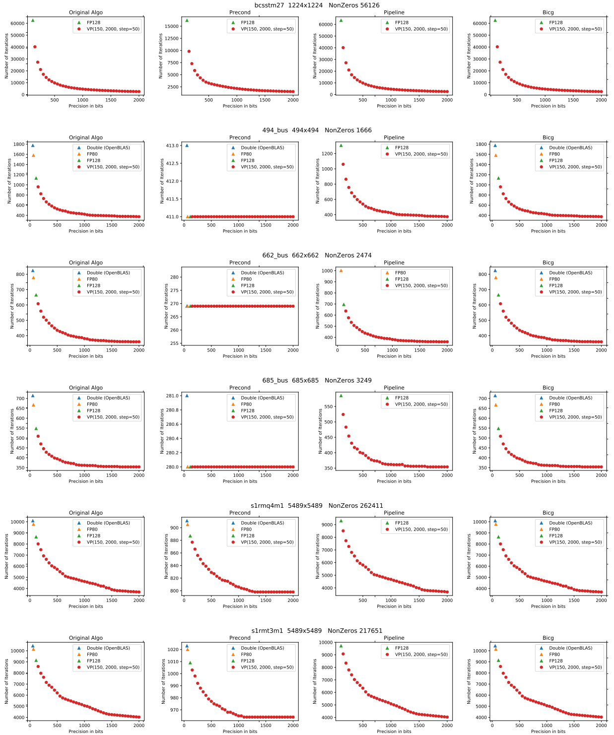
Figure A.4: CG variants with multiple formats with matrices bcsstm27 , 494_bus , 662_bus , 685_bus , s1rmq4m1 , and s1rmt3m1 from matrix market [24, 86]. Graph lines represent different matrices, and graph columns correspond to variants (from left to right: original CG, preconditioned CG, pipelined CG, BiCG). Y-axes show the number of iterations needed to converge for precision in bits between 150 and 2000 with a \text{step}=50 . A missing type in a graph implies the algorithm did not converge.
