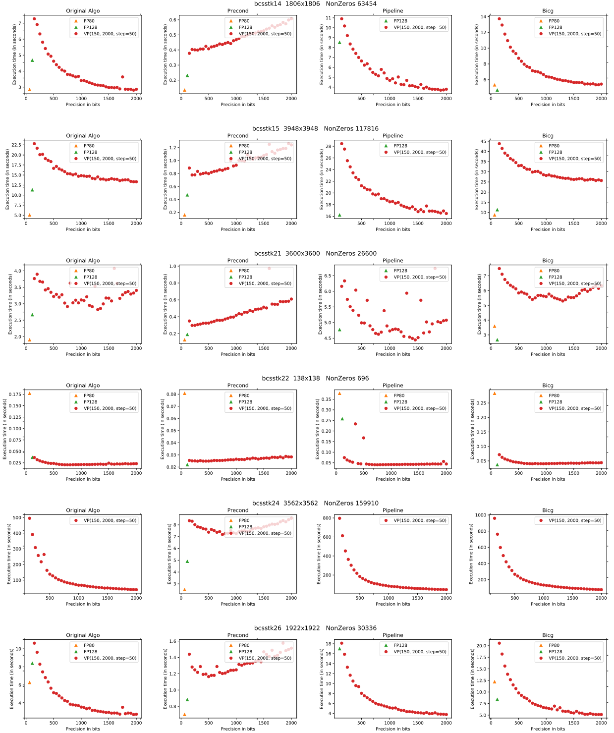
Figure B.2: Execution time for CG variants with multiple formats with matrices bcsstk14 , bcsstk15 , bcsstk21 , bcsstk22 , bcsstk24 , and bcsstk26 from matrix market [24, 86]. Graph lines represent different matrices, and graph columns correspond to variants (from left to right: original CG, precond CG, pipelined CG, BiCG). A missing type in a graph implies the algorithm did not converge. Results for double are not displayed.
