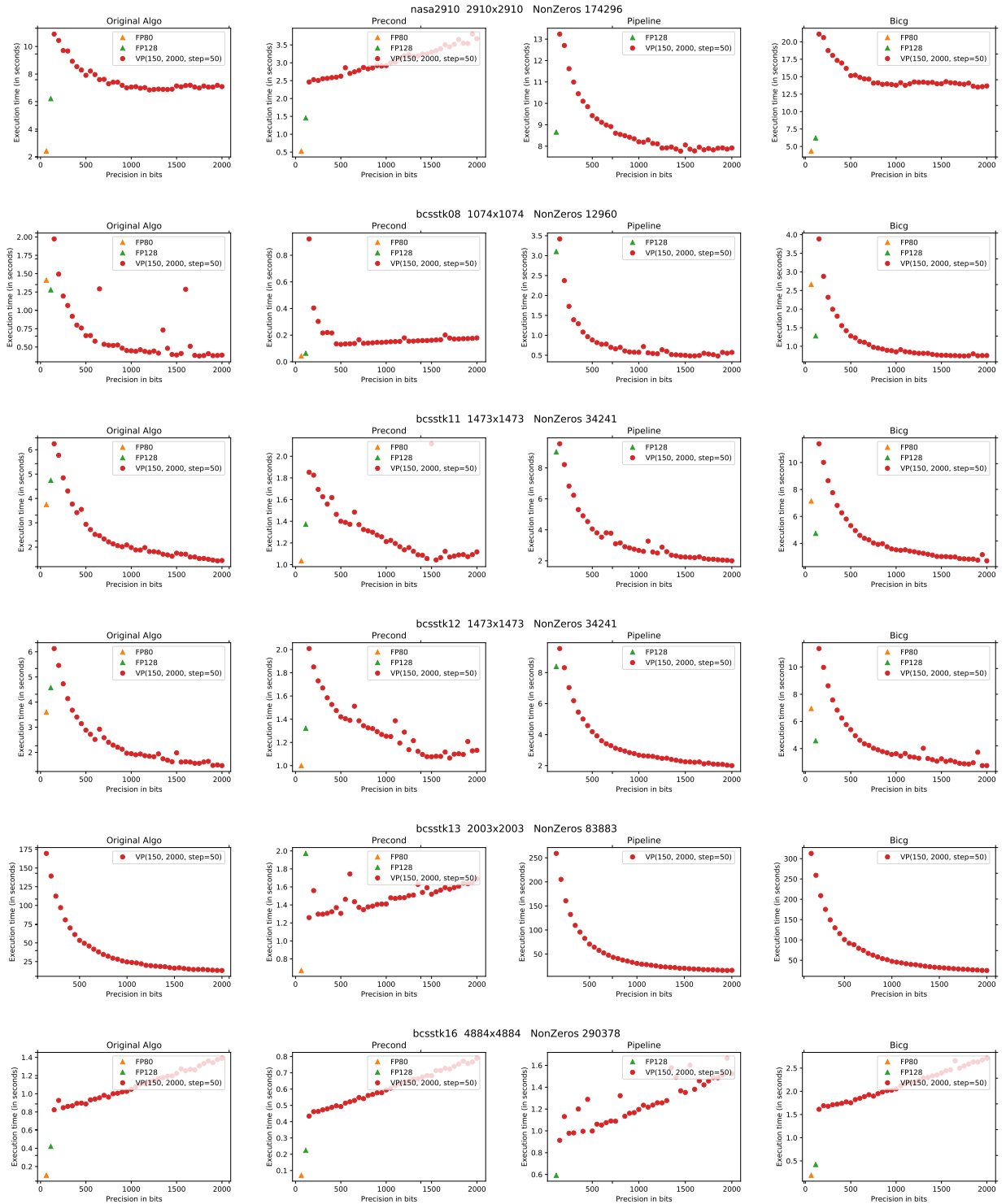
Figure 6.8: Execution time for CG variants with multiple formats with matrices nasa2910 , bcsstk08 , bcsstk11 , bcsstk12 , bcsstk13 , and bcsstk16 from matrix market [24, 86]. Graph lines represent different matrices, and graph columns correspond to variants (from left to right: original CG, precond CG, pipelined CG, BiCG). A missing type in a graph implies the algorithm did not converge. Results for double are not displayed.
