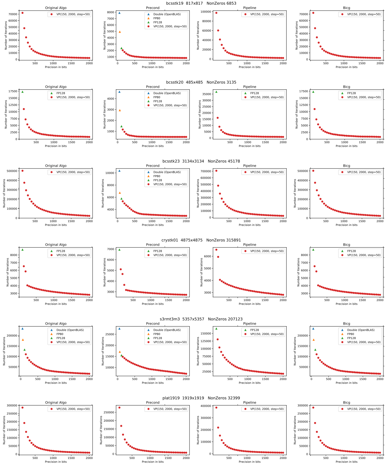
Figure 6.7: CG variants with multiple formats with matrices bcsstk19 , bcsstk20 , bcsstk23 , crystk01 , s3rmt3m3 , and plat1919 from matrix market [24, 86]. Graph lines represent different matrices, and graph columns correspond to variants (from left to right: original CG, precond CG, pipelined CG, BiCG). Y-axes show the number of iterations needed to converge for precision in bits between 150 and 2000 with a \text{step}=50 . A missing type in a graph implies the algorithm did not converge.
