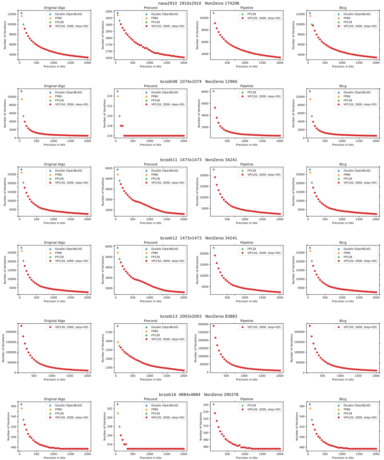
Figure 6.6: CG variants with multiple formats with matrices nasa2910 , bcsstk08 , bcsstk11 , bcsstk12 , bcsstk13 , and bcsstk16 from matrix market [24, 86]. Graph lines represent different matrices, and graph columns correspond to variants (from left to right: original CG, precond CG, pipelined CG, BiCG). Y-axes show the number of iterations needed to converge for precision in bits between 150 and 2000 with a \text{step}=50 . A missing type in a graph implies the algorithm did not converge.
