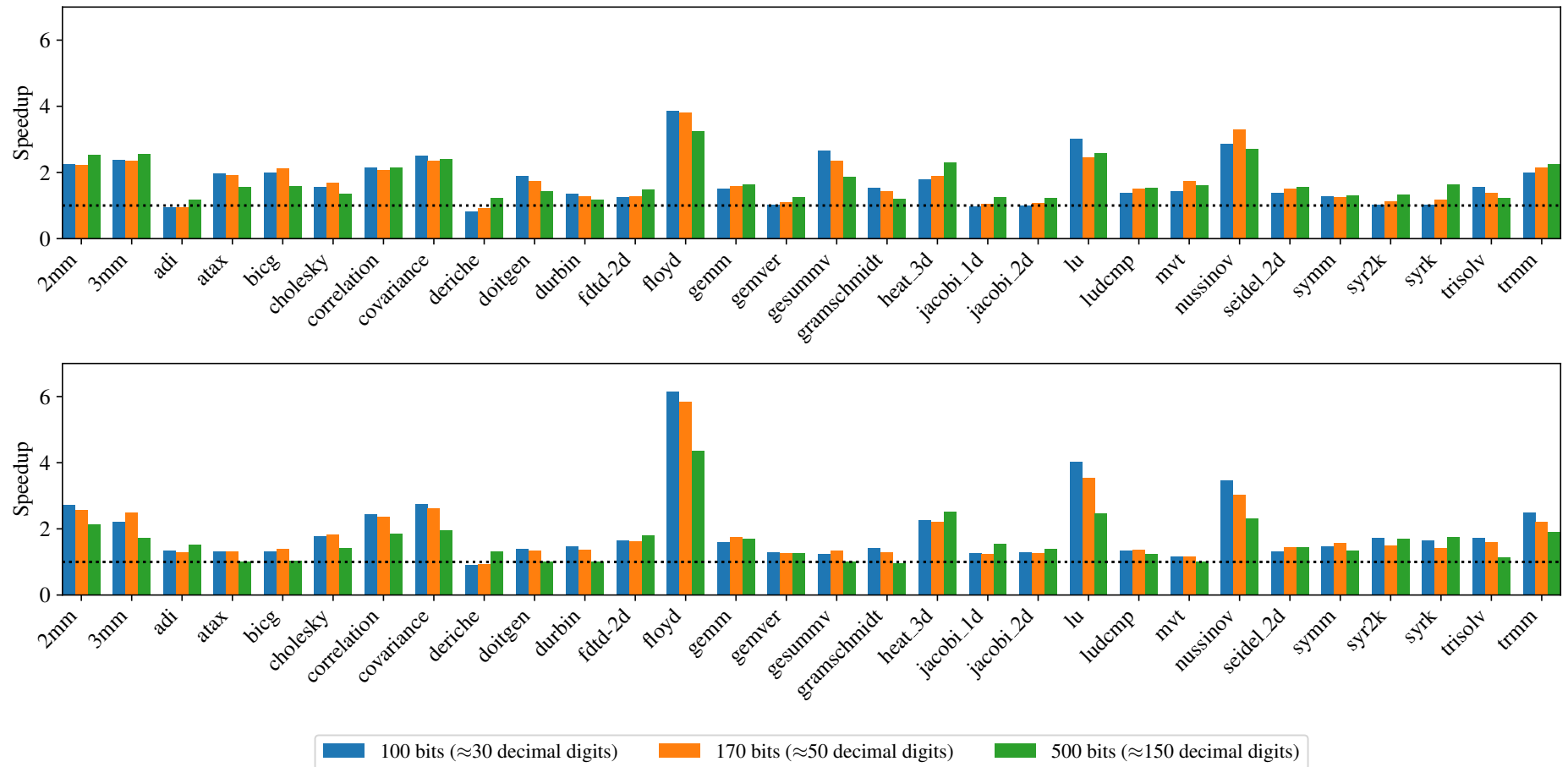
Figure 6.2: Speedup of vpfloat<mpfr, ...> over the Boost library for multi-precision for the Polybench benchmark suite, and compiled with optimization level -O3 . The execution time reference taken are the best between compilations with and without Polly. Results are shown for two different machines: an Intel Xeon E5-2637v3 with 128GB of RAM (M1), and an Intel Xeon Gold 5220 with 96 GB of RAM (M2), respectively. Y-axes are shown with the same limits to ease comparisons between results in the two machines.
