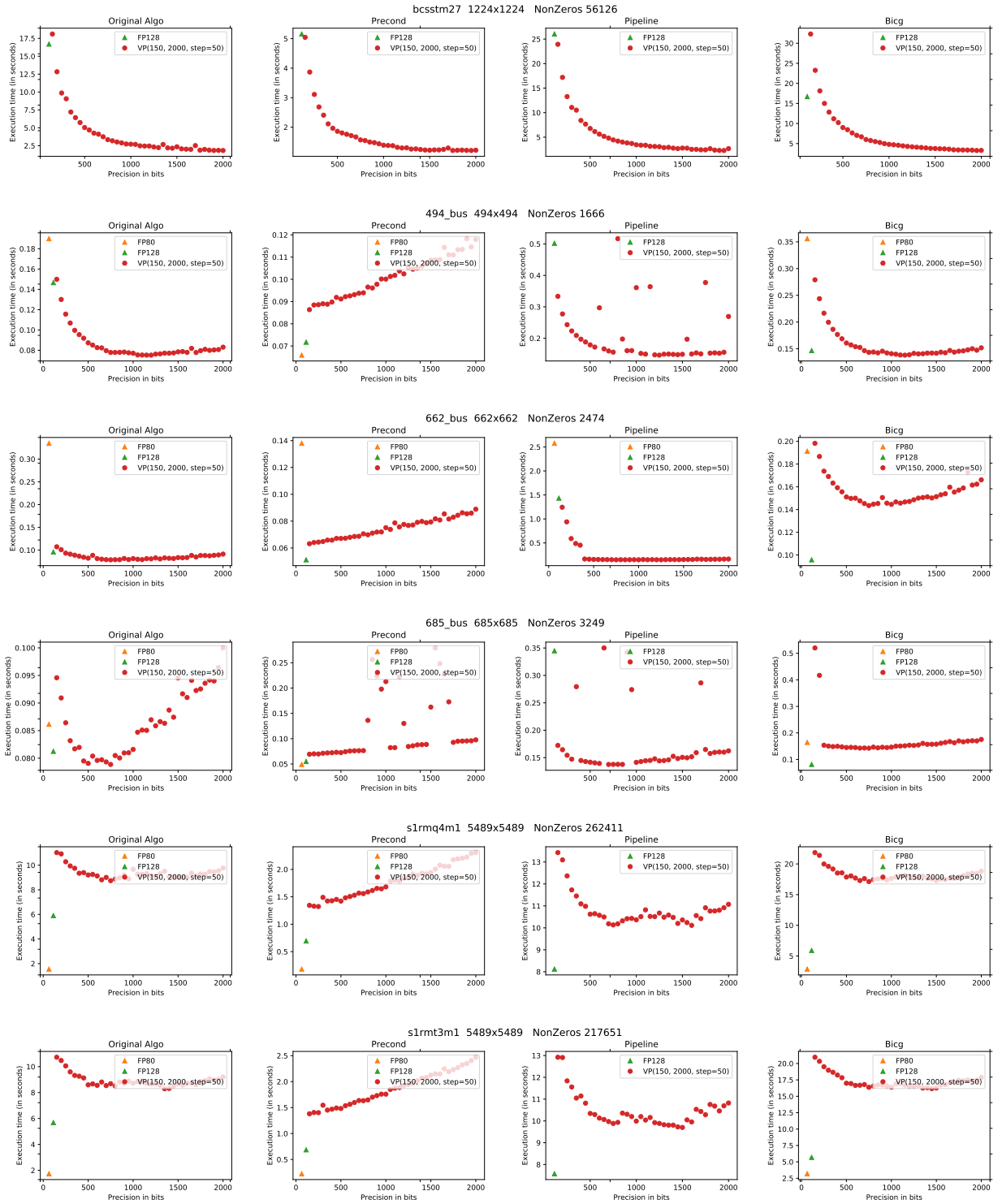
Figure B.4: Execution time for CG variants with multiple formats with matrices bcsstm27 , 494_bus , 662_bus , 685_bus , s1rmq4m1 , and s1rmt3m1 from matrix market [24, 86]. Graph lines represent different matrices, and graph columns correspond to variants (from left to right: original CG, preconditioned CG, pipelined CG, BiCG). A missing type in a graph implies the algorithm did not converge. Results for double are not displayed.
