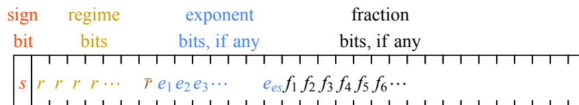
Figure 2.3: The Posit Format
