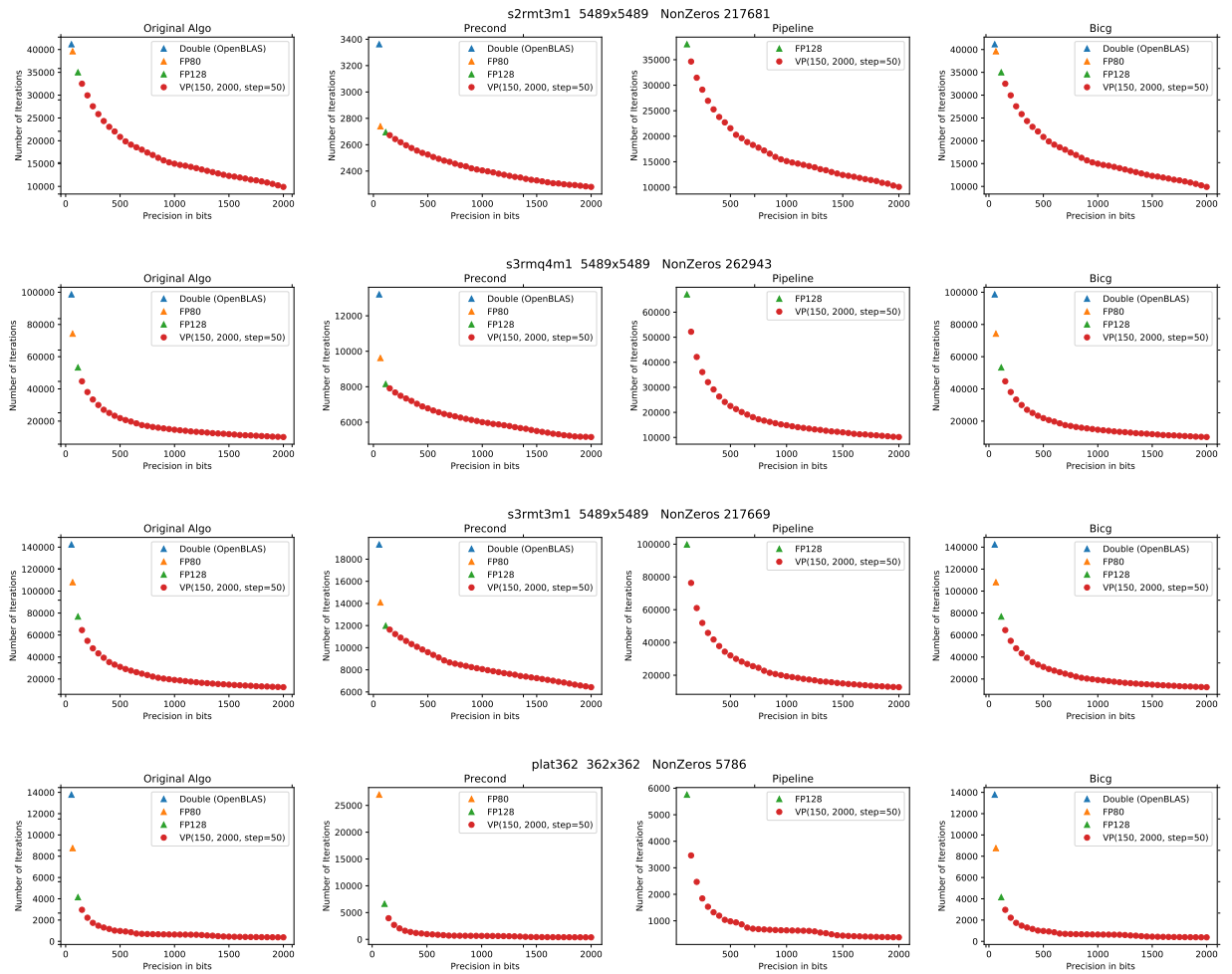
Figure A.5: CG variants with multiple formats with matrices s2rmt3m1 , s3rmq4m1 , s3rmt3m1 , and plat362 from matrix market [24, 86]. Graph lines represent different matrices, and graph columns correspond to variants (from left to right: original CG, precond CG, pipelined CG, BiCG). Y-axes show the number of iterations needed to converge for precision in bits between 150 and 2000 with a step=50. A missing type in a graph implies the algorithm did not converge.
