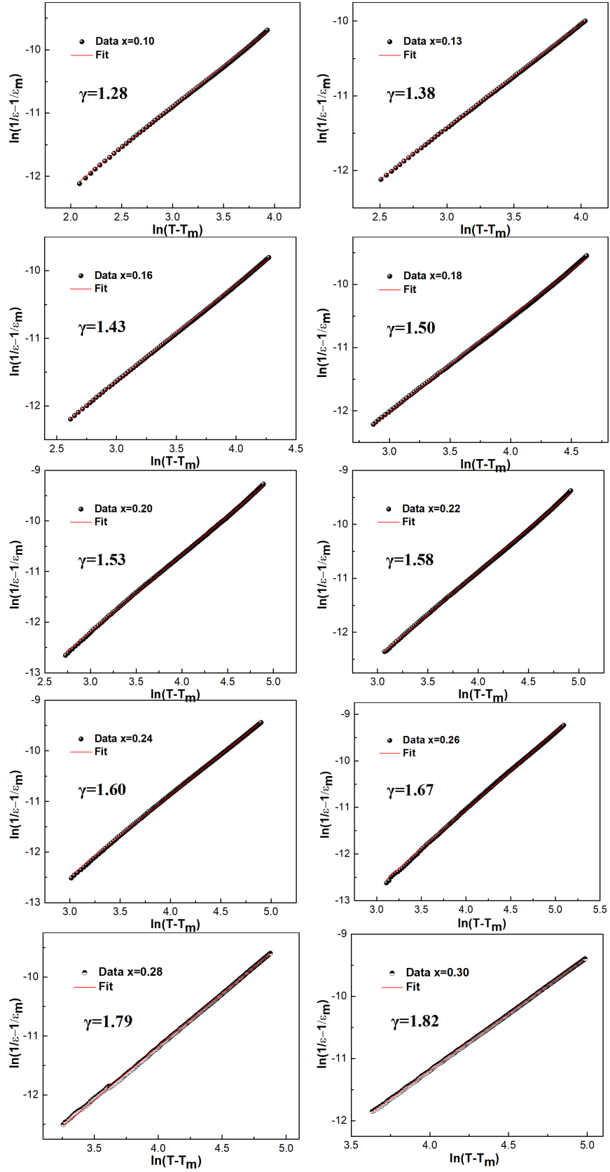
Figure 3.15 Plots of \ln(1/\epsilon-1/\epsilon_m) vs. \ln(T-T_m) for the (0.76-x)\text{BF}-0.24\text{PT}-x\text{BST} ceramics.
