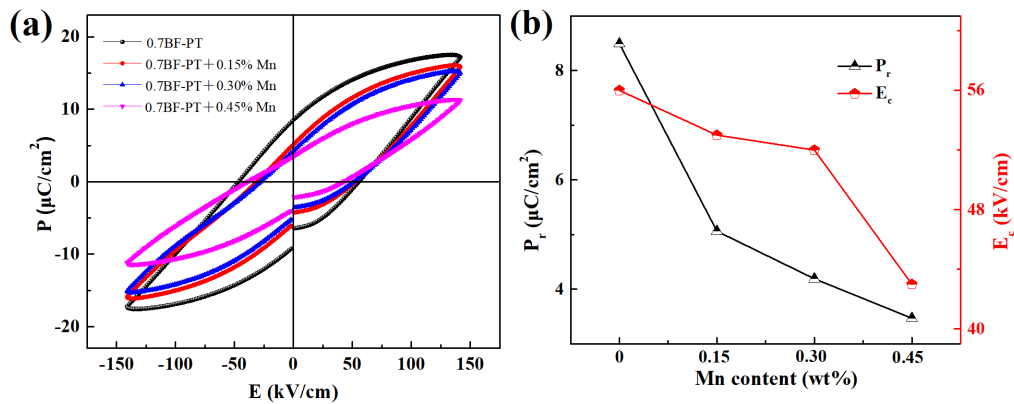
Figure 5.9 (a) The P - E loops of 0.7BF-0.3PT+ x wt%MnCO 3 ( x=0, 0.15, 0.3, 0.45 ) ceramics; (b) P_r and E_c as a function of Mn content.
