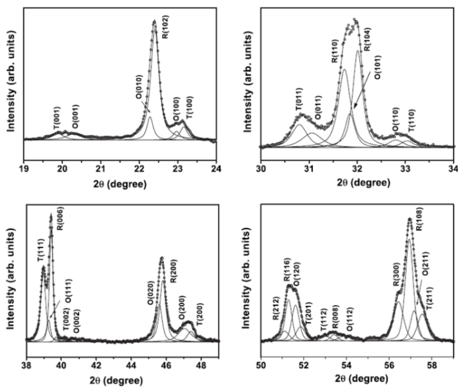
Figure 1.12 XRD pattern of 72BF-28PT ceramics, in which the dots are the experimental data and the solid lines are the fitting data [92] .
