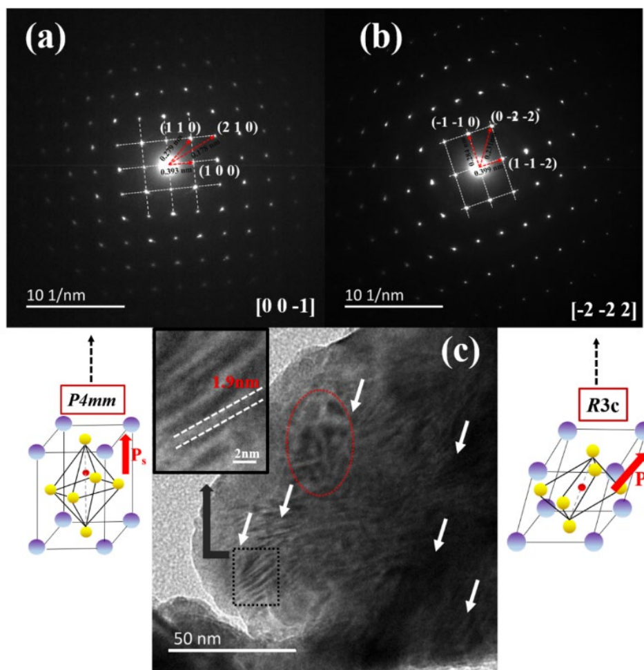
Figure 3.18 (a)(b) SAED patterns taken from different grains of BF-PT-0.2BST ceramics correspond to tetragonal and rhombohedral phase, respectively; (c) TEM bright-field images of domain configurations of BF-PT-0.2BST ceramics.
