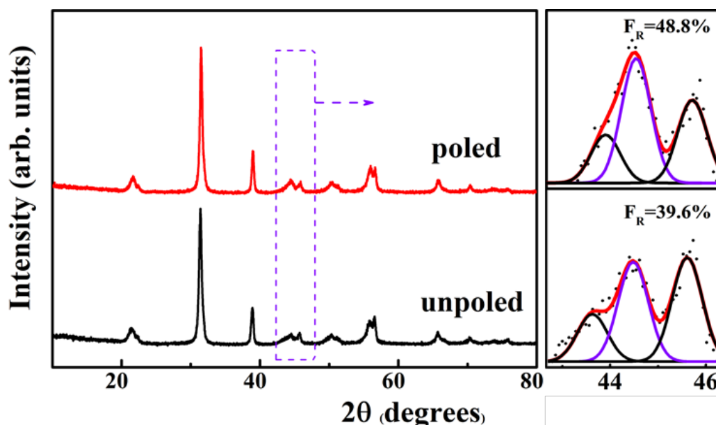
Figure 4.2 XRD pattern of the poled and unpoled 0.6BF-0.24PT-0.16BST ceramics.
