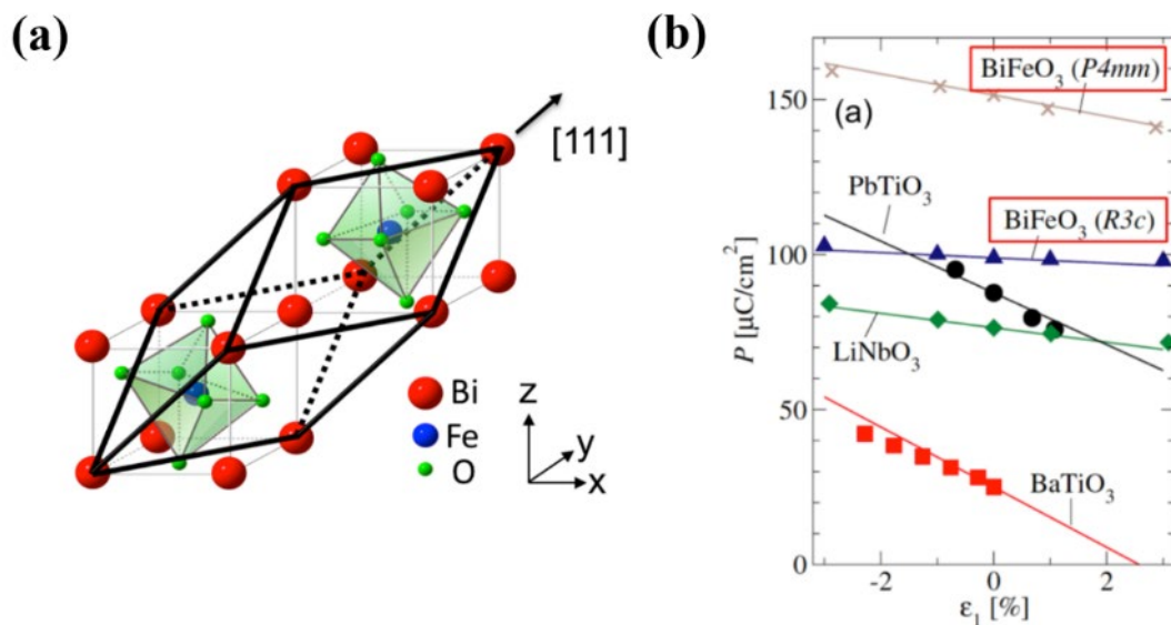
Figure 1.9 (a) Structure of \text{BiFeO}_3 [75]; (b) The polarization for \text{BiFeO}_3 , \text{BaTiO}_3 , \text{PbTiO}_3 and \text{LiNbO}_3 as a function of epitaxial strain [76].
