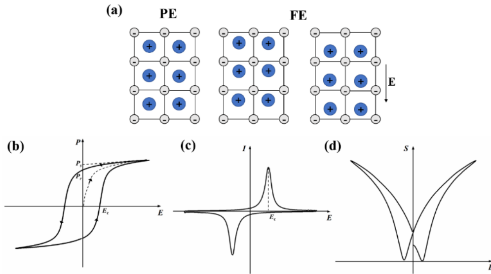
Figure 1.1 (a) Formation of dipole moments: paraelectric (PE) state and ferroelectric (FE) states (before and after the application of an external field); (b) Typical hysteresis loops; (c) I-E loops; (d) Bipolar strain-electric-field curve.
