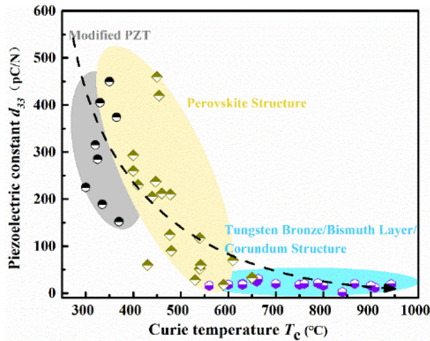
Figure 1.7 The d_{33} and T_c for different kinds of high-temperature piezoelectric ceramics.
