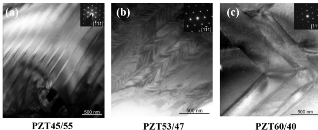
Figure 1.3 Ferroelectric domain configurations of \text{Pb}(\text{Zr}_{1-x}\text{Ti}_x)\text{O}_3 piezoelectric ceramics with different content of Zr/Ti [18] .
