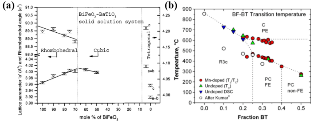
Figure 17 (a) Variation of lattice parameters for the BF-BT system [119] ; (b) Revised phase diagram for the BF-BT system [120] .
