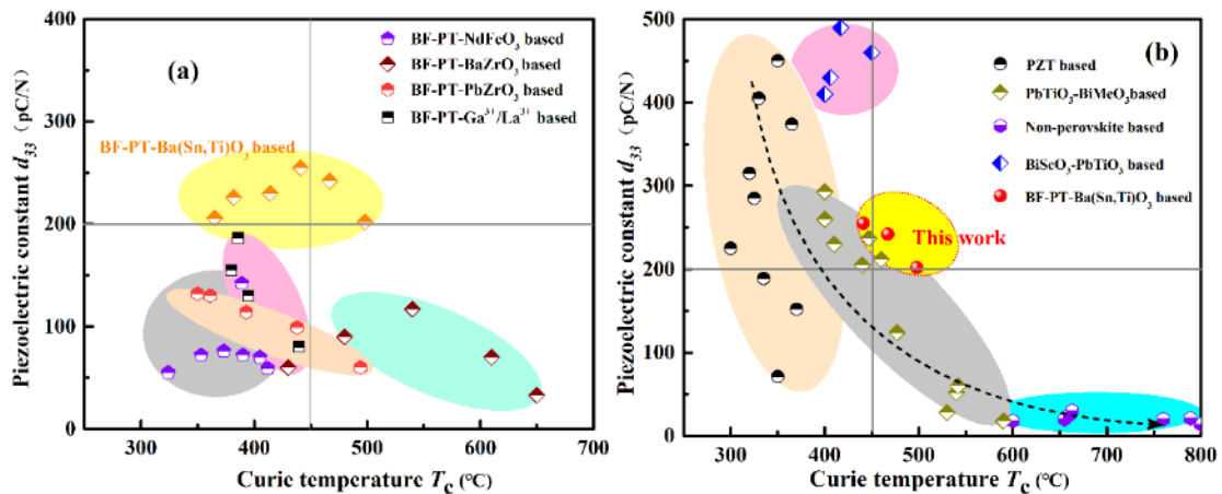
Figure 3.19 A comparison of the d_{33} and T_c values among (a) the modified BF-PT-based ceramics reported previously; and (b) the canonical high Curie temperature ferroelectric ceramics.
