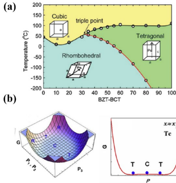
Figure 1.5 (a) The phase diagram of BZT-BCT based ceramics [22] ; (b) The (1-10) projection of the free energy profiles for the BZT-BCT based ceramics at the tricritical point and the corresponding 2D free energy profiles [23] .
