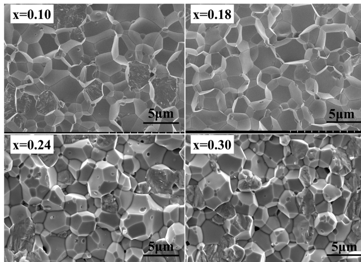
Figure 3.11 SEM images of the fresh fracture surfaces of (0.76-x)\text{BF}-0.24\text{PT}-x\text{BST} ceramics ( x=0.1, 0.18, 0.24, 0.30 ).
