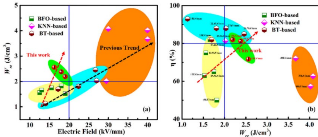
Figure 1.18 A comparison of energy storage properties ( W_{re} and \eta ) among the canonical lead-free ferroelectric ceramics [131].
