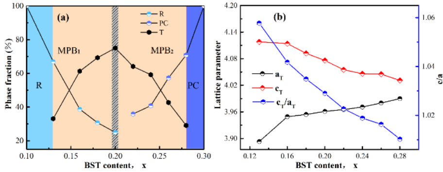
Figure 3.10 Phase fraction and lattice parameters of (0.76-x)\text{BF}-0.24\text{PT}-x\text{BST} ceramics.
