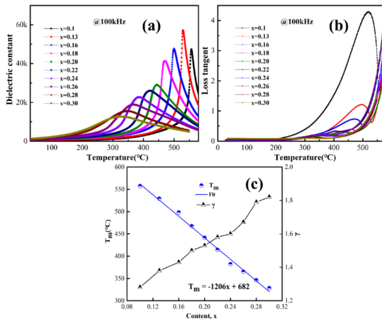
Figure 3.13 (a) Dielectric constant; (b) loss tangent as a function of temperature for (0.76-x)\text{BF}-0.24\text{PT}-x\text{BST} ceramics; and (c) T_m and \gamma values as a function of x .
