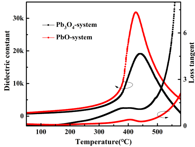
Figure 3.3 The temperature dependencies of \epsilon_r and \tan\delta for the ceramics with different lead raw materials.
