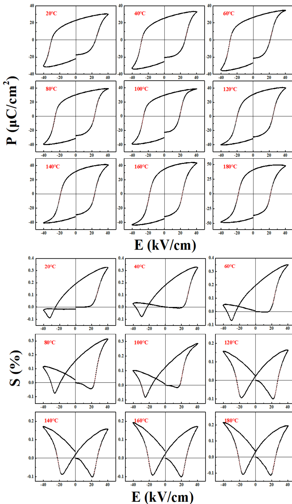
Figure 4.5 The temperature-dependent of the hysteresis ( P - E ) loops and the bipolar S - E loops for the poled 0.6BF-0.24PT-0.16BST ceramics.
