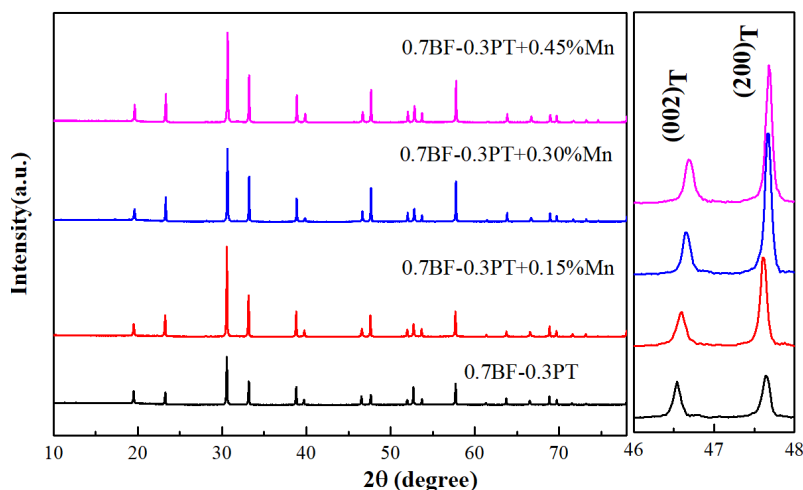
Figure 5.1 XRD pattern of the 0.7\text{BF}-0.3\text{PT}+x\text{wt}\%\text{MnCO}_3 ( x=0, 0.15, 0.3, 0.45 ) ceramics.
