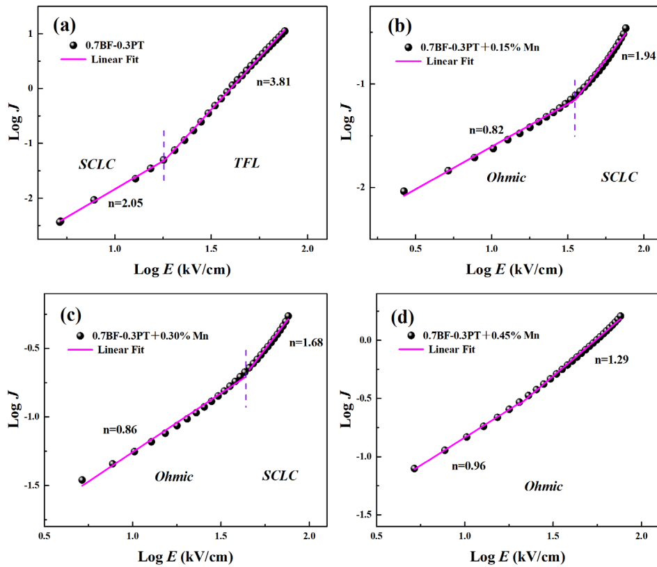
Figure 5.11 Plots of \log J vs. \log E for the 0.7BF-0.3PT+ x wt%MnCO 3 ( x=0, 0.15, 0.3, 0.45 ) ceramics.
