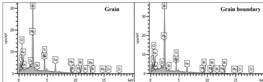
Figure 3.5 The ion beam etching surface images and EDS analysis of ceramics with different lead raw materials.
