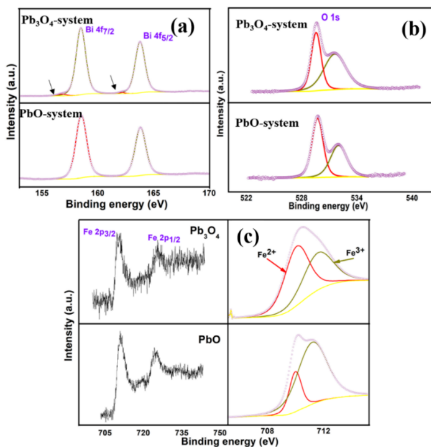
Figure 3.7 XPS analysis for Bi 4f, O 1s and Fe 2p core level binding energy spectra of ceramics with different lead raw materials.
