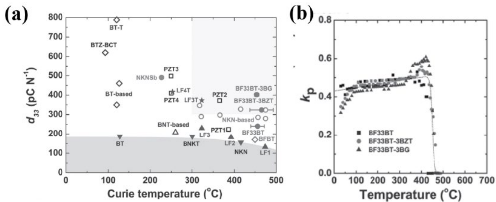
Figure 1.6 (a) The d_{33} and T_c of various piezoceramics; (b) The k_p of \text{BiFeO}_3 - \text{BaTiO}_3 based ternary ceramics versus temperature [47].
