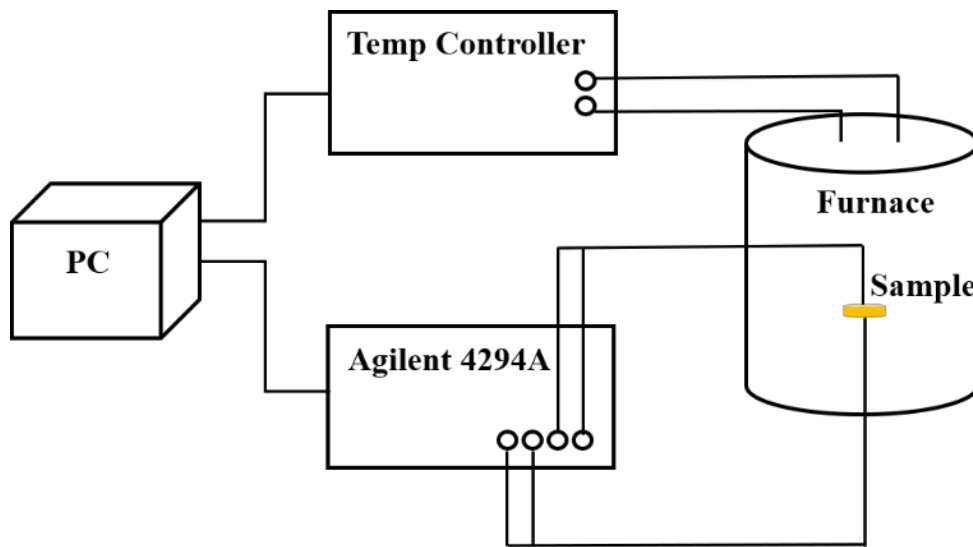
Figure 2.4 Schematic of high-temperature of dielectric spectrum.
