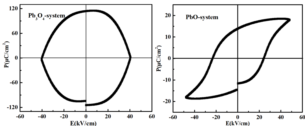
Figure 3.4 The electric field dependence of the electrical polarization for ceramics with different lead raw materials.
