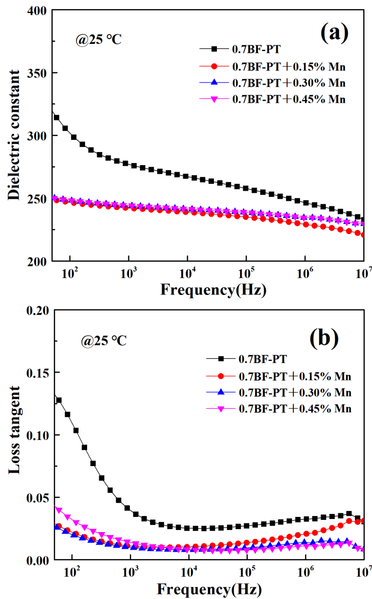
Figure 5.5 The frequency dependencies of (a) \epsilon_r ; (b) \tan\delta at room temperature for the 0.7BF-0.3PT+xwt%MnCO 3 (x=0, 0.15, 0.3, 0.45) ceramics.
