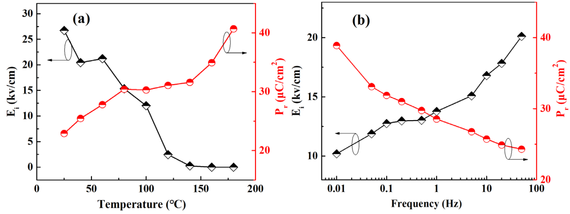
Figure 4.7 (a) The temperature dependences of E_i and P_r for the poled 0.6BF-0.24PT-0.16BST ceramics; (b) the frequency dependences of E_i and P_r for the poled 0.6BF-0.24PT-0.16BST ceramics.
