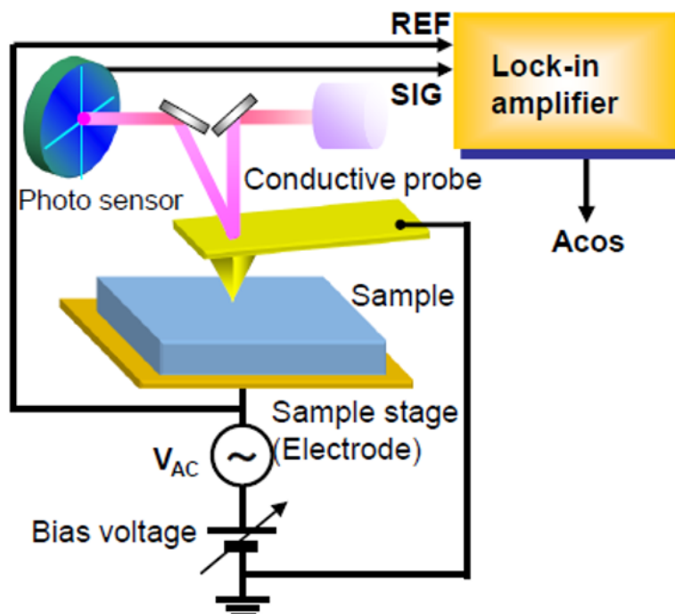
Figure 2.2 Schematic set-up of piezoelectric force microscopy (PFM).
