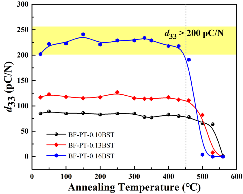
Figure 3.17 The variation of d_{33} values after thermal annealing for selected samples.
