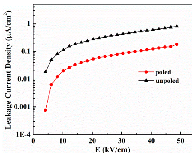
Figure 4.4 Leakage current density as a function of electric field for the poled and unpoled 0.6BF-0.24PT-0.16BST ceramics.
