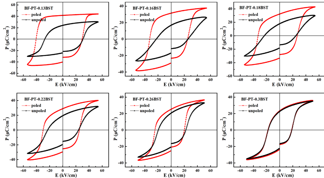
Figure 4.8 The hysteresis ( P - E ) loops of the poled and the unpoled (0.76- x )BF-0.24PT- x BST ( x=0.13, 0.16, 0.18, 0.22, 0.26, 0.3 ) ceramics
