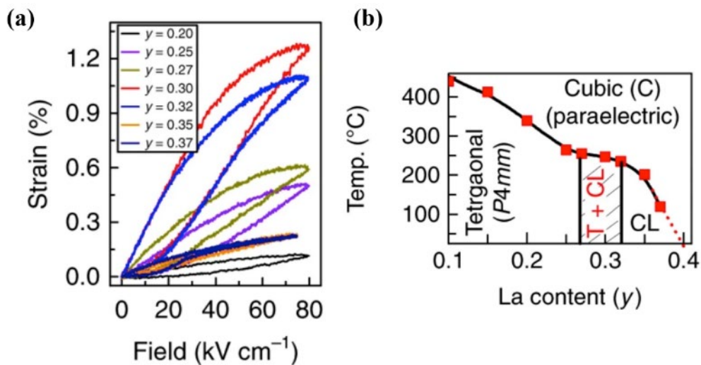
Figure 16 (a) The unipolar strain-electric-field curve of 0.55\text{Bi}_{1-y}\text{La}_y\text{FeO}_3\text{-}0.45\text{PbTiO}_3 for different La concentration; (b) The phase diagram of BLF-PT based ceramics [118].
