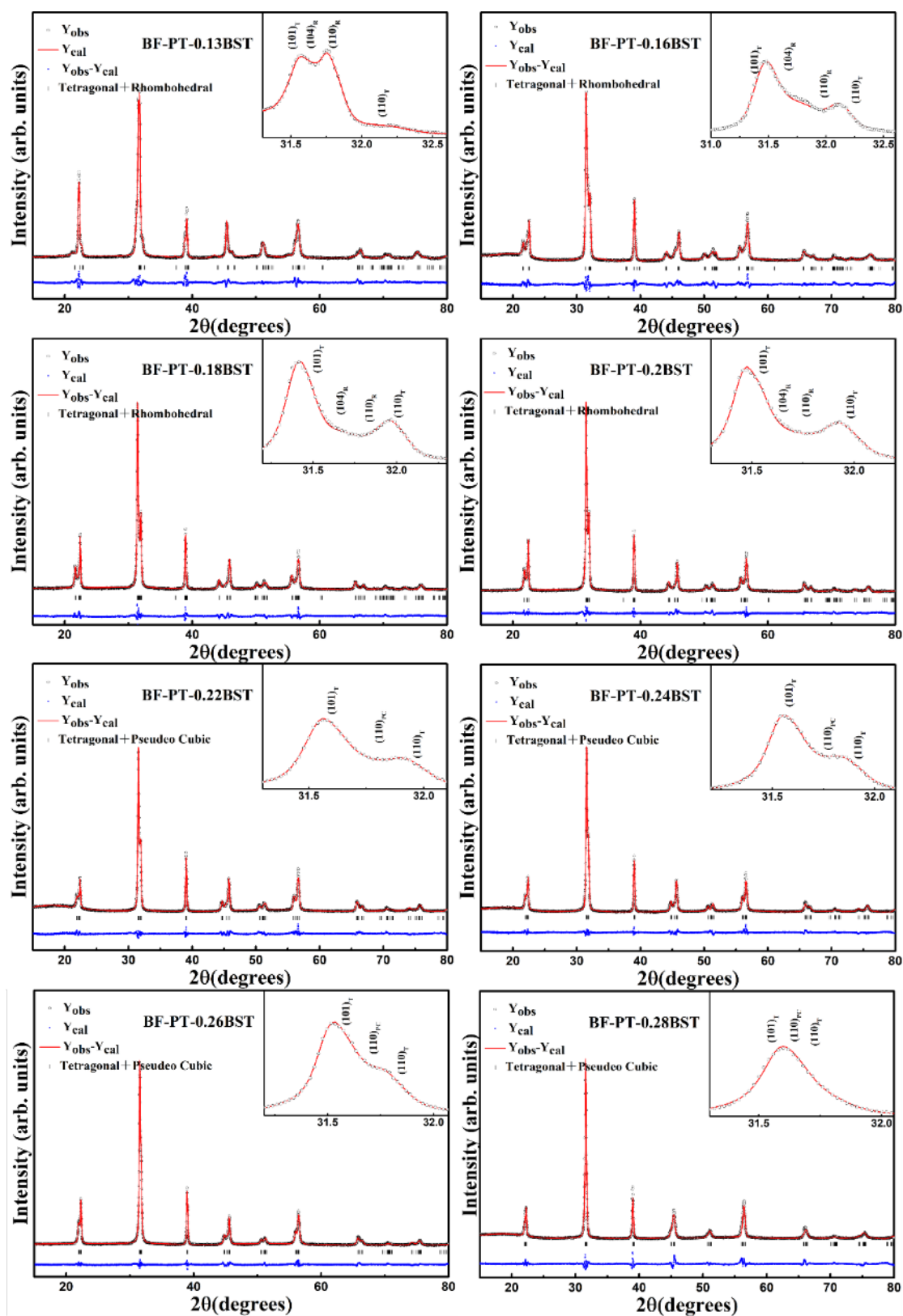
Figure 3.9 XRD patterns with Rietveld refinement of (0.76-x)\text{BF}-0.24\text{PT}-x\text{BST} ceramics
