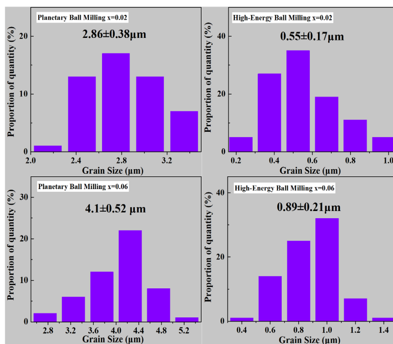
Figure 6.4 Grain size distributions of BFBT-xBMN ( x=0.02 , 0.06 ) ceramics.
