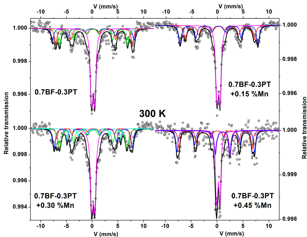
Figure 5.12 Mössbauer spectrum of 0.7\text{BF}-0.3\text{PT}+x\text{wt}\%\text{MnCO}_3 ( x=0, 0.15, 0.3, 0.45 ) ceramics.
