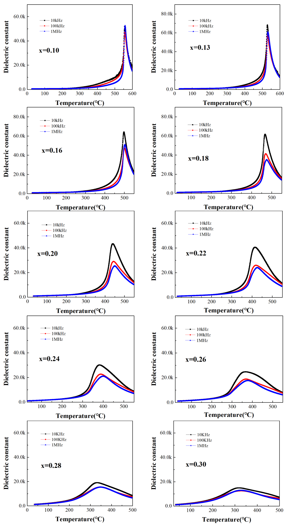
Figure 3.14 Dielectric constant \epsilon as a function of temperature with different frequency for (0.76-x)\text{BF}-0.24\text{PT}-x\text{BST} ceramics.
