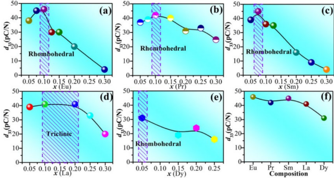
Figure 1.11 The piezoelectric coefficient d_{33} of BFO ceramics doped with different rare earth elements (Eu, Pr, Sm, La, Dy) [86].
