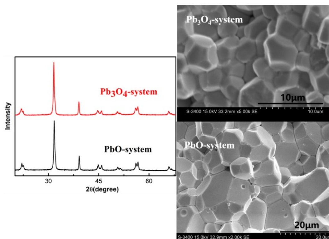
Figure 3.1 The XRD patterns and the SEM images of the ceramics with different lead raw materials.
