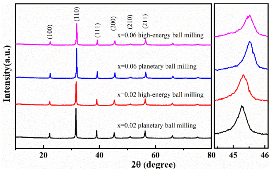
Figure 6.2 XRD patterns of BFBT-xBMN ( x=0.02, 0.06 ) ceramics.
