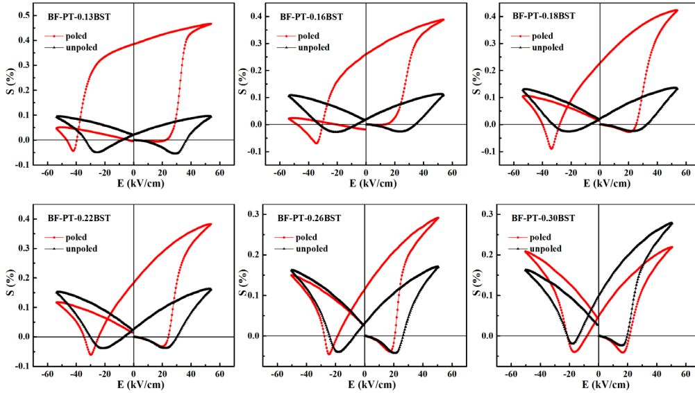
Figure 4.9 The bipolar S - E loops of the poled and the unpoled (0.76-x)\text{BF}-0.24\text{PT}-x\text{BST} ( x=0.13, 0.16, 0.18, 0.22, 0.26, 0.3 ) ceramics.
