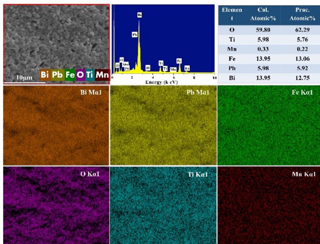
Figure 5.4 The element distribution of the sample and the surface SEM images of the 0.7BF-0.3PT+0.15wt%Mn ceramics.
