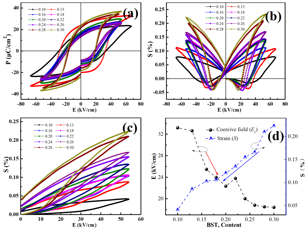
Figure 3.16 (a) Bipolar polarization hysteresis loops; (b) bipolar S - E loops; (c) unipolar S - E loops of (0.76-x)\text{BF}-0.24\text{PT}-x\text{BST} ceramics at room temperature; (d) E_c and unipolar strain values with varying BST content.
