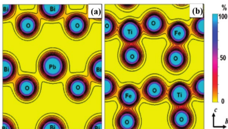
Figure 1.15 Valence electron density distributions on the bc planes of 0.67BF-0.33PT ceramics [105] .
