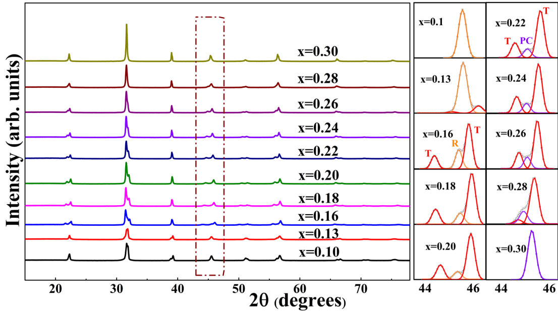
Figure 3.8 Powder XRD patterns of (0.76-x)\text{BF}-0.24\text{PT}-x\text{BST} ceramics ( x=0.10-0.30 ), and locally magnified (200) diffraction peaks.
