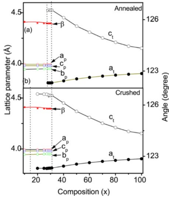
Figure 1.13 Lattice parameters of (1-x)\text{BF}-x\text{PT} binary solid solution [97].
