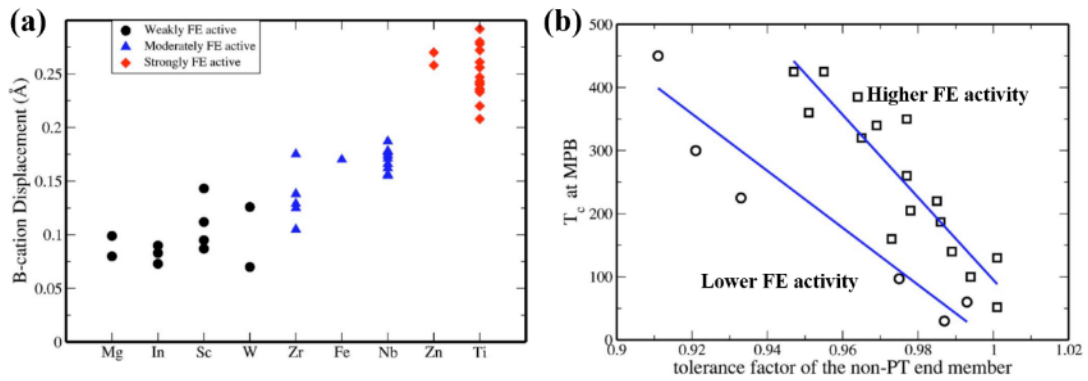
Figure 1.8 (a) Distortion for the B cation in PT solid solutions; (b) T_c of \text{Bi}(\text{Me})\text{O}_3\text{-PbTiO}_3 based ceramics at MPB vs tolerance factor of \text{Bi}(\text{Me})\text{O}_3 [73].
