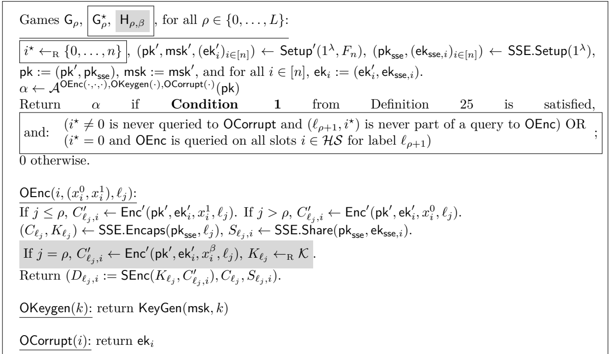
Figure 6.9: Games for the proof of Theorem 18. Here, \mathcal{HS} := [n] \setminus \mathcal{CS} , the set of honest slots, where \mathcal{CS} is the set of slots queried to \text{OCorrupt} . Recall that the algorithm \text{SSE.Encaps} is randomized, thus, different invocation of \text{SSE.Encaps}(pk_{\text{sse}}, \ell_j) on the same input will produce different outputs.
