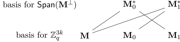
Figure 3.1: Solid lines mean orthogonal, that is: \mathbf{M}^\top \mathbf{M}_0^* = \mathbf{M}_1^\top \mathbf{M}_0^* = \mathbf{0} = \mathbf{M}^\top \mathbf{M}_1^* = \mathbf{M}_0^\top \mathbf{M}_1^* .
