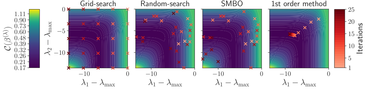
Figure 5.2 – Elastic net CV, rcv1 dataset. Level sets of a 5-fold cross-validation error \mathcal{C}(\hat{\beta}^{(\lambda)}) as a function of \lambda_1 and \lambda_2 for multiple hyperparameter optimization methods for the elastic net \arg \min_{\beta \in \mathbb{R}^p} \frac{1}{2} \|y - X\beta\|_2^2 + e^{\lambda_1} \|\beta\|_1 + e^{\lambda_2} \|\beta\|^2/2 . The crosses represent 25 first errors evaluation by each method.
