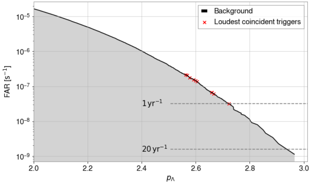
Figure 4.23: False alarm rate of the PySTAMPAS O3a search as a function of \rho_\Lambda after applying all post-processing selection criteria (DQ flags and SNRfrac). On top of the curve are placed the values for the 10 most significant triggers found in coincidence with red crosses.
