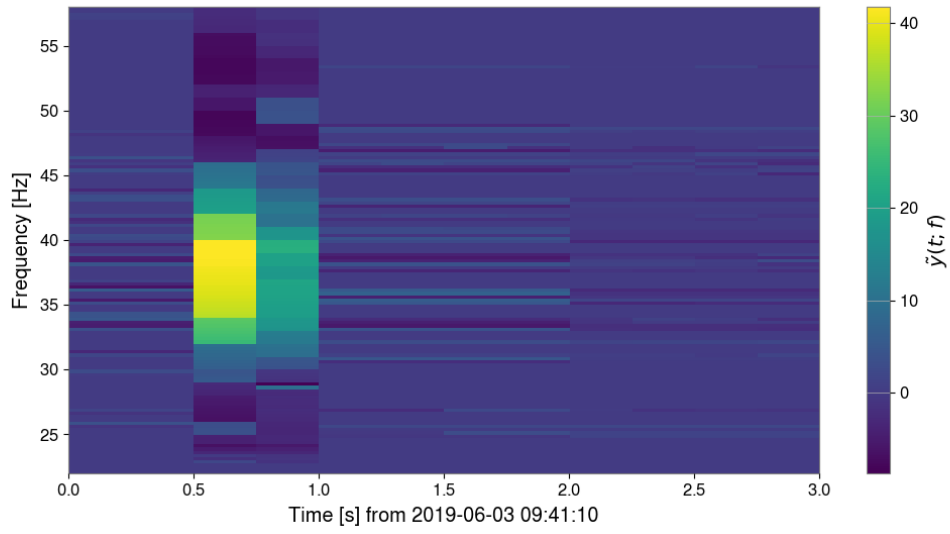
Figure 4.20: Coherent tf -map of the loudest background trigger found in the PySTAMPAS O3a analysis before the application of the SNRfrac veto.
