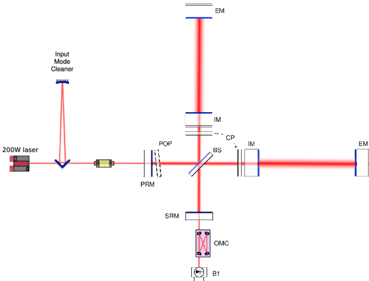
Figure 1.4: Simplified optical layout of Advanced Virgo. Input mirror (IM) and end mirror (EM) are forming the two Fabry-Perot cavities. The recycling cavities at the center of the interferometer are 12 meters long and are formed by the power recycling Mirror (PRM), the signal recycling mirror (SRM) and the two IM mirrors [31]. Compensation plates (CP) and ring heaters around optical components are in charge of controlling the thermal effects that could make cavities unstable to control.
