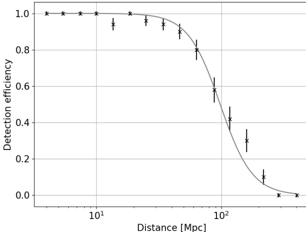
Figure 3.9: Detection efficiency as a function of distance for an accretion disk instability signal (ADI-B, see Table 3.1) added to Gaussian noise colored with LIGO O2 PSD. Error bars at 1\sigma are computed from Eq. (3.48) for N_{\text{inj}} = 50 .
