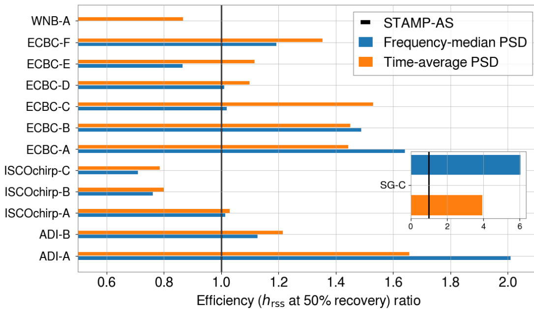
Figure 3.16: Ratio between the h_{r_{50\%}} at 50% detection efficiency obtained with PySTAMPAS and STAMP-AS for \text{FAR} = 1/50 \text{ yr}^{-1} for both PSD estimation methods over Gaussian noise. The white noise burst waveform WNB-A was not recovered at all using the frequency-median PSD.
