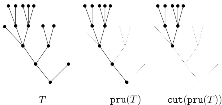
Figure 6.1: Essential structure \text{cut}_n(\text{pru}_n(T)) for n = 4, k = 5 .
