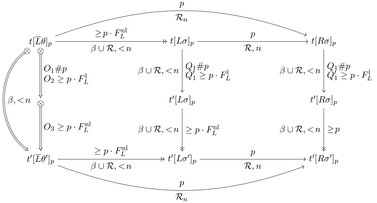
Figure 4.3: DD for the mixed peak: \xleftrightarrow[\beta; k]{\otimes} \xleftrightarrow[\mathcal{R}, n]{\otimes} with k < n . See Lemma 4.4.6.
