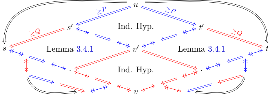
Figure 3.6: Parallel decreasing diagrams merging in Theorems 3.5.8 and 3.5.9
