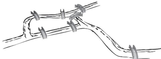
Figure 2.10: The seven bridges of Königsberg. Source: http://planund.com/
