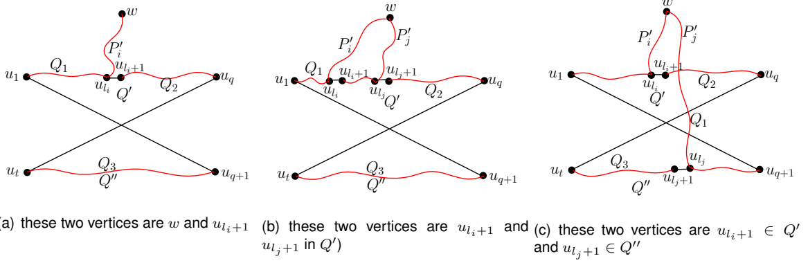
Figure 3.6: Two of four vertices w, u_{i+1}, u_{i+2}, u_{i+3} should be in the same parity X_i with i \in \{1, 2, 3\}
