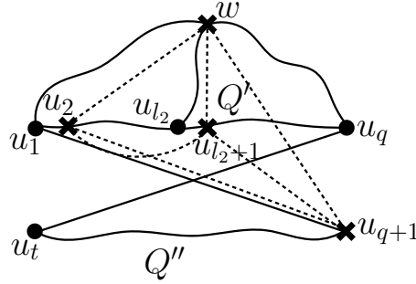
Figure 3.7: When u_{l_3} = u_q and u_{l_2} \in Q'
