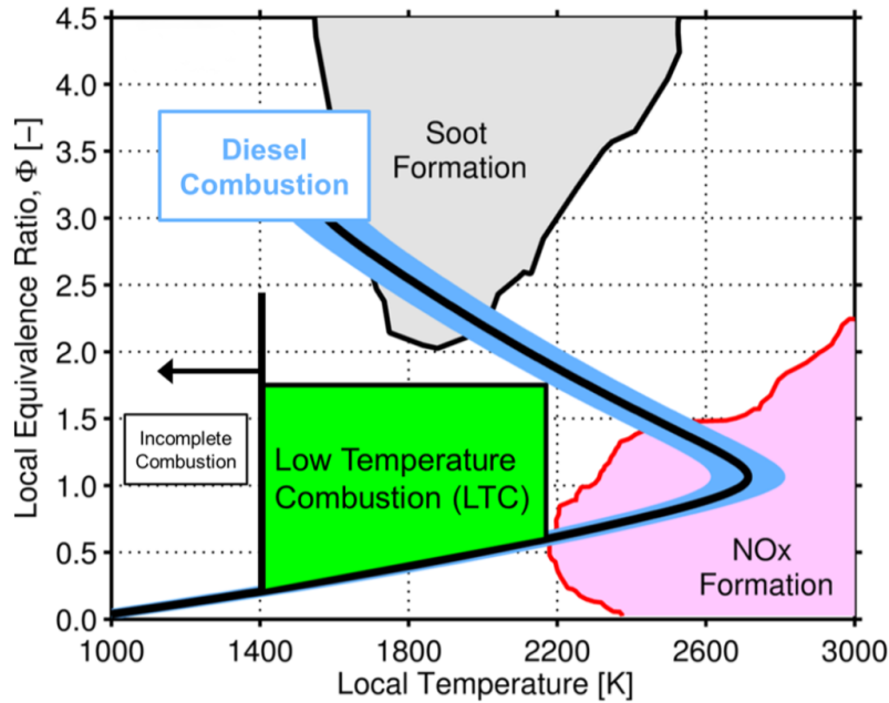
Figure 5: Soot and \text{NO}_x formation regions in a local equivalence ratio \Phi vs. local temperature T space. Extracted from Dempsey et al. (2016) .
