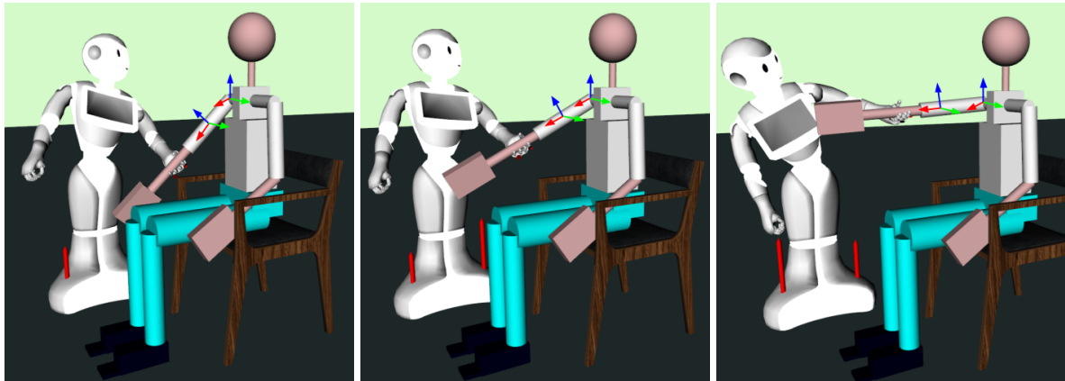
FIGURE 5.3 – MQP controller scenes of the interaction wrench and robot motion computation for assistance under pHRI constraints.
