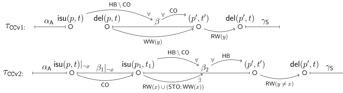
Figure 3.10: Robustness violation patterns under \text{CCv} . We use a \xrightarrow{R} \forall \beta to denote \forall b \in \beta . (a, b) \in R . We use \beta_1|_{\neg x} to say that all delayed transactions in \beta_1 do not access x . For violation \tau_{\text{CCv1}} , t is the only delayed transaction. For \tau_{\text{CCv2}} , all delayed transactions are in \text{isu}(p, t) \cdot \beta_1 \cdot \text{isu}(p_1, t_1) and they form a causality chain that starts at \text{isu}(p, t) and ends at \text{isu}(p_1, t_1) .
