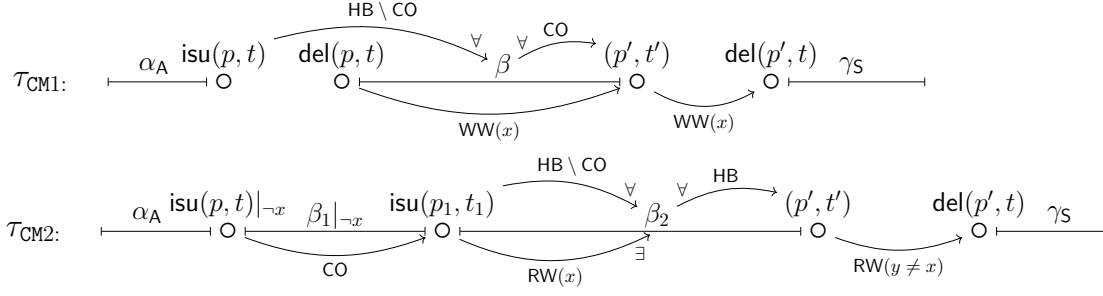
Figure 3.12: Robustness violation patterns under \text{CM} . For violation \tau_{\text{CM1}} , t is the only delayed transaction. For \tau_{\text{CM2}} , all delayed transactions are in \text{isu}(p, t) \cdot \beta_1 \cdot \text{isu}(p_1, t_1) and they form a causality chain that starts at \text{isu}(p, t) and ends at \text{isu}(p_1, t_1) .
