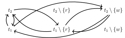
Figure 4.2: Commutativity dependency graph of WS where the read of y is omitted.
