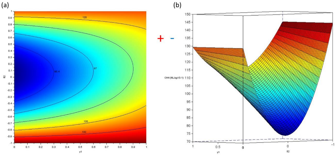
Figure 34 : (a, b) : Predicted methane yield for Run 2, according to the recirculation frequency and the damp grass composition
