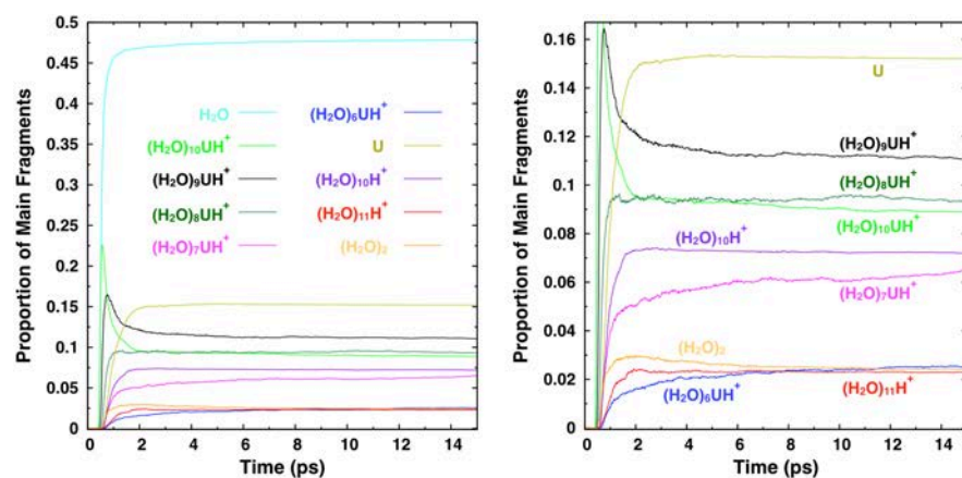
Figure 4.9: Time-dependent proportions of the main fragments obtained from the dissociation of the lowest-energy isomer of (H_2O)_{11}UH^+ . Right panel corresponds to a zoom over the lower proportions.
