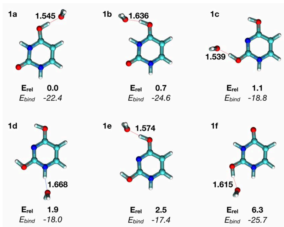
Figure 3.19: Lowest-energy structures of (\text{H}_2\text{O})\text{UH}^+ obtained at the MP2/Def2TZVP level of theory. Relative ( E_{rel} ) and binding energies ( E_{bind} ) are given in kcal.mol -1 . Important hydrogen-bond distances are indicated in bold and are given in Å.
