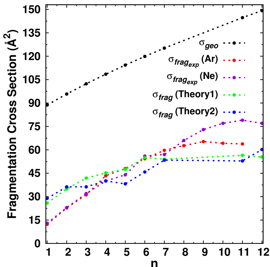
Figure 4.17: Theoretical (green and blue lines) and experimental (red line) \sigma_{frag} values for the (H_2O)_{1-7,11,12}UH^+ clusters. Theory 1 (green line) is obtained from the isomers which P_{NUL} matches best to the experimental data while Theory 2 (blue line) is obtained from lowest-energy isomers.
