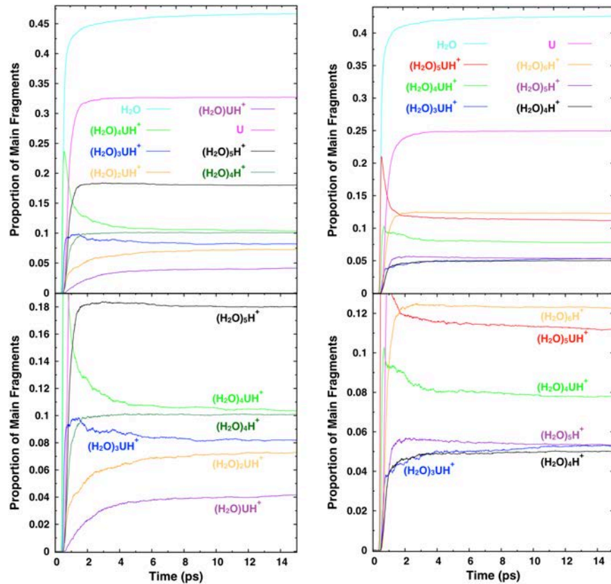
Figure 4.8: Time-dependent proportions of the main fragments obtained from the dissociation of the lowest-energy isomers of (H_2O)_5UH^+ (left) and (H_2O)_6UH^+ (right). Bottom panels correspond to a zoom over the lower proportions.
