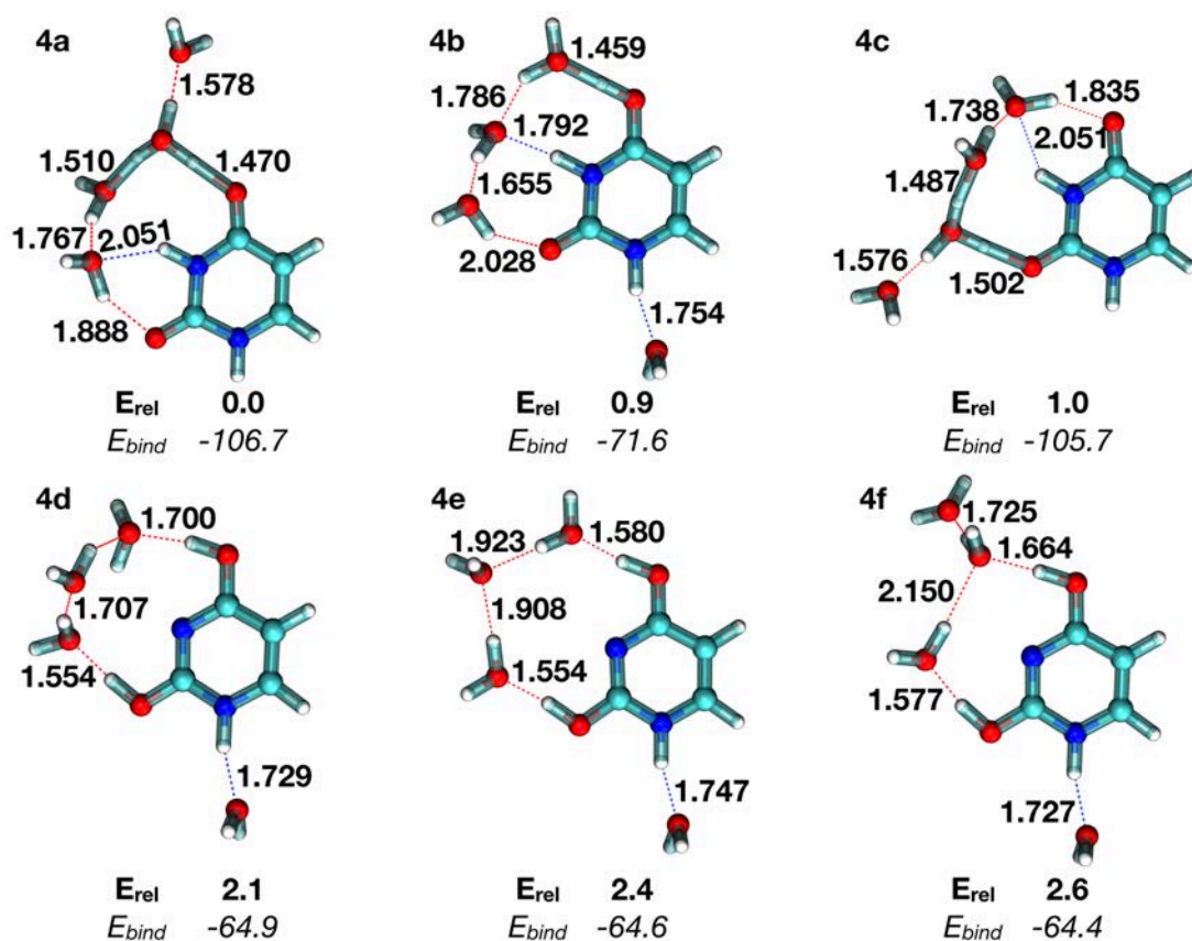
Figure 3.23: Lowest-energy structures of (\text{H}_2\text{O})_4\text{UH}^+ obtained at the MP2/Def2TZVP level of theory. Relative ( E_{\text{rel}} ) and binding energies ( E_{\text{bind}} ) are given in kcal.mol ^{-1} . Important hydrogen-bond distances are indicated in bold and are given in Å.
