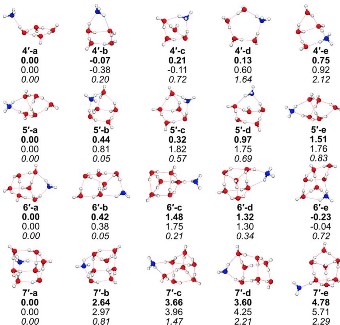
Figure 3.10: The five low-energy isomers of cluster (\text{H}_2\text{O})_4\text{-}_7\text{NH}_3 and the associated relative energies (in kcal·mol -1 ) at MP2/Def2TZVP level with (bold) and without ZPVE correction and SCC-DFTB level (italic).
