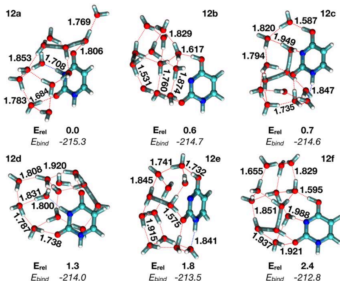
Figure 3.28: Lowest-energy structures of (\text{H}_2\text{O})_{12}\text{UH}^+ obtained at the MP2/Def2TZVP level of theory. Relative ( E_{\text{rel}} ) and binding energies ( E_{\text{bind}} ) are given in kcal.mol ^{-1} . Important hydrogen-bond distances are indicated in bold and are given in Å.
