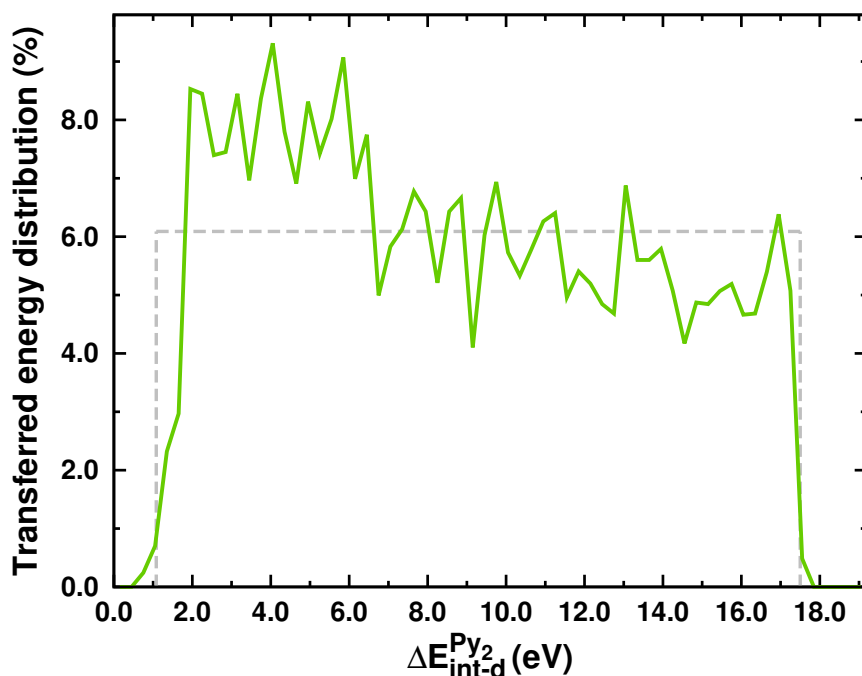
Figure 4.26: Distribution of transferred energy in rovibrational modes \Delta E_{int-d}^{Py_2} for trajectories leading to dissociation at the end of MD (center of mass collision energy of 17.5 eV). The dashed line shows the distribution of transferred energy used in the LOC model.
