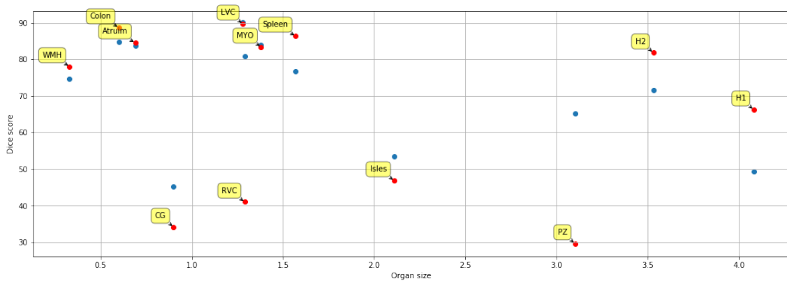
Figure 5.4 – Influence on the organ size on the average Dice score. Each dot represents a dataset. Blue (resp. red) dots show the Dice score obtained with the Dice loss (resp. the Size loss).
