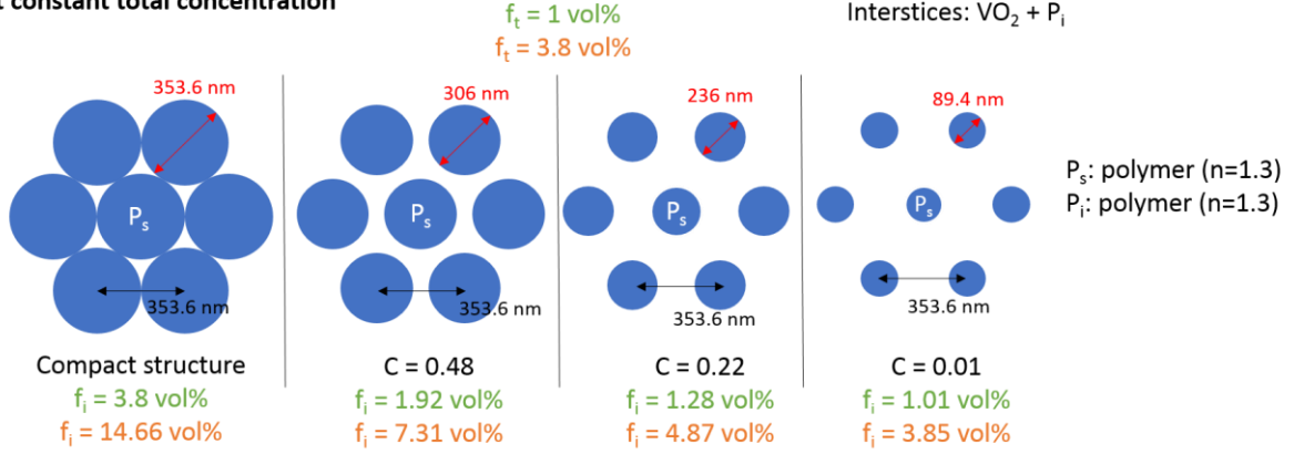
Figure 80: Top views of a (111) plane of the simulated opals at various structure compactities C with constant total \text{VO}_2 concentrations f_t = 1 \text{ vol\%} and f_t = 3.8 \text{ vol\%} .
