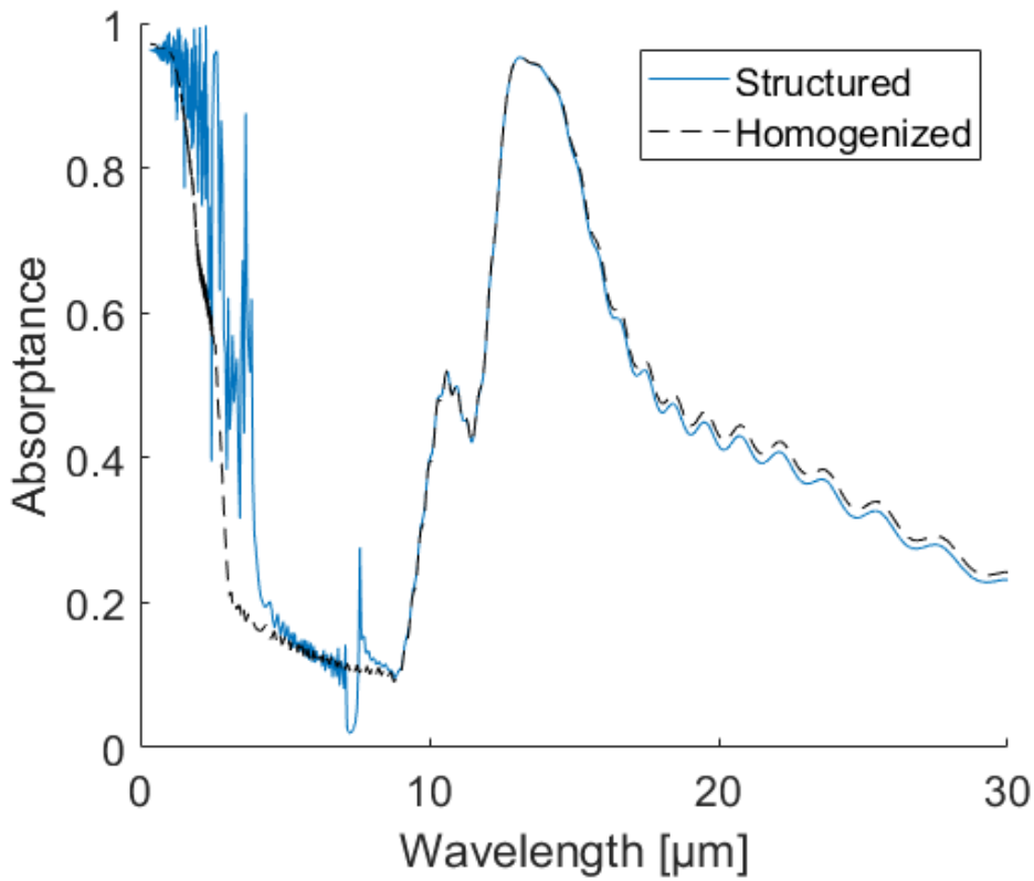
Figure 109: Absorptance spectra of a polymer compact opal photonic crystal consisting of polymer spheres ( n=1.3 ) surrounded by a mixture of \text{VO}_2 and another polymer ( n=1.7 ) (solid lines), and its homogenized counterpart (dashed lines), with a cell parameter a=4.5 \mu\text{m} , at normal incidence, in cold conditions. The \text{VO}_2 total concentration is 1 vol%.
