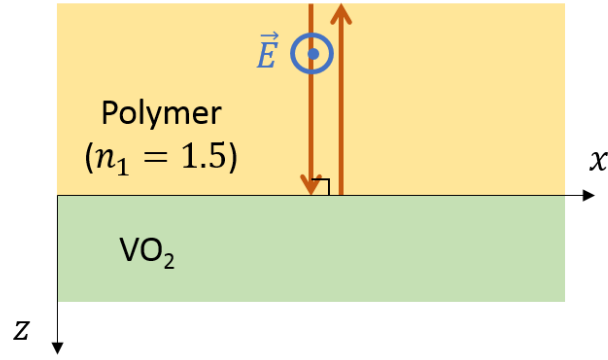
Figure 38: Illustration of a polymer-VO 2 interface with normally incident light.
