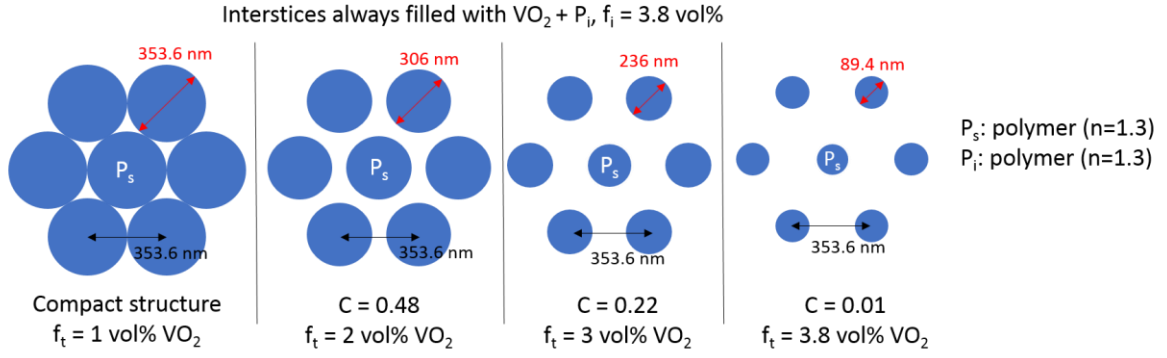
Figure 75: Top views of a (111) plane of the simulated opals at various structure compactities C with a constant \text{VO}_2 concentration in the opal interstices f_i .
