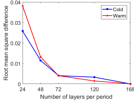
Figure 95: Root mean square difference compared to our finest model (168 layers/period), as a function of the model spatial resolution along the axis normal to the surface ([111] direction), for both cold and warm conditions.
