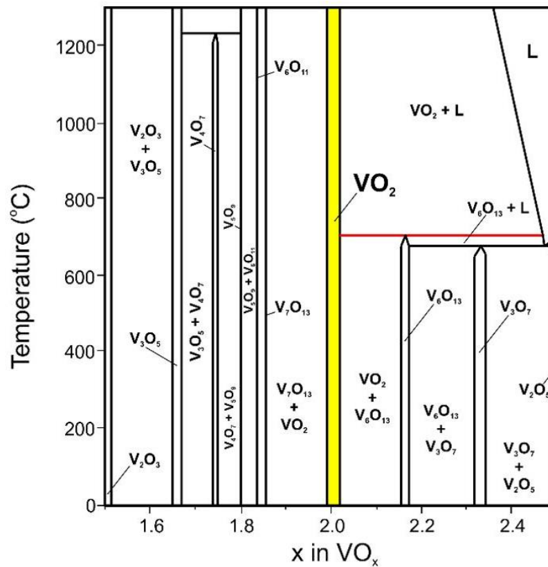
Figure 17: \text{V}_2\text{O}_3 - \text{V}_2\text{O}_5 phase diagram [21]
