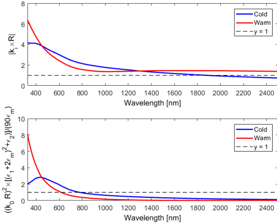
Figure 56: Left terms of the criteria given by Rupp (Equations (2. 10) and (2. 11)), for VO 2 spherical nanoparticles, with a 100 nm radius, surrounded by a polymer matrix ( n = 1.5 ) in cold (blue) and warm (red) conditions. For a valid Maxwell-Garnett homogenization, these values should be small compared to 1 (dashed lines).
