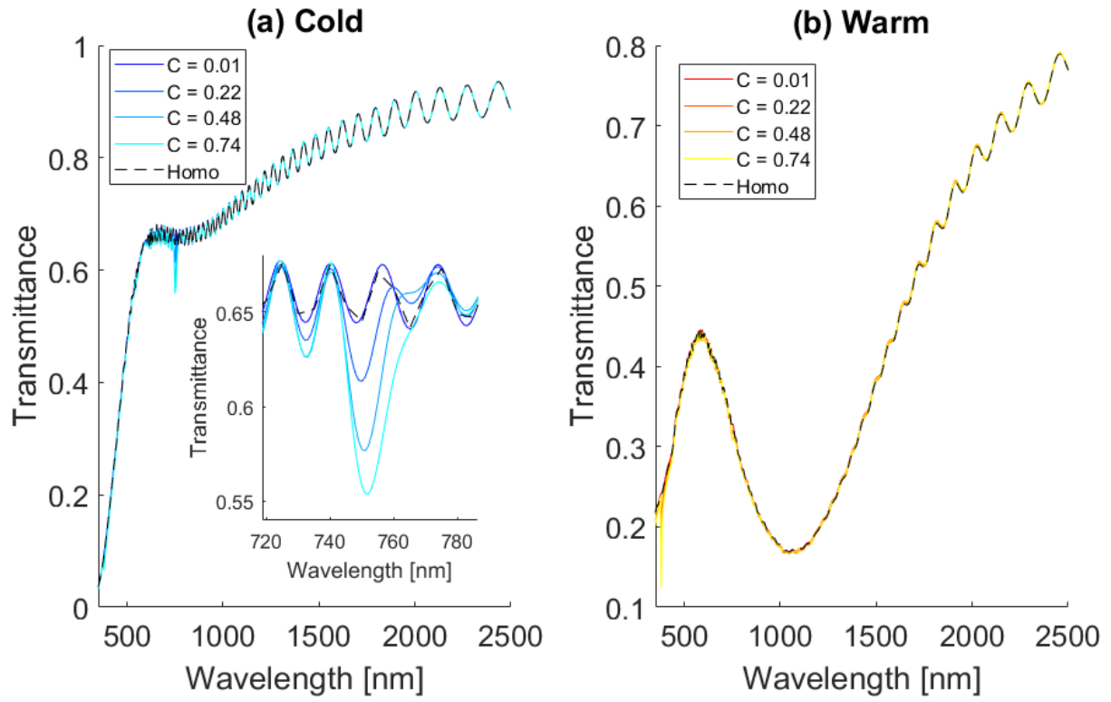
Figure 81: Transmittance spectra for normally incident light of an opal made of polymer ( n=1.3 ) spheres and a mixture of VO 2 nanoparticles dispersed in the same polymer, for different structure compacities C and both VO 2 cold (a) and warm (b) phases, considering a structured material (solid lines) and a homogenized one (dashed lines). The total VO 2 concentration is set to ft = 1 vol%. The inset in the left figure is a zoom around the PBG position for the cold VO 2 phase.
