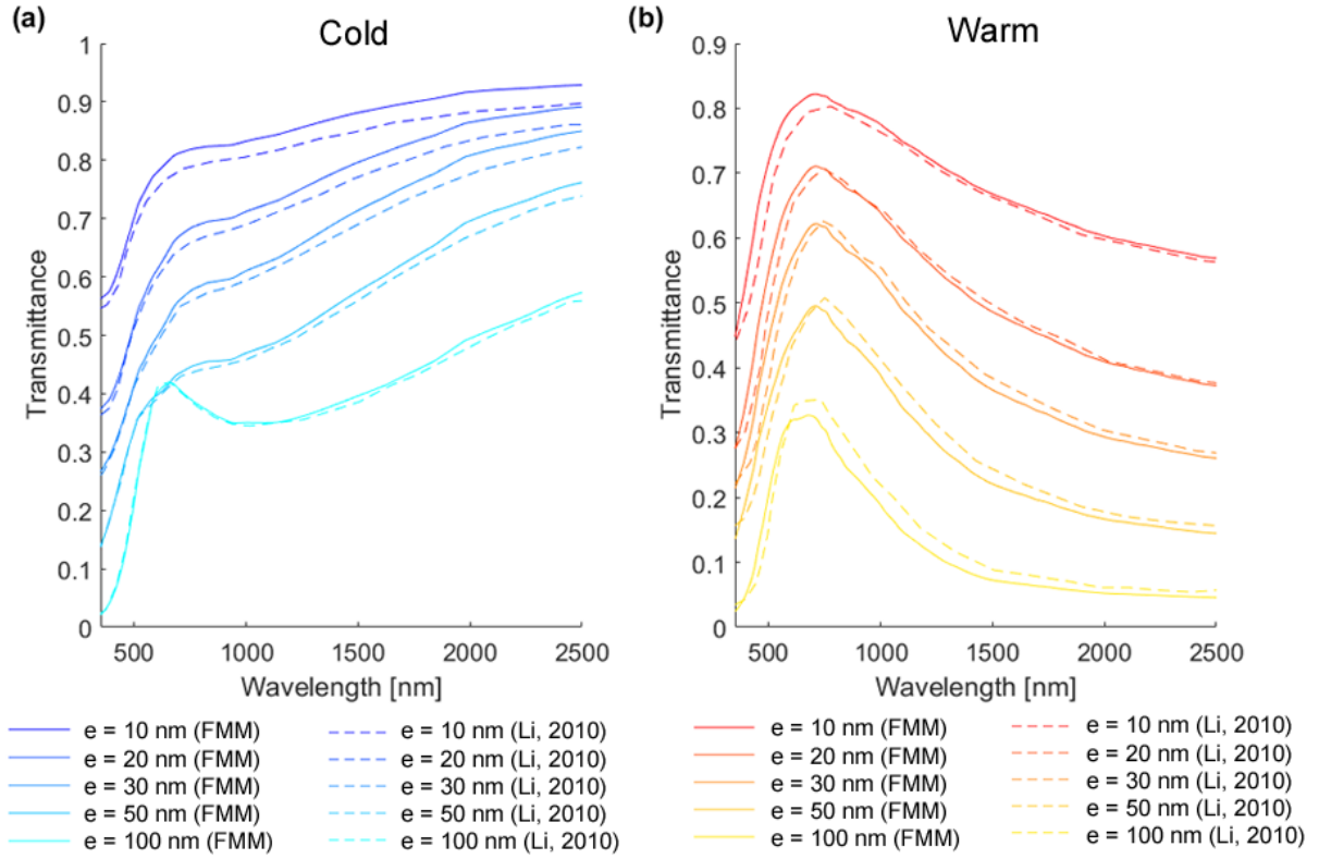
Figure 41: Computed spectral transmittances of a pure dense \text{VO}_2 film on a glass substrate ( n=1.5 ), for different thicknesses (10, 20, 30, 50 and 100 nm), in cold (a) and warm (b) conditions (solid lines). Results are compared with [36] (dashed lines).
