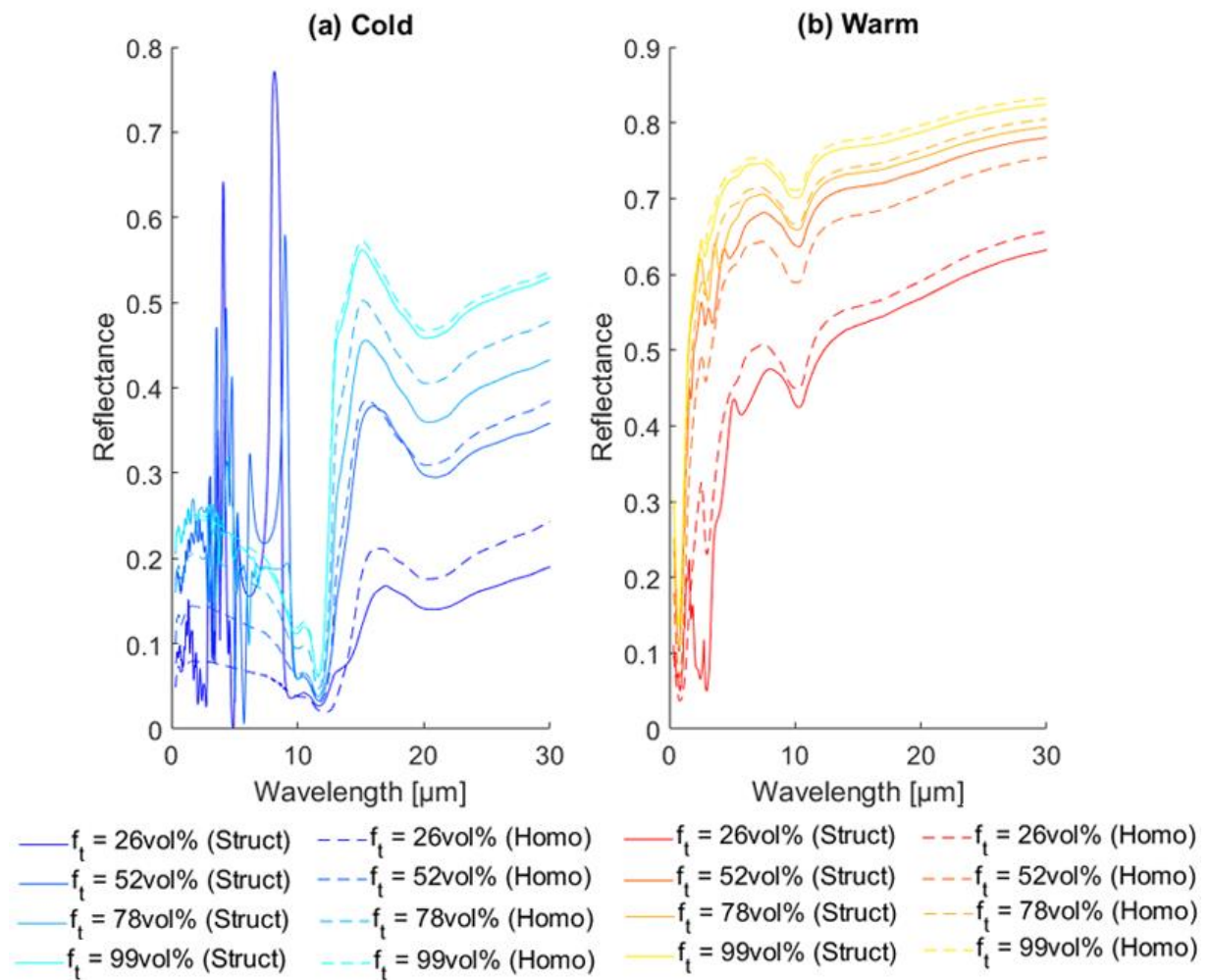
Figure 102: Reflectance spectra of a polymer opal photonic crystal consisting of polymer spheres ( n=1.3 ) surrounded by VO 2 with a cell parameter a=4.5 \mu\text{m} (solid lines) and of the corresponding homogenized material (dashed lines), at normal incidence, in both cold (left) and warm (right) conditions, as a function of the total VO 2 concentration f_t .
