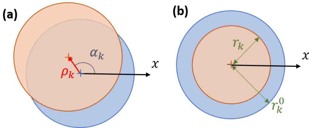
Figure 127: Schematic representation of a cylinder before (blue) and after (orange) applying a center position shifting defined by a distance \rho_k and an angle \alpha_k relative to the x-axis (a), and a radius variation from r_k^0 to r_k (b).
