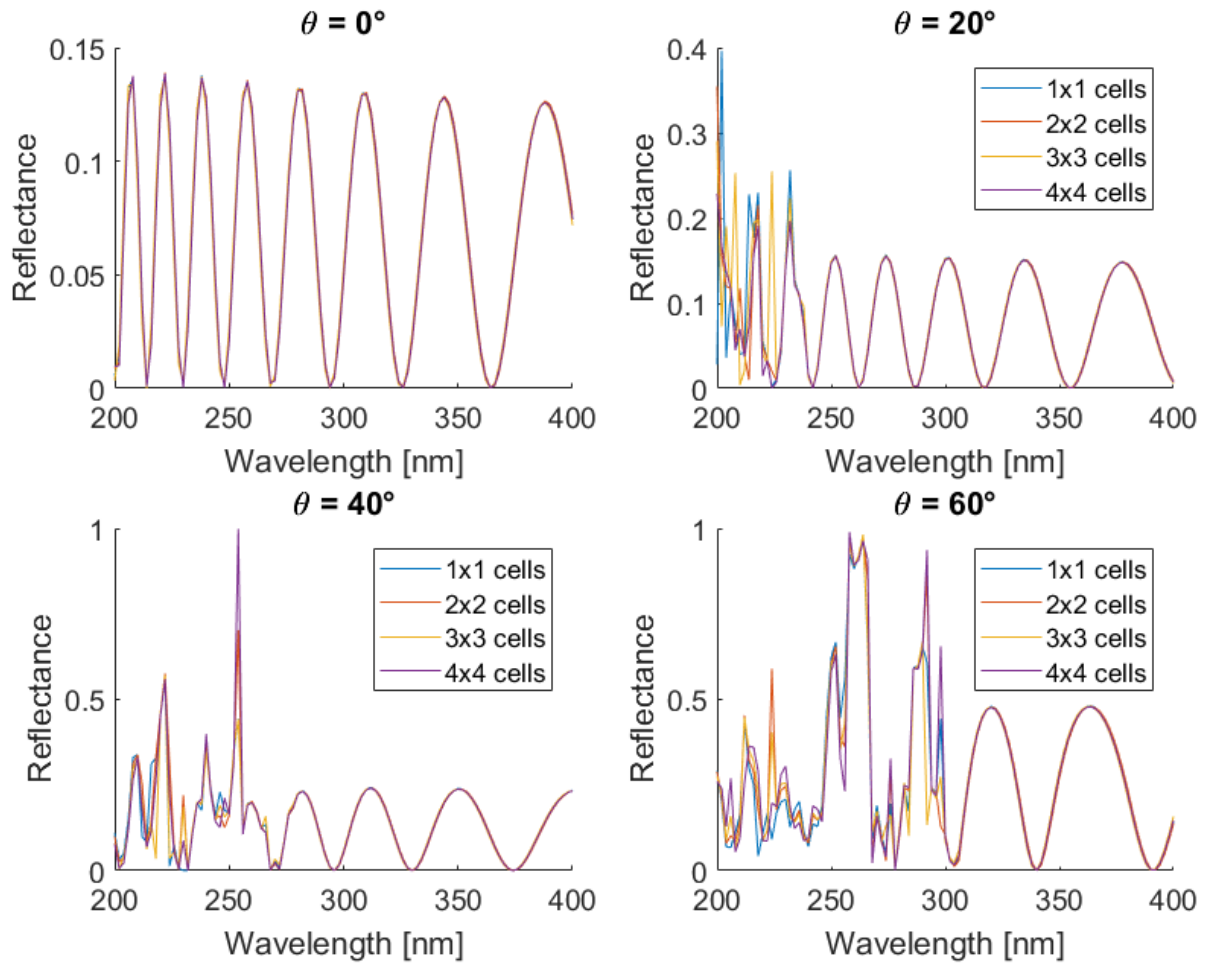
Figure 132: Reflectance spectra of a perfectly ordered porous alumina triangular photonic crystal (thickness e = 1 \mu\text{m} ) for different incidence angles \theta ( 0^\circ , 20^\circ , 40^\circ and 60^\circ ), for TE polarized incident light, in the case of a 2-cylinder primitive cell (blue curves, denoted as 1x1 cell) and for 2x2, 3x3 and 4x4 primitive supercells. The numbers of modes are respectively (15-7), (15-7), (20-15) and (25-15) for the 2-cylinder primitive cell, the 2x2, 3x3 and 4x4 supercells.
