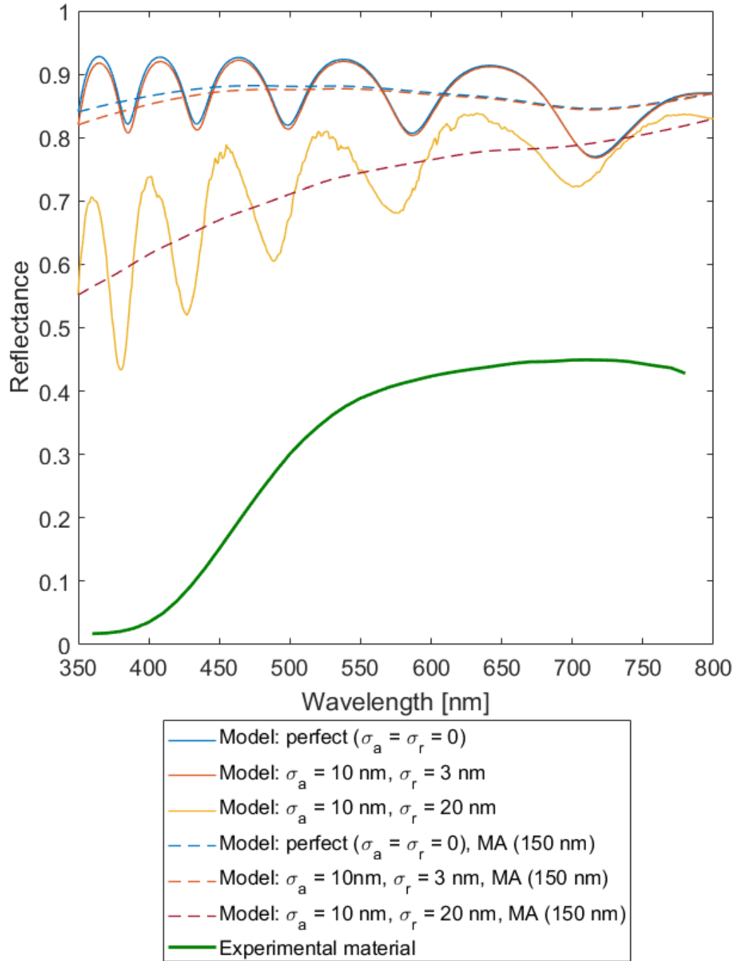
Figure 151: Reflectance spectra of the perfectly ordered (blue) and deformed (orange, yellow) alumina 2D photonic crystal modelled by a 3x3 supercell primitive cell, their averaged spectra (moving average filter with a 150 nm window) (dashed lines) and the measured total reflectance of the real material (green). The incident light is unpolarized and incident with an 8^\circ angle on the material surface. The model material thickness is 1 \mu\text{m} . All calculated spectra are averaged over the \phi angles.
