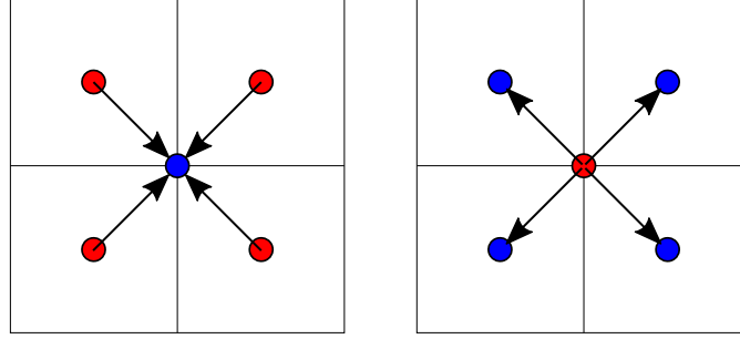
Figure 2.4: Expansion translation from children to parent (left), from parent to children (right).
