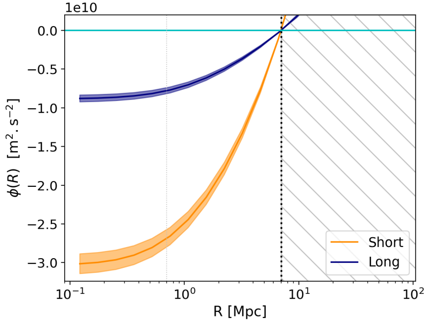
Figure 4.19: Gravitational potential (Eq. 4.17) felt by a test mass inside short (orange) and long filaments (blue). The limit between inside and outside for the computation of the gravitational potential is set to R_{\text{lim}} = r_{\text{ext}} = 7 Mpc. The outside regions are hatched in gray.
