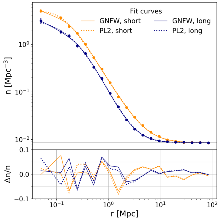
Figure 4.13: Top: Fit-curves of short (orange) and long (blue) filaments. Solid and dashed lines correspond respectively to the GFW (Eq. 4.3) and the double power law (Eq. 4.6) models. The fit curves are plotted using the parameters of Tables 4.2 and 4.3. Bottom: Relative difference of the fits with respect to the data, defined as: \Delta n/n(r) = [n^{\text{data}}(r) - n^{\text{model}}(r)]/n^{\text{data}}(r) . This figure is extracted from Galárraga-Espinosa et al. (2020).
