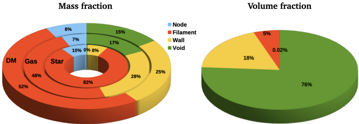
Figure 1.2: Volume and mass fractions of the nodes, filaments, walls and voids of the cosmic web (identified by the NEXUS code of Cautun et al. 2013 in the EAGLE simulation, Schaye et al. 2015). These results are reproduced from Ganeshaiah Veena et al. (2019).
