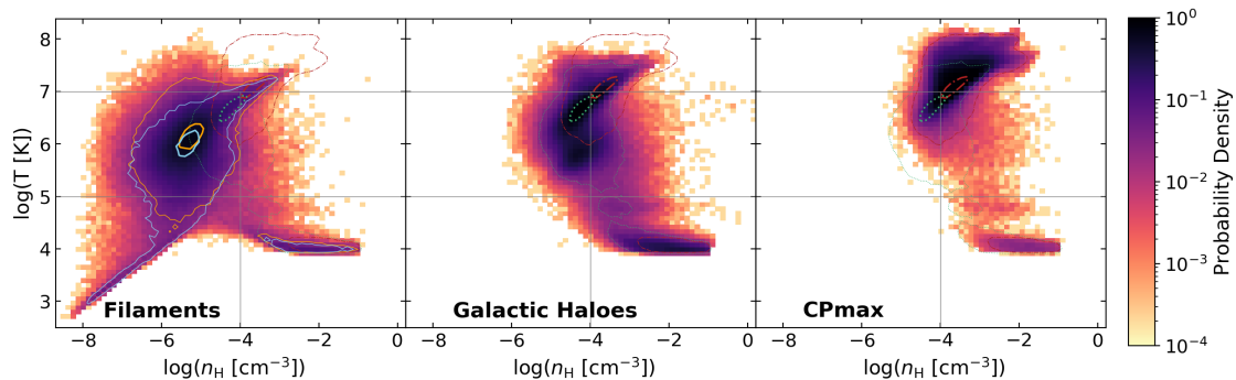
Figure 5.7: Phase portraits of gas, presenting the normalised 2D histograms of the gas cells in the corresponding structures. First panel: gas in filaments (within 1 Mpc from the core). Second panel: gas within the R_{200} radius of galactic haloes (defined as haloes of mass M_{\text{tot}} > 10^{12} M_{\odot} hosting at least one galaxy of mass 10^9 \leq M_{*}[M_{\odot}] \leq 10^{12} ). Third panel: gas within the R_{200} radius of the DisPerSE maximum density critical points (CPmax), tracers of nodes. The 68% and 99% contours correspond to results of short (orange) and long filaments (blue), to galactic haloes (dotted green lines), and CPmax (dashed-dotted red contours).
