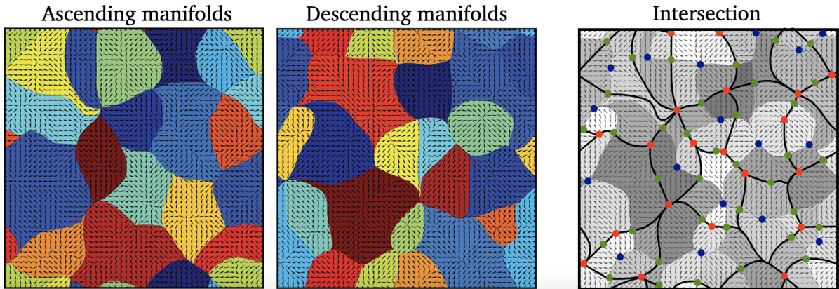
Figure 2.5: Left: Ascending and descending manifolds of the density field of Fig.2.4, reproduced from Sousbie (2011). Right: Intersection between the ascending and descending manifolds presented in the left panels. The intersection lines that connect CPmax (red) to saddles (green) correspond to the filaments (black lines). The minima of the density field are marked by the blue points.
