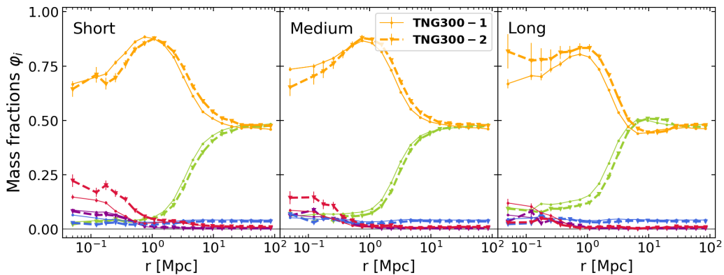
(b) Comparison with lower resolution simulation, TNG300-2
