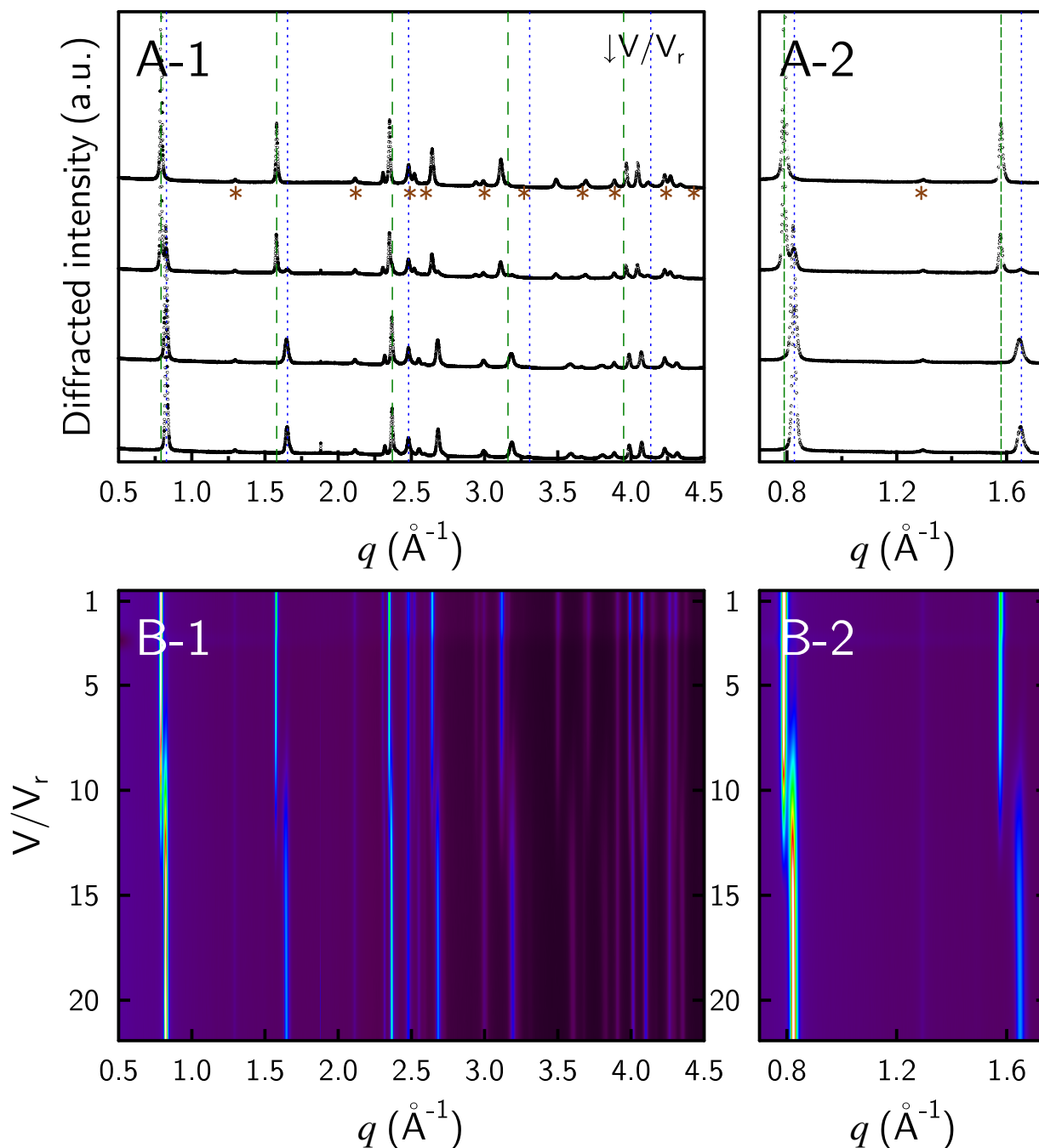
Figure V.14 – XRD patterns recorded in situ during experiment " \text{Na}_2\text{CO}_3 -XRD" with micro-Co-GR(Cl) sample (Input solution concentration: 40 \text{ mmol}\cdot\text{L}^{-1} NaCl and 10 \text{ mmol}\cdot\text{L}^{-1} \text{Na}_2\text{CO}_3 , pH = 10.9). Caption is the same as Figure V.4, except for the following details. (A) Patterns recorded after 0.5, 7.3, 14.6 and 21.4 pore volumes ( V/V_r ).
