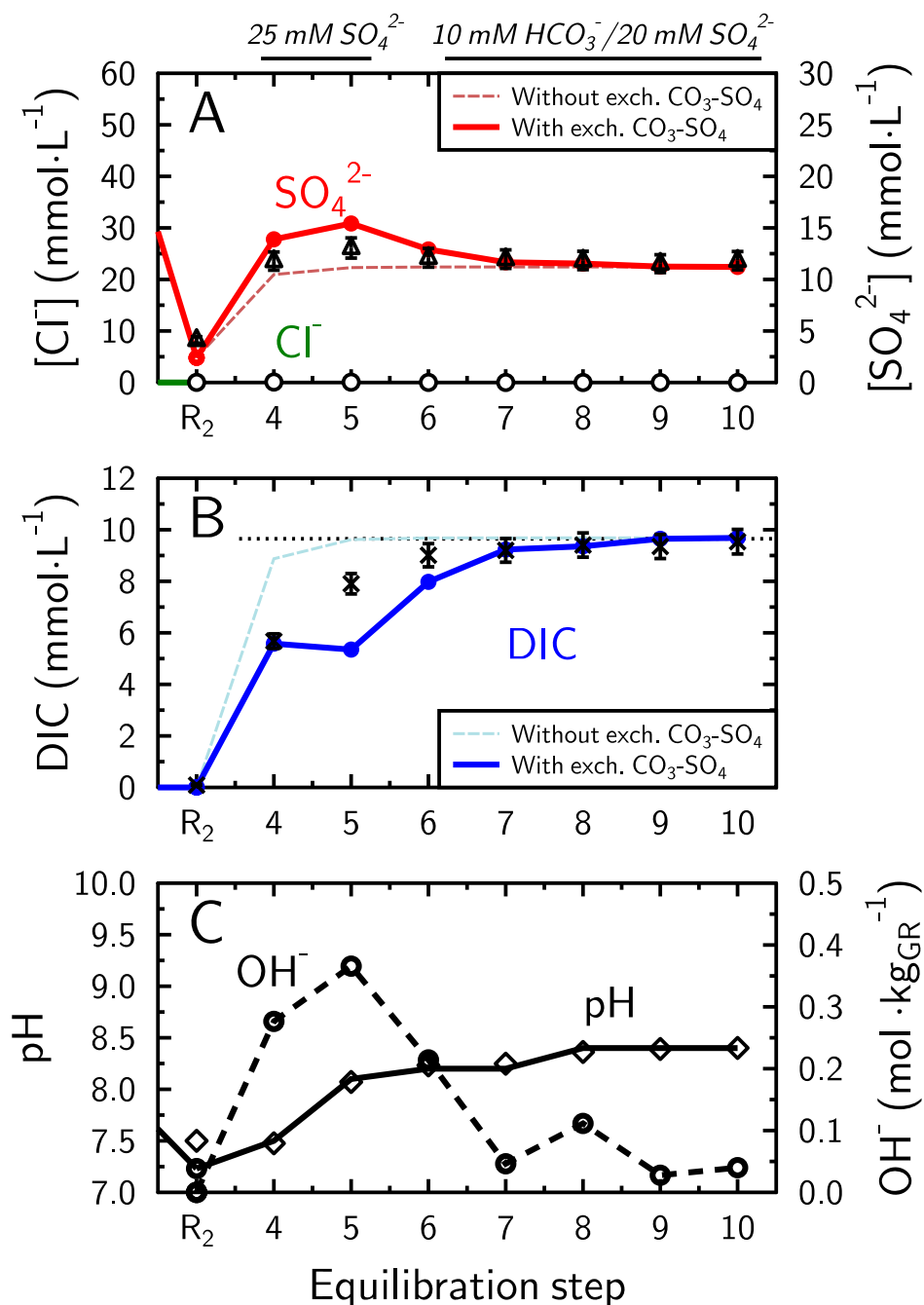
Figure V.46 – \text{CO}_3^{2-} , \text{SO}_4^{2-} & \text{Cl}^- exchange data and model on micro-Co-GR sample with one selectivity coefficient and fixing the pH. Steps R_2 corresponds to the rinsing of the sample with ultrapure water. Steps 4-10 correspond to equilibration with \text{NaHCO}_3 - \text{Na}_2\text{SO}_4 solutions with a concentration of 10 \text{ mmol} \cdot \text{L}^{-1} of \text{NaHCO}_3 and 20 \text{ mmol} \cdot \text{L}^{-1} of \text{Na}_2\text{SO}_4 (HC10/S20). (A) \text{Cl}^- and \text{SO}_4^{2-} concentrations obtained by the model compared to data ( \text{Cl}^- - black circles; \text{SO}_4^{2-} - black triangles). Colored lines are the results of the model if equation V.3 was added to the model with a Gaines & Thomas exchange model and a \log_{10} K_{ex,GT}^{\text{SO}_4-\text{CO}_3} = 2.5 (full red lines). The colored dashed line is the modelled results without equation V.3. (B) Concentrations of carbonate species obtained by the model compared to data ( \text{CO}_3^{2-} - black crosses). Colored lines are the results of the model with the same cases as figure A ( \log_{10} K_{ex,GT}^{\text{SO}_4-\text{CO}_3} = 2.5 full blue lines). The colored dashed line is the modelled results without equation V.3. The black dashed lines represent the total DIC input concentration. (C) pH (diamond - data ; full line - model) and quantity of \text{OH}^- released by micro-Co-GR phase to buffer the pH (dashed black line). pH was partially fixed in the model from step 4 to step 10.
