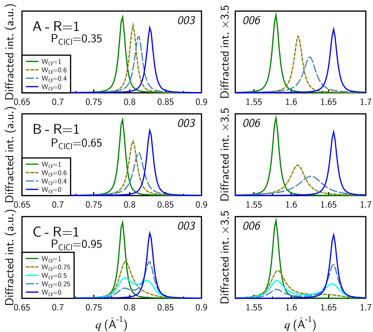
Figure V.10 – Influence of various types of interstratification on 00 l reflections of micro-Co-GR phase XRD patterns for R = 1. The caption is the same as Figure V.9. Probabilities are P_{C/CI} = 0.35 (A), P_{C/CI} = 0.65 (B) and P_{C/CI} = 0.95 (C).
