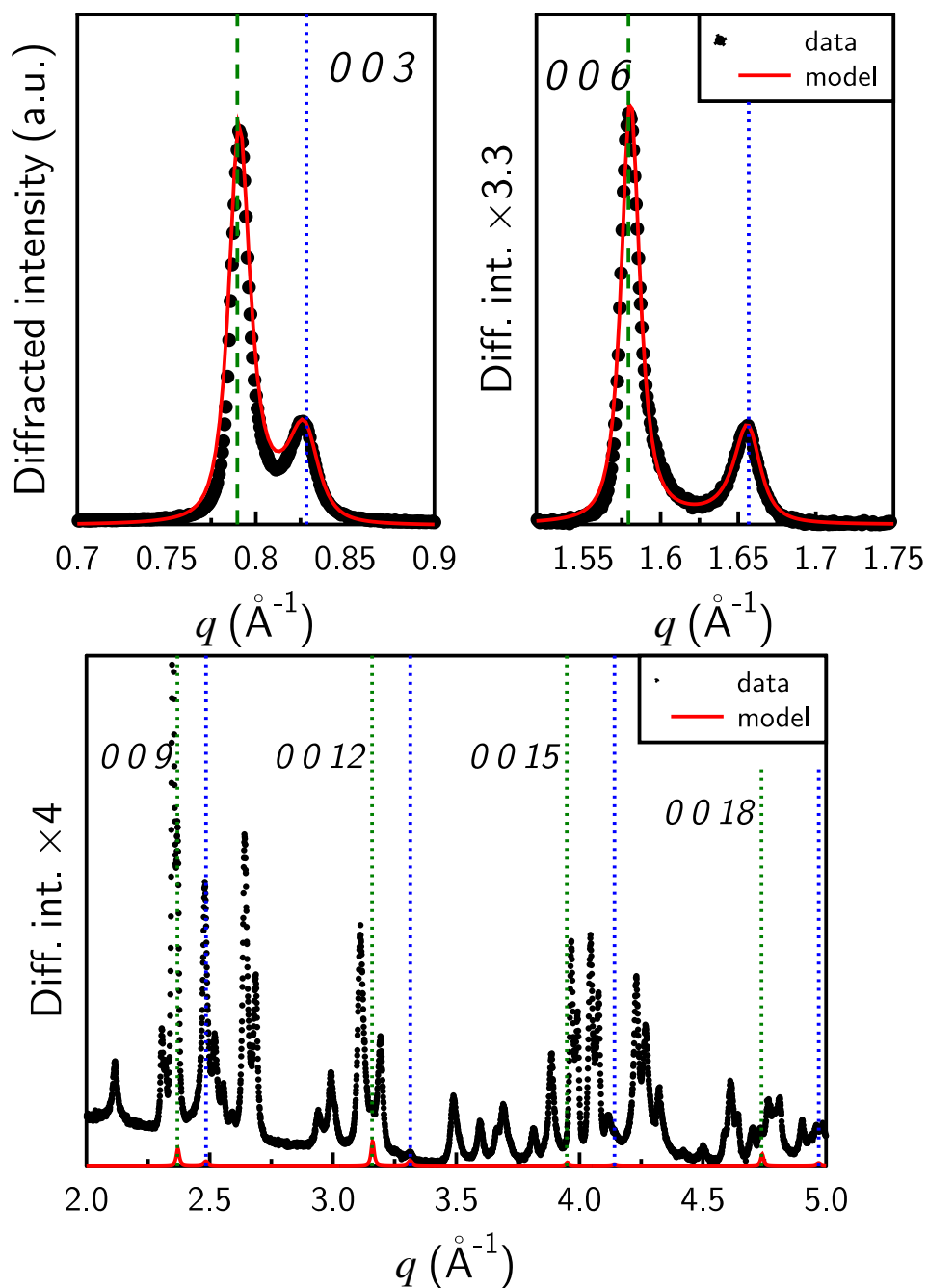
Figure S4 – Interstratification processes on micro-Co-GR sample during an exchange with C(IV) species at V/V_r = 6.0 (Solution concentration: 10 \text{ mmol} \cdot \text{L}^{-1} NaCl and 40 \text{ mmol} \cdot \text{L}^{-1} \text{NaHCO}_3 ). Green dashed line was the initial position of the 00l reflections of micro-Co-GR(Cl) phase (for V/V_r = 0 ). Blue dashed line was the initial position of the 00l reflections of micro-Co-GR(C(IV)) phase (for V/V_r = 20.4 ).
