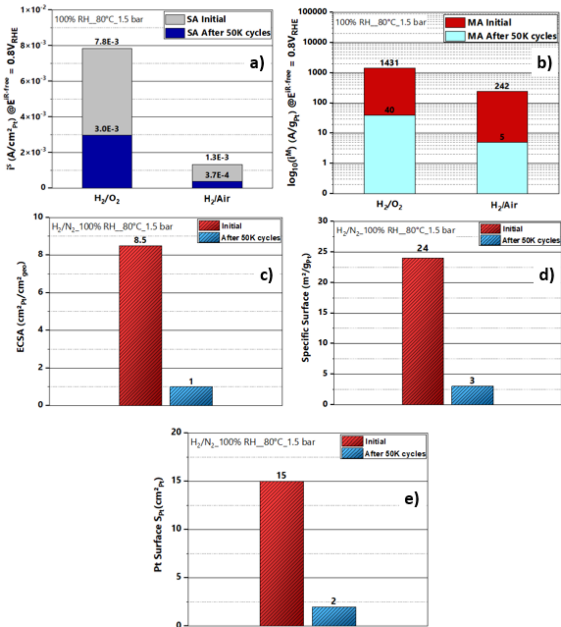
Figure IV-23: Performance comparison of Pt/C electrodes at a cathode loading of 35 μg Pt /cm 2 before degradation and after 50K potential cycles in H 2 /O 2 , H 2 /Air, and H 2 /N 2 : a) and b) specific activity and mass activity data recorded (in logarithm scale) at E IR-free =0.8 V RHE , c) ECSA values before and after degradation, d) Specific surface in m 2 /g Pt , and e) Platinum total surface before and after degradation.
