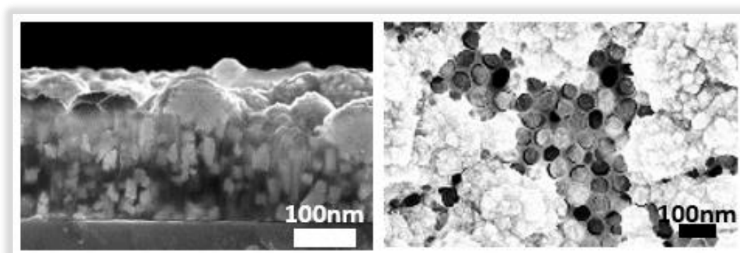
Figure III-52: SEM cross-sectional and top-view and images of the confined NiNWs galvanic displacement reaction in an \text{H}_2\text{PtCl}_6 solution at 0.1 M HCl at room temperature for 60 minutes.
