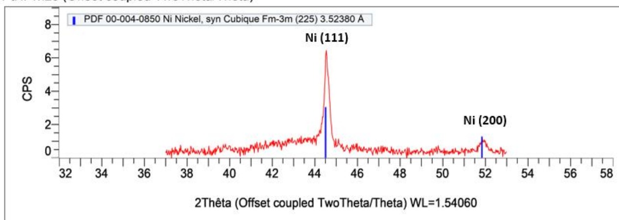
Figure III-68: XRD measurements performed on PtNiNWs at low Pt deposition where Ni peaks are clearly visible. PtNi nanowires were obtained after exposing the NiNWs sample to a K_2PtCl_4 solution at 80^\circ C for 1.5 hours.
