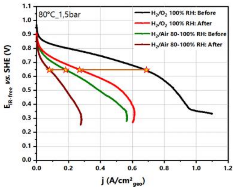
Figure IV-34: Comparison of fuel cell's polarization curves (corrected from ohmic drop) of PtNiNWs cathodes at operating conditions in the order of anode/cathode in H_2/O_2 and H_2/Air , cell temperature of 80°C, at different relative humidity values and a total pressure of 1.5 bar, 1.38 bar, 1.38-1.5 bar, and 1.5-1.38 bar at 100% RH, 80% RH, 80%-100% RH, and 100%-80% RH, respectively, before and after 50K load cycles.
