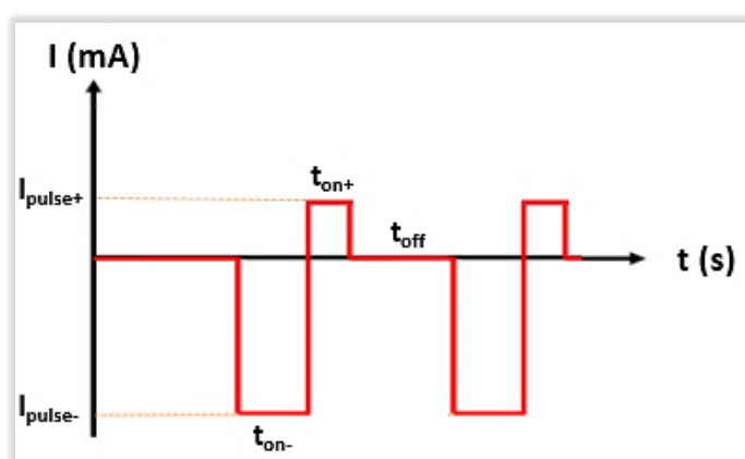
Figure III-8: Schematic diagram of the time evolution of current during pulsed electrodeposition. Applied parameters in this thesis: Each high current pulse I_{\text{pulse}-} is applied for a time t_{\text{on}-} followed by a lower current pulse I_{\text{pulse}+} for a shorter time, then a concentration recovery time t_{\text{off}} of 1s. This process is repeated for 135, the experimental number of pulses.
