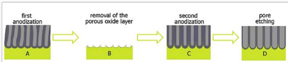
Figure II-8: Schematic representation of template-based nanoporous aluminum oxide templates. Reprinted and edited from reference.
