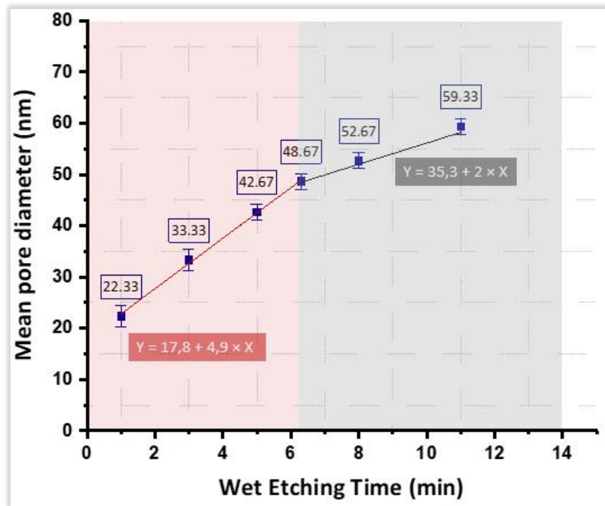
Figure II-30: Evolution of mean pore diameter size ( D_p ) as a function of wet chemical etching time of porous anodic aluminum oxide formed in 3%wt oxalic acid at 34 V. Wet etching was performed in 5%wt orthophosphoric acid at 35°C.
