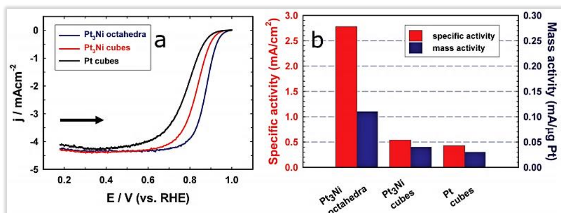
Figure III-24: a) Polarization curves for ORR on Pt 3 Ni nanostructures, Pt 3 Ni nanocubes, and Pt nanocubes supported on a rotating glassy carbon disk electrode in O 2 saturated 0.1 M HClO 4 solution at 295K; scan rate, 20 mV/s; rotation rate, 900 rpm. Catalyst loading in terms of Pt mass: Pt 3 Ni octahedra, 3.0 μg; Pt 3 Ni cube, 2.0 μg; Pt cube, 1.1 μg. The current density was normalized to the glassy carbon geometric surface area (0.196 cm 2 ). The arrow indicates the potential scan direction. b) Comparison of the OR activities on the three types of catalysts. Specific activity and mass activity were all measured at 0.9 V vs. RHE at 295 K [41].
