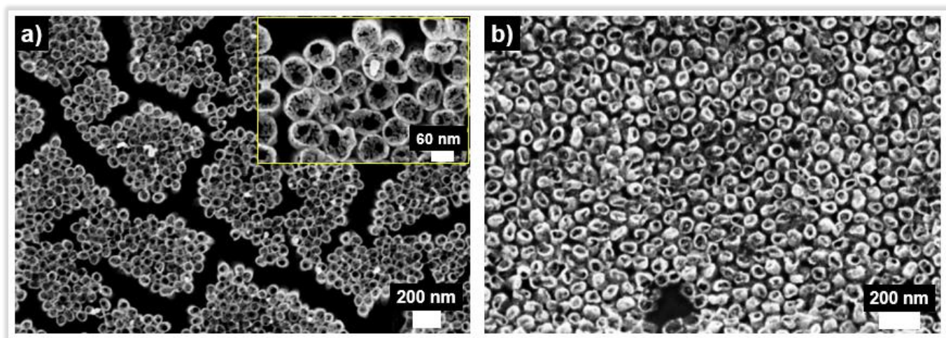
Figure IV-37 : SEM top-view images of the fabricated PtNiNTs a) before optimization (acid leaching performed on PtNiNWs on a silicon substrate), and b) after optimization (acid leaching performed on PtNiNWs transferred onto Nafion ® membrane).
