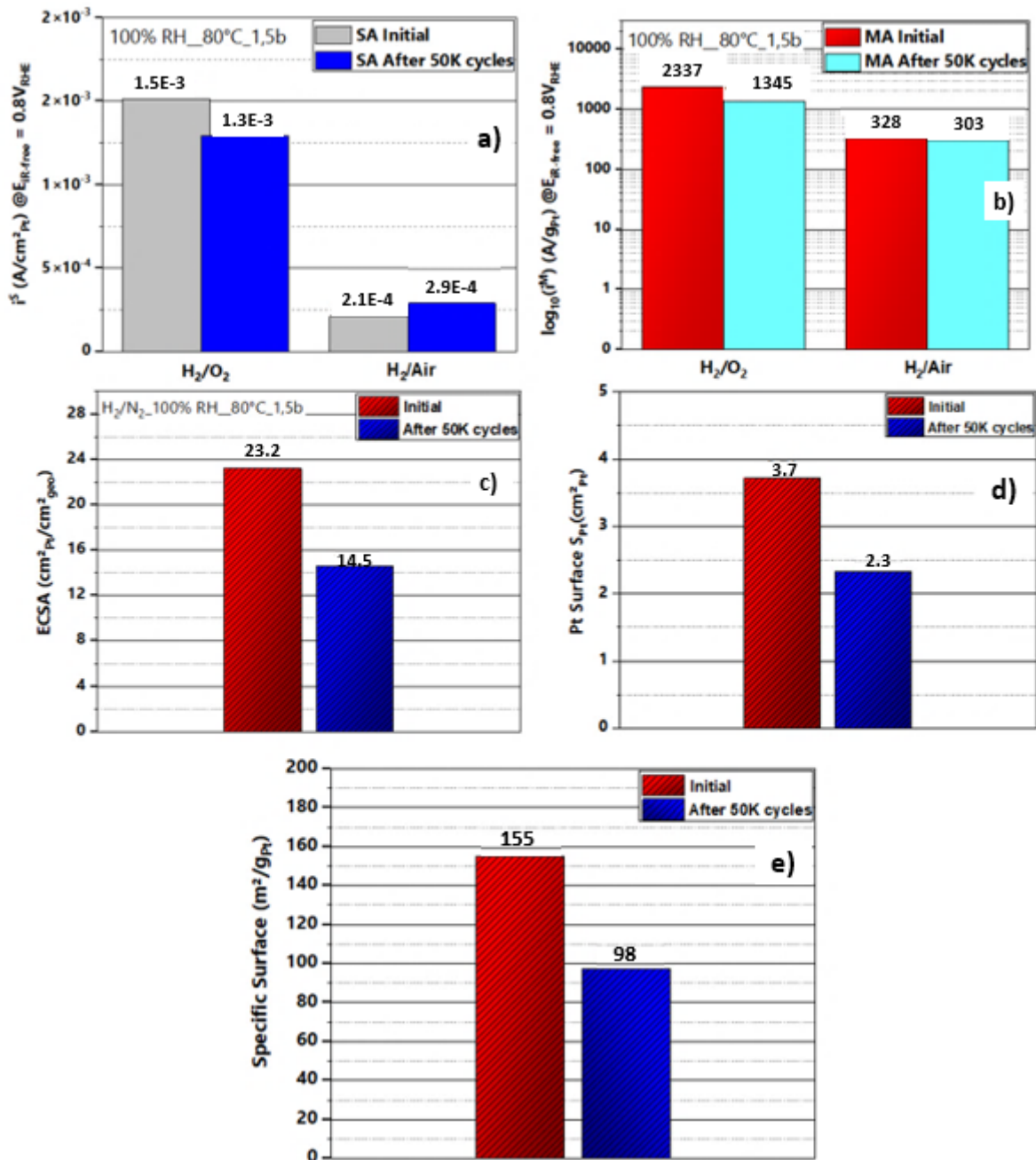
Figure IV-46: Performance comparison of the MEA with PtNiNTs at a cathode at a loading of 14 \mu g_{Pt}/cm^2 before degradation and after 50K potential cycles in H 2 /O 2 , H 2 /Air, and H 2 /N 2 : a) and b) specific activity and mass activity data recorded at E_{iR-free}=0.8 V_{RHE} , c) ECSA values before and after degradation, d) Specific surface in m^2/g_{Pt} , and e) Platinum total surface before and after degradation.
