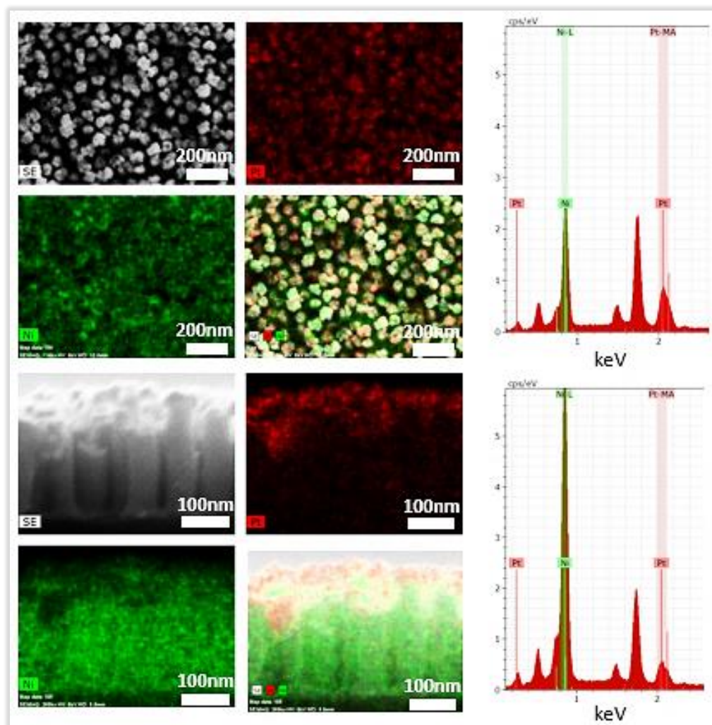
Figure III-76: Top-view and cross-sectional SEM coupled EDX analysis of the result of NiNWs GD reaction in \text{H}_2\text{PtCl}_6 solution in 0.1 M HCl HCl for 30 minutes.
