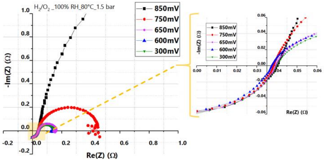
Figure IV-11: Electrochemical Impedance Spectroscopy (EIS) was performed at various voltage values, at T_{cell}=80^{\circ}C , 100% RH, wet H_2/O_2 gas flow, and a total pressure of 1.5 bar.
