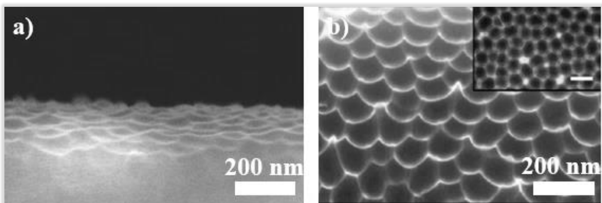
Figure II-28: Scanning electron microscopy micrographs of a) aluminum nanobowls-like surface after i/ first step anodization of aluminum thin film (1 μm) on a silicon substrate, and ii/ first etching in 5%wt Orthophosphoric acid at 35°C; b) tilted-view scanning electron microscopy image of an Al foil with nanobowl surface patterns. Reprinted from reference [18].
