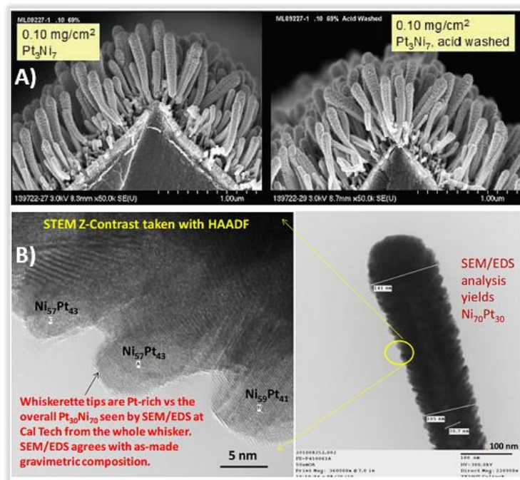
Figure III-32: A) SEM images, at originally 50 kX, of the NSTF catalysts with Pt 3 Ni 7 coatings as-made (left) and after acid washing (right). B) TEM images of roll-good fabricated Pt 3 Ni 7 alloy coated NSTF whiskers showing the composition of the whiskerettes on the whiskers' sides have a Pt-rich composition versus the overall as-made composition and composition determined from EDS of the whole whisker. Reprinted from reference [63] and [64].
