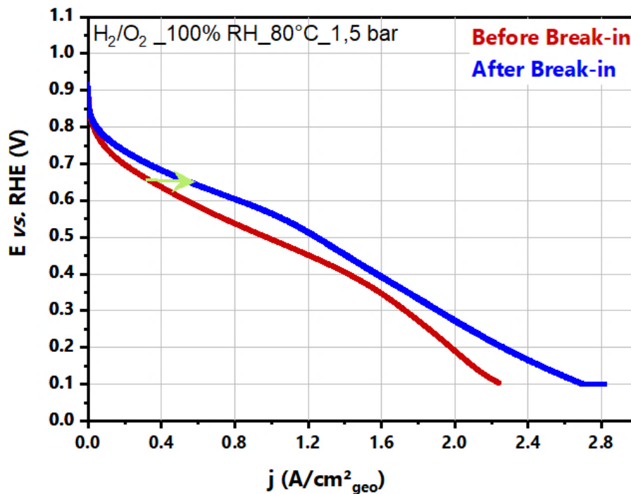
Figure IV-8: Measured polarization curve as a function of geometrical current density at T_{cell}=80^{\circ}C , 100% RH (dew points), wet H_2/O_2 gas flow, and a total pressure 1.5 bar. Red-curve: original un-corrected polarization curve, Blue-curve: polarization curve after the break-in, The homemade catalyst layer is made of Pt/Carbon ( 0.1\text{ mg}_{Pt}/\text{cm}^2 - 0.035\text{ mg}_{Pt}/\text{cm}^2 at the anode and the cathode, respectively).
