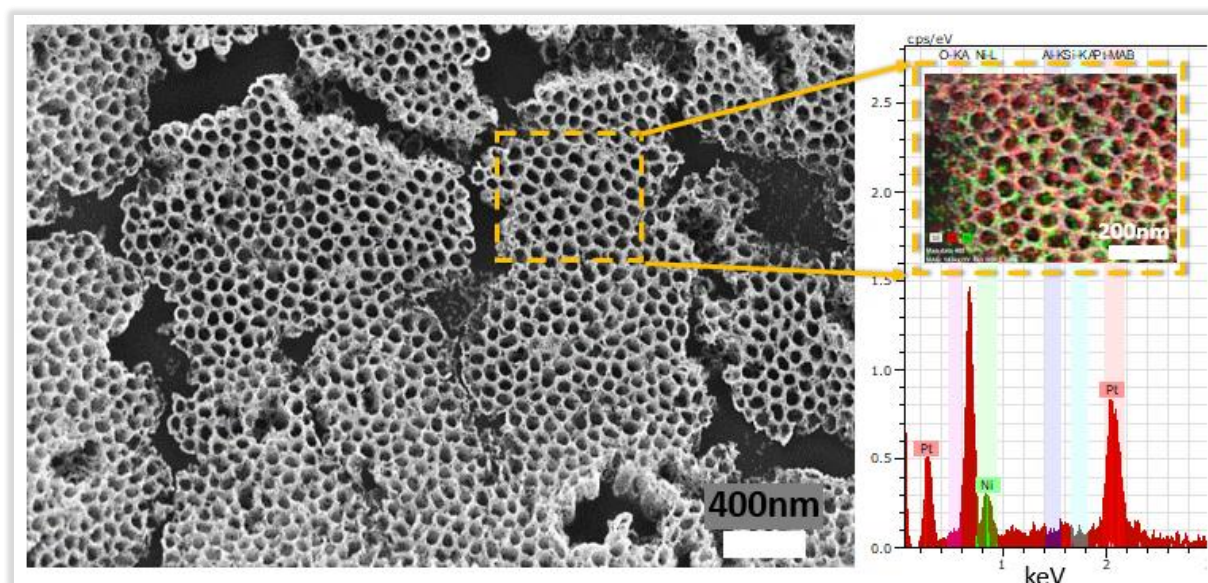
Figure III-71: SEM top of PtNi nanotubes transferred to Nafion ® membrane, obtained in a non-confined system in K 2 PtCl 4 solution heated to 80°C for 1.5 hours. After GD, the PtNiNWs were heated under H 2 /Ar atmosphere for 2 hours at 250°C. After that, PtNiNWs were transferred to the Nafion ® membrane by a hot-pressing process followed by an acid-leaching process in a sulfuric acid solution. According to the EDX quantitative analysis, the atomic ratio of Pt:Ni is 3:1.
