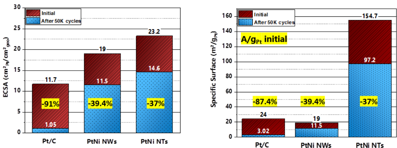
Figure IV-48: Electrochemical surface area (ECSA) and the Pt-specific surface comparison electrodes at operating conditions in H_2/O_2 , cell temperature of 80^\circ C , 100% RH and 1.5 bar, before and after 50K load cycles.
