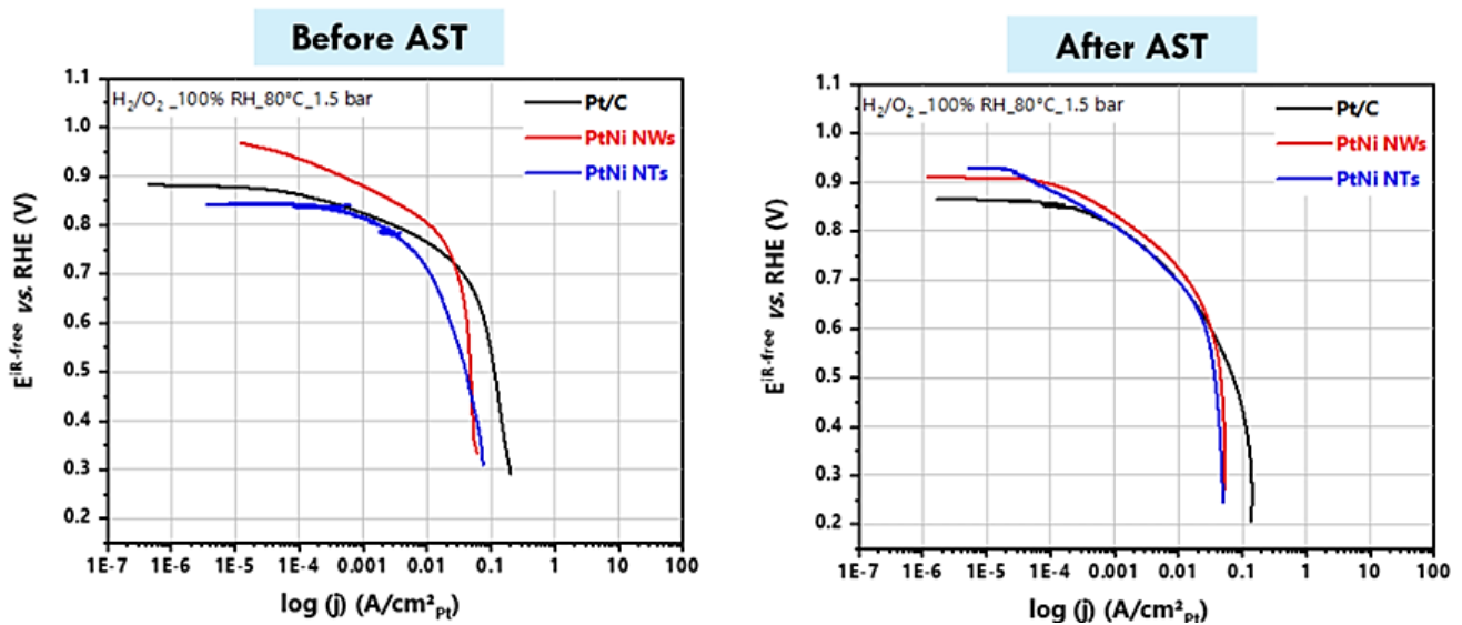
Figure IV-54: Specific Tafel plot for oxygen reduction reaction under fully humidified H_2/O_2 atmosphere at 80^\circ C and 1.5 bar, before and after AST.
