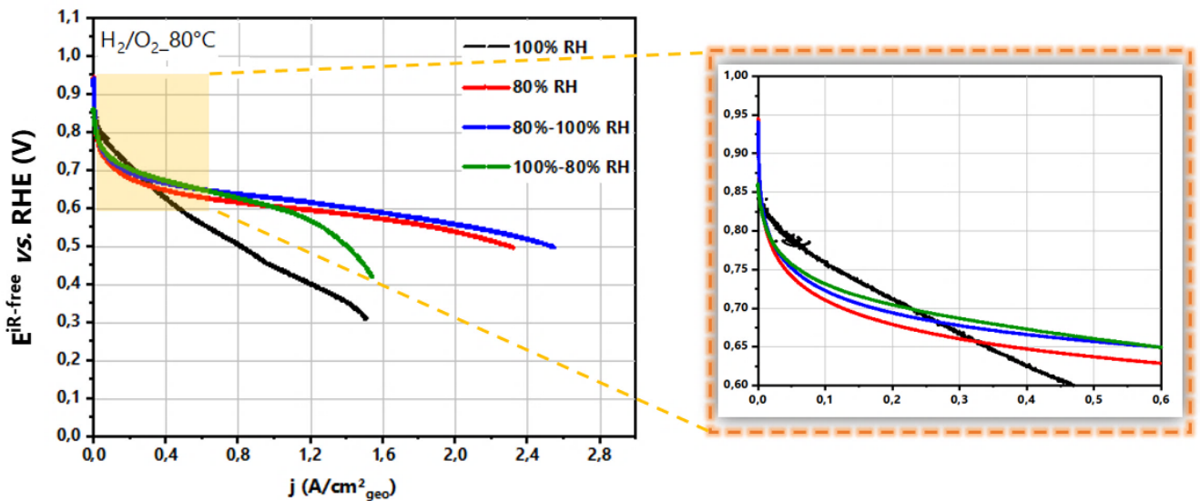
Figure IV-39: Comparison of fuel cell's ohmically-corrected polarization curves of PtNiNTs cathodes at operating conditions in the order of anode/cathode in H_2/O_2 , a cell temperature of 80^\circ C , at different relative humidity values and a total pressure of 1.5 bar, 1.38 bar, 1.38-1.5 bar, and 1.5-1.38 bar at 100% RH, 80% RH, 80%-100% RH, and 100%-80% RH, respectively.
