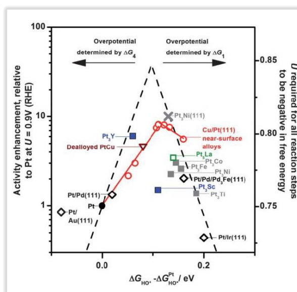
Figure III-18: Volcano plot depicting the rate of the oxygen reduction reaction and activity enhancement on Pt-based alloys as a function of hydroxyl binding energy, \Delta G_{HO^*} , both relative to pure Pt. All data are at U= 0.9 V, with respect to a reversible hydrogen electrode (RHE) from reference [35].
