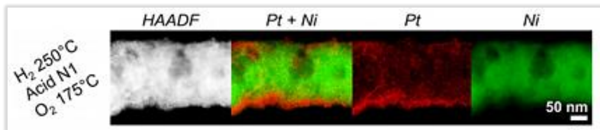
Figure III-38: STEM-HAADF of PtNi nanowires ( 7.3 \pm 0.3 wt% Pt); annealed in hydrogen to 250 °C and ex-situ acid-leached in a mixture of acetic and sulfuric acid, then and annealed in oxygen to 175°C.
