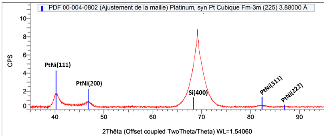
Figure III-82: XRD measurements performed on the as-prepared PtNiNWs supported on p-Si(100) synthesized in a K_2PtCl_4 solution in 0.05 M HCl at 35°C for 8 minutes.
