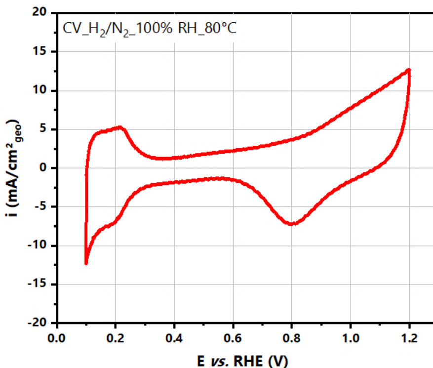
Figure IV-36: Cyclic voltammograms of PtNiNTs, recorded in fully humidified \text{H}_2/\text{N}_2 gas flow from 0.1 V_{\text{RHE}} to 1.2 V_{\text{RHE}} at 80°C with a sweep rate of 200 mV/s.
