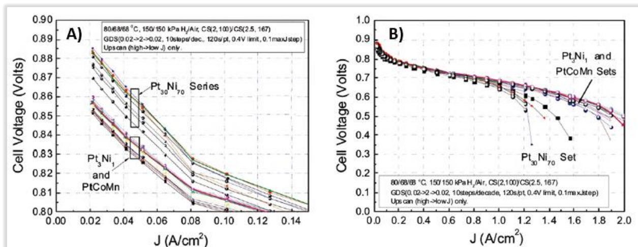
Figure III-33: A) Hydrogen/air galvanodynamic polarization curves (GDS) in the kinetic region at the conditions shown in the inset for various NSTF Pt x Ni y compositions compared to Pt 3 Ni 1 and the NSTF standard PtCoMn. B) H 2 /air GDS polarization curves at the conditions shown in the inset for NSTF MEA's with the Pt 3 Ni 70 composition versus the Pt 3 Ni 1 and standard PtCoMn. Reprinted from reference [63].
