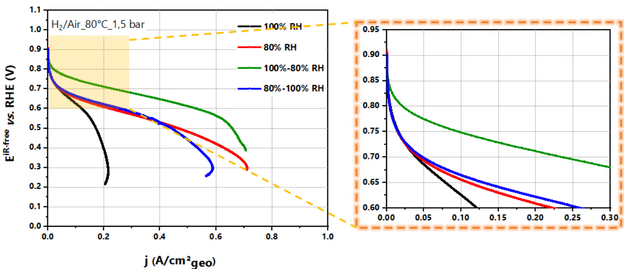
Figure IV-40: Comparison of fuel cell's ohmically-corrected polarization curves of PtNiNTs cathodes at operating conditions in the order of anode/cathode in H_2/Air , a cell temperature of 80^\circ C , at different relative humidity values and a total pressure of 1.5 bar, 1.38 bar, 1.38-1.5 bar, and 1.5-1.38 bar at 100% RH, 80% RH, 80%-100% RH, and 100%-80% RH, respectively.
