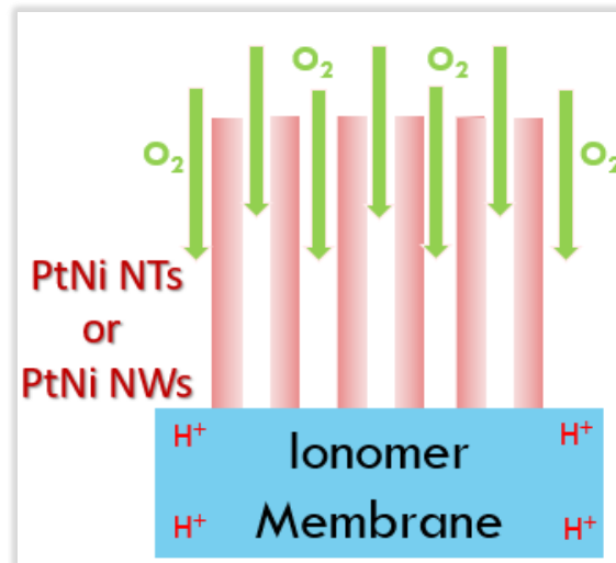
Figure I-1: Scheme of the cross-section of an oriented carbon-free PtNi nanotube transferred onto the Nafion ® membrane.
