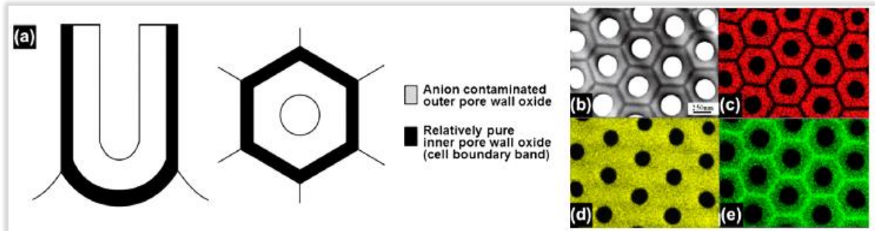
Figure II-17: a) Schematics illustrating the duplex structure of pore walls of porous AAO: vertical (left) and transverse (right) cross-sections. TEM plane view (b) of H_3PO_4 -AAO and the corresponding X-ray diffraction maps of the elements: (c) phosphorus, (d) oxygen, and (e) aluminum [46].
