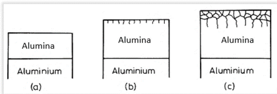
Figure II-4 : Schematic diagram illustrating the development of penetration paths, from the precursors (surface defects) to pores, during anodizing in chromic acid. Reprinted from reference [5].
