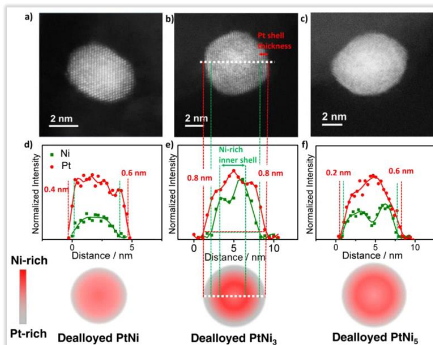
Figure III- 26: High-resolution HAADF-STEM images of dealloyed PtNi a), PtNi 3 b), and PtNi 5 Nanoparticles (NPs) c), and EELS line compositional profiles d-f) across the NPs, respectively. Bottom line: Structural model of distinctly different compositional core-shell fine structures of dealloyed Pt x Ni 1-x catalysts. Extracted from reference [48].
