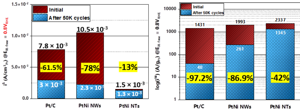
Figure IV-49: Specific and Mass activity comparison for Pt/C, PtNiNWs, and PtNiNTs electrodes at E_{IR-free}=0.8 V_{RHE} at operating conditions in H_2/O_2 , cell temperature of 80^\circ C , 100% RH and 1.5 bar, before and after 50K load cycles.
