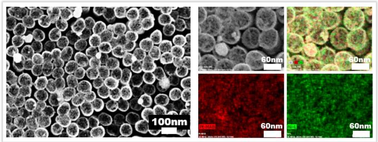
Figure III-70: SEM top-view image of quasi-porous PtNiNWs before the complete detachment from the silicon substrate and its corresponding EDX analysis.
