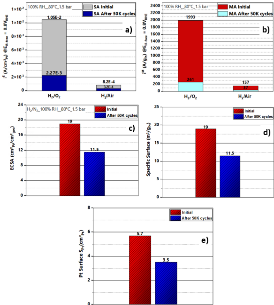
Figure IV-35: Performance comparison of the MEA with PtNiNWs at a cathode at a loading of 100 \mu\text{g}_{\text{Pt}}/\text{cm}^2 before degradation and after 50K potential cycles in H 2 /O 2 , H 2 /Air, and H 2 /N 2 : a) and b) specific activity and mass activity data recorded at E_{IR-free} = 0.8 V_{RHE} , c) ECSA values before and after degradation, d) Specific surface in m 2 /g Pt , and e) Platinum total surface before and after degradation.
