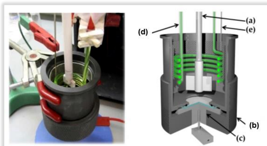
Figure II-23 : Electrochemical cell setup used for anodizing aluminum on p-type silicon substrate: a) Stirrer, b) 3D model of the PVC cell, c) Metal cap that ensures electrical contact and mechanical cohesion between the cell and the sample (electrode), d) Flowing cooling liquid system to adjust the temperature of the electrolyte, e) Cylindrical platinum gauze as counter-electrode.
