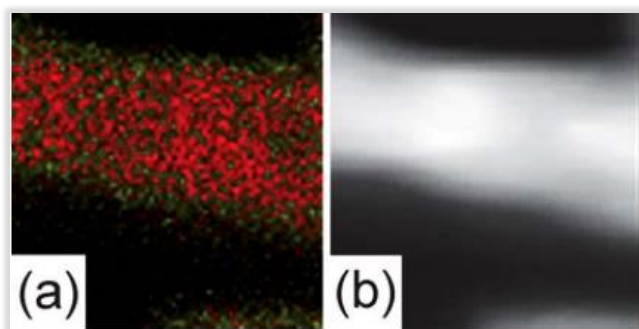
Figure III-34: PtNi 5 after core-shell structure treatment and acid test: (a) In the overlapped mapping, the red points indicate Ni, and the green points are Pt. (b) The wire where mapping was executed.
