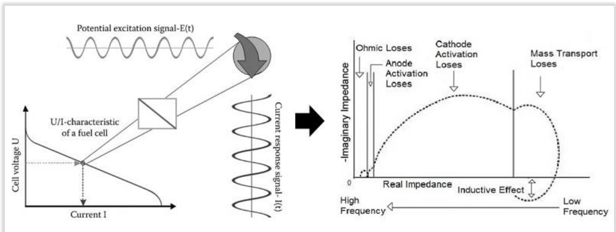
Figure IV-10: Illustration displaying the principle of the electrochemical impedance spectroscopy as a perturbative characterization of the dynamics of an electrochemical process and the Nyquist plot with the main physical phenomena extracted.
