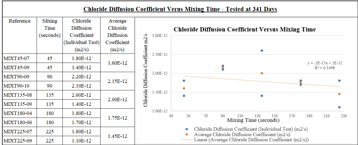
Figure 4.23 - Chloride Diffusion Coefficient - MIXT Series
