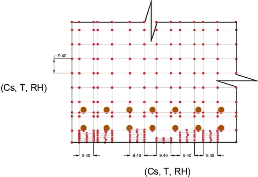
Figure 6.11 - Beam Subjected to a chloride concentration C_s , an ambient temperature T , and a relative humidity RH
