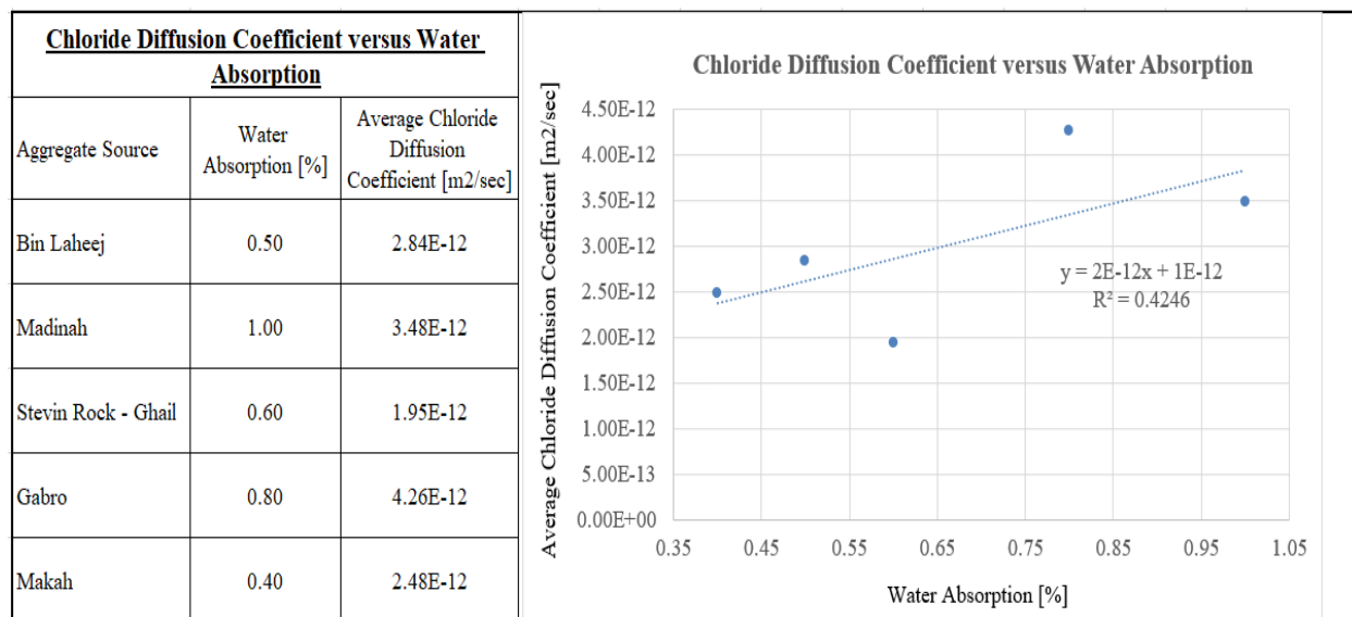
Figure 2.12 - Chloride Diffusion Coefficient versus Water Absorption
