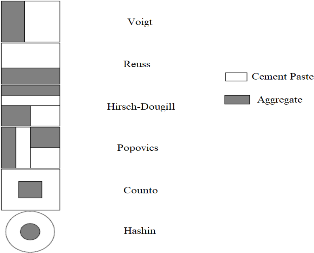
Figure 2.26 - Modulus of Elasticity Illustration Models
