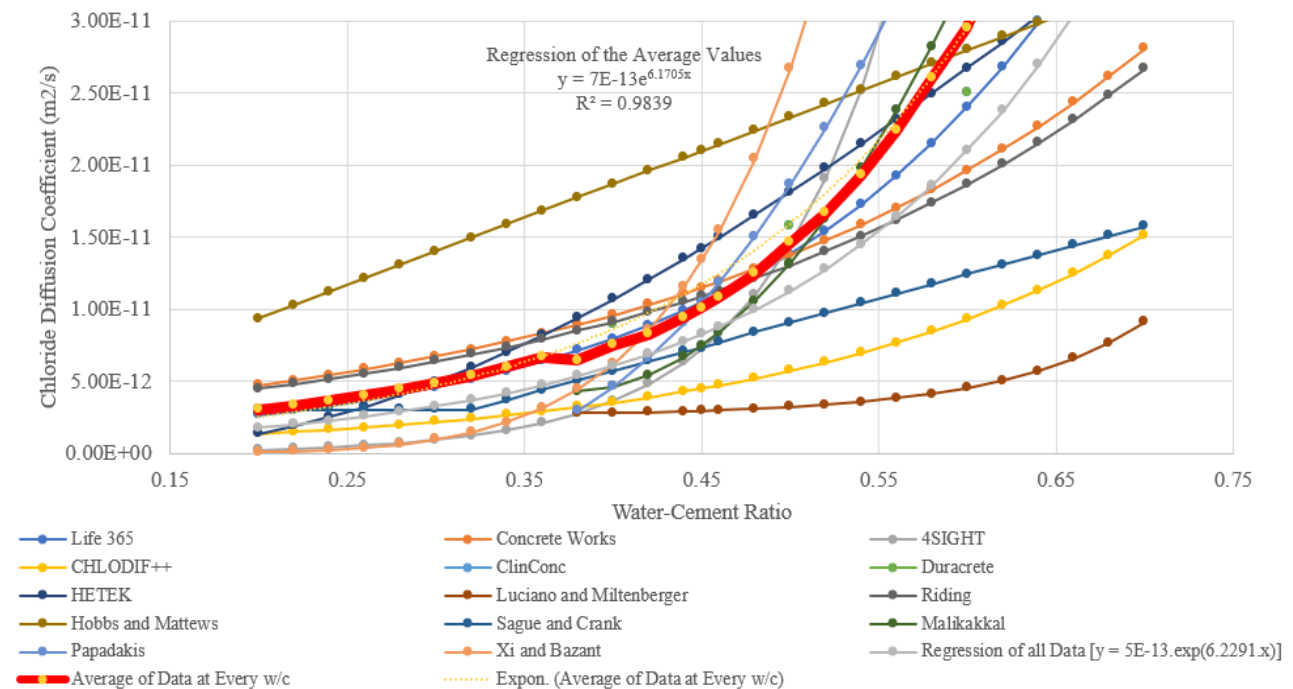
Figure 6.1 - Chloride Diffusion Coefficient (Different Models; Cement Content = 425kg/m3)
