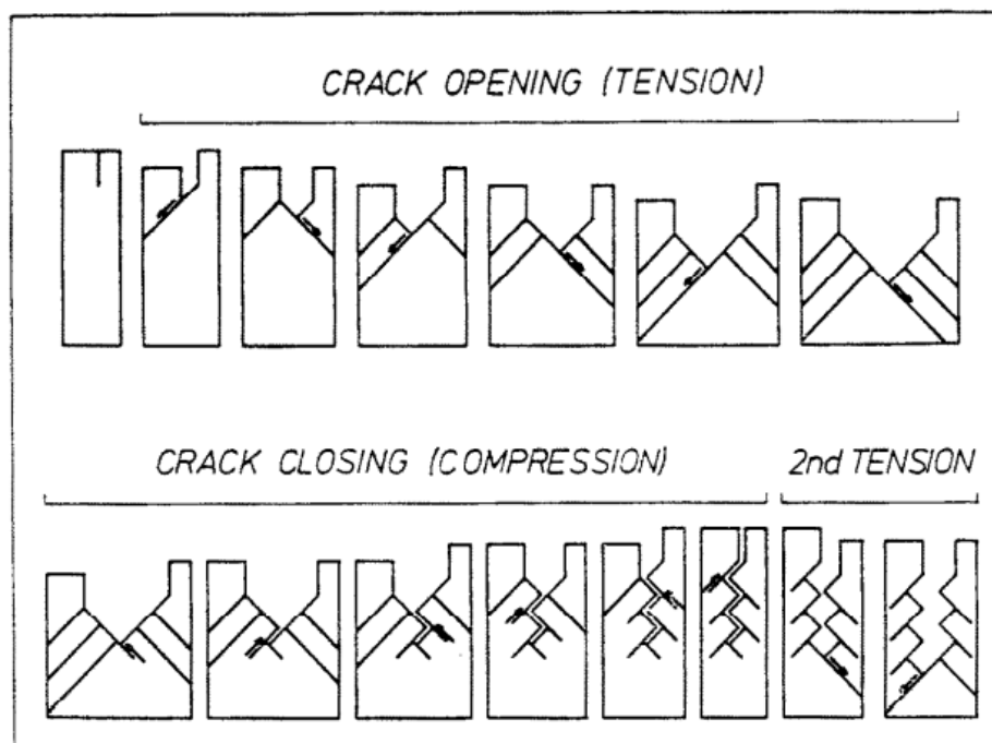
Figure 2-20: Schematic illustration of the blunting-resharpening model. Crack tip blunting occurs during tension with plastic slip activity and the resharpening occurs during compression with reversal slip. Due to the non full reversibility of the plastic slip, the crack propagates [Neumann, 1974]
