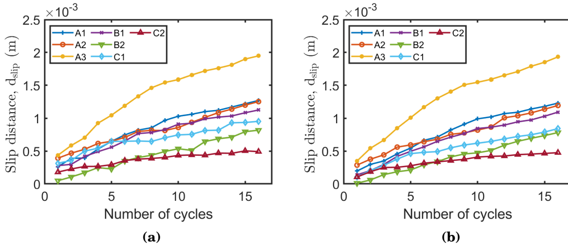
Figure 4-22: Evolution of the slip distance computed, for different crack configurations and for \Delta K = 2 \text{ MPa}\sqrt{\text{m}} . (a) at maximum load ( K_{max} = 2 ) and (b) at minimum load ( K_{min} = 0 ). The cumulative plastic slip in the crack-tip region increases during cyclic loading.
