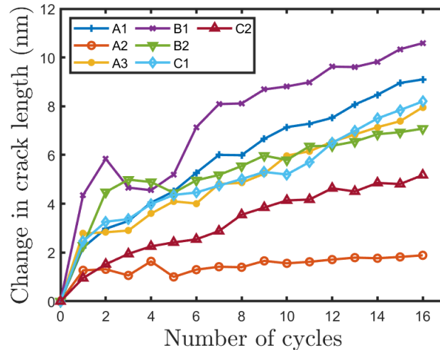
Figure 5-1: Change in crack length during cyclic loading for different crack orientations applying \Delta K = 2.5 \text{ MPa}\sqrt{\text{m}} and R = 0 . Whatever the orientation, two main regimes are observed: a transient regime at the beginning then a quasi steady regime.
