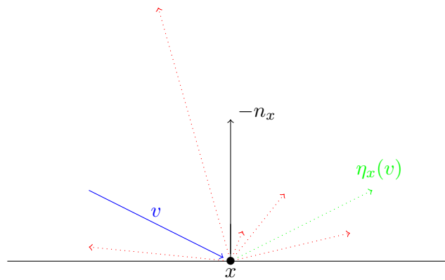
Fig. 1.4 The Maxwell boundary condition. The situation is the same as in the case of the pure diffusive reflection, except that the outgoing velocity vector is \eta_x(v) with probability 1 - \alpha(x) .
