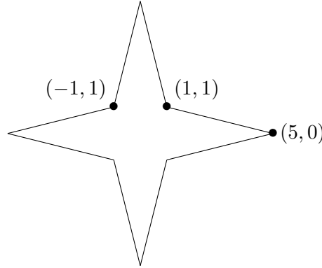
Fig. 3.1 Star-shaped domain in \mathbb{R}^2 .
