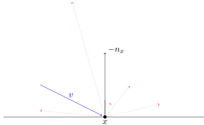
Fig. 1.3 The pure diffusive boundary condition. Dotted red vectors are possible outgoing velocities.
