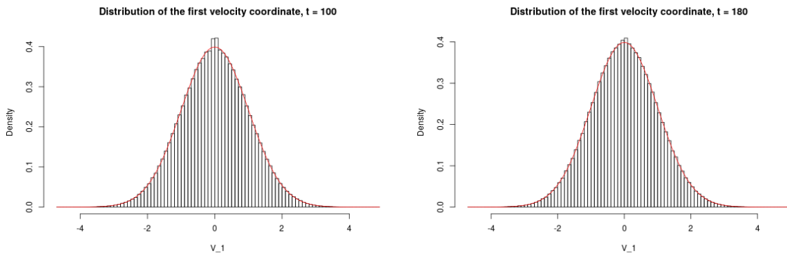
Fig. 3.10 Distribution of the first space velocity coordinate at time t = 100 and t = 180 in the case where the initial data is given by (3.3.2).
