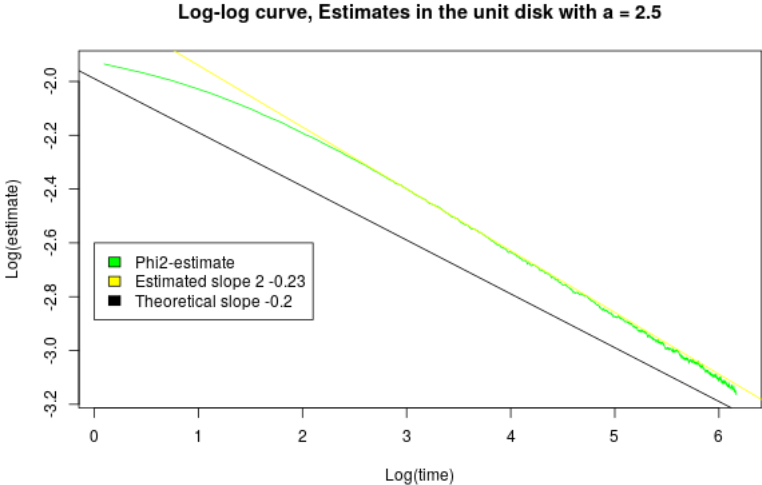
Fig. 3.21 Convergence of the \phi_2 estimate, in the case where a = 2.5 and the reflection law has variance 1, with f_0 is given by \frac{M_{2.5,0.01}}{|D|} .
