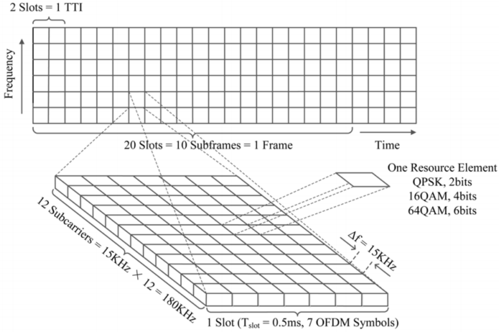
Figure 2.3: Time-frequency resources in LTE [4]
