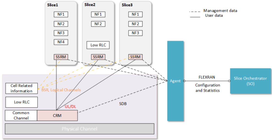
Figure 3.2: 2 level MAC scheduler system model [12]
