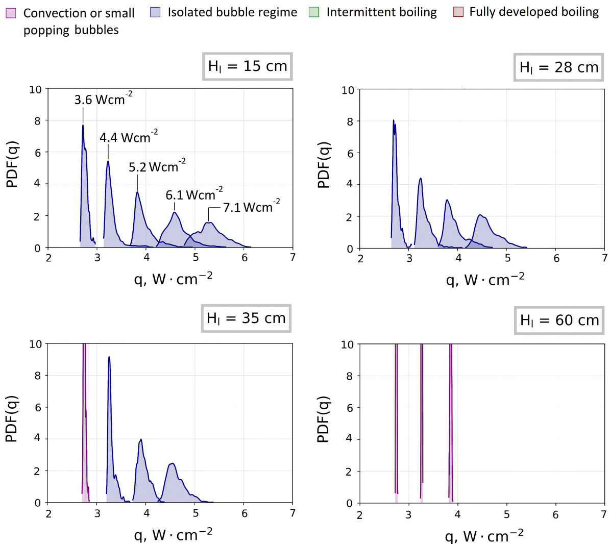
Figure B.4: PDF graphs for vapor pressure p_v = 4.1 kPa, S_q = 2.8 \mu m (applied heat fluxes for the graphs from left to right: 3.6 W \cdot cm^{-2} , 4.4 W \cdot cm^{-2} , 5.2 W \cdot cm^{-2} , 6.1 W \cdot cm^{-2} and 7.1 W \cdot cm^{-2} ).
