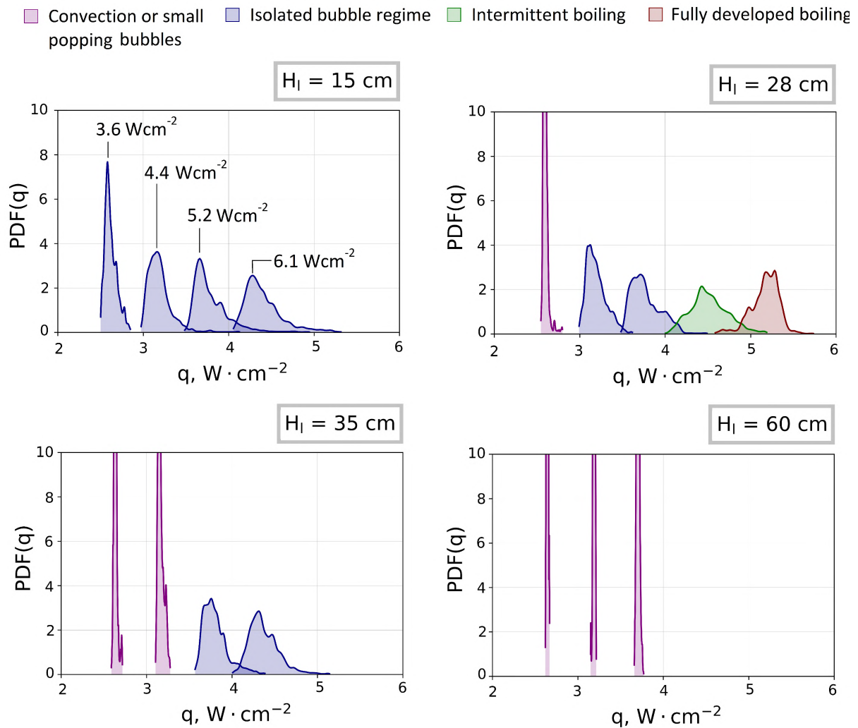
Figure B.2: PDF graphs for vapor pressure p_v = 4.1 \text{ kPa} , S_q = 3.5 \mu\text{m} (applied heat fluxes for the graphs from left to right: 3.6 \text{ W} \cdot \text{cm}^{-2} , 4.4 \text{ W} \cdot \text{cm}^{-2} , 5.2 \text{ W} \cdot \text{cm}^{-2} , 6.1 \text{ W} \cdot \text{cm}^{-2} and 7.1 \text{ W} \cdot \text{cm}^{-2} ).
