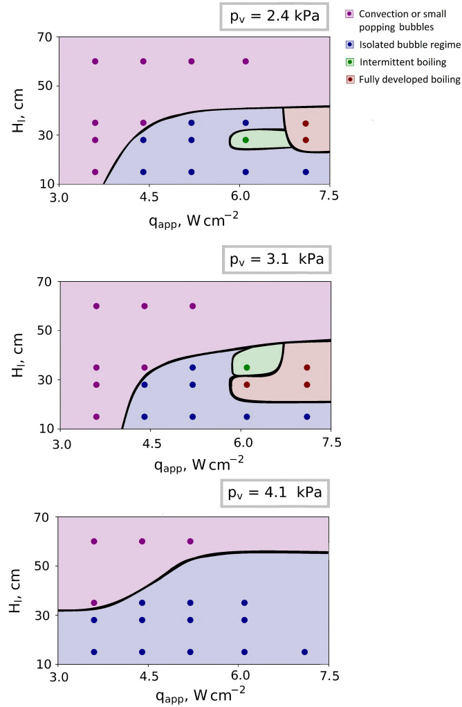
Figure 4.19: Boiling regime maps created for various pressures, liquid levels and applied heat fluxes.
