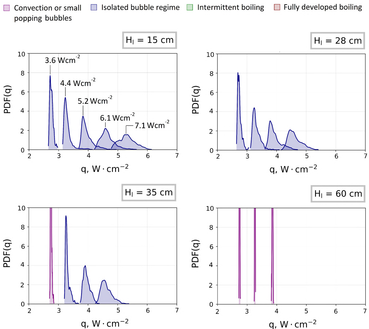
Figure B.4: PDF graphs for vapor pressure p_v = 4.1 \text{ kPa} , S_q = 2.8 \mu\text{m} (applied heat fluxes for the graphs from left to right: 3.6 \text{ Wcm}^{-2} , 4.4 \text{ Wcm}^{-2} , 5.2 \text{ Wcm}^{-2} , 6.1 \text{ Wcm}^{-2} and 7.1 \text{ Wcm}^{-2} ).
