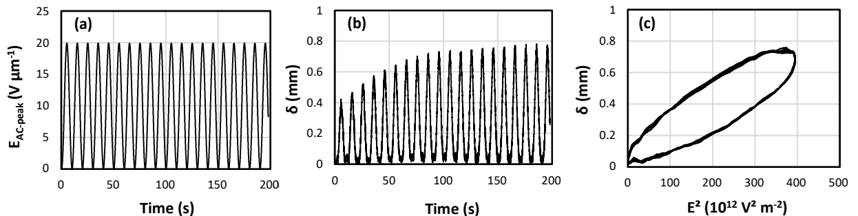
Fig. 3.4. Example of bender measurements at 0.1 Hz: (a) electric field applied to PU with electrodes applied and tip displacement versus (b) time and (c) the square of the electric field.
