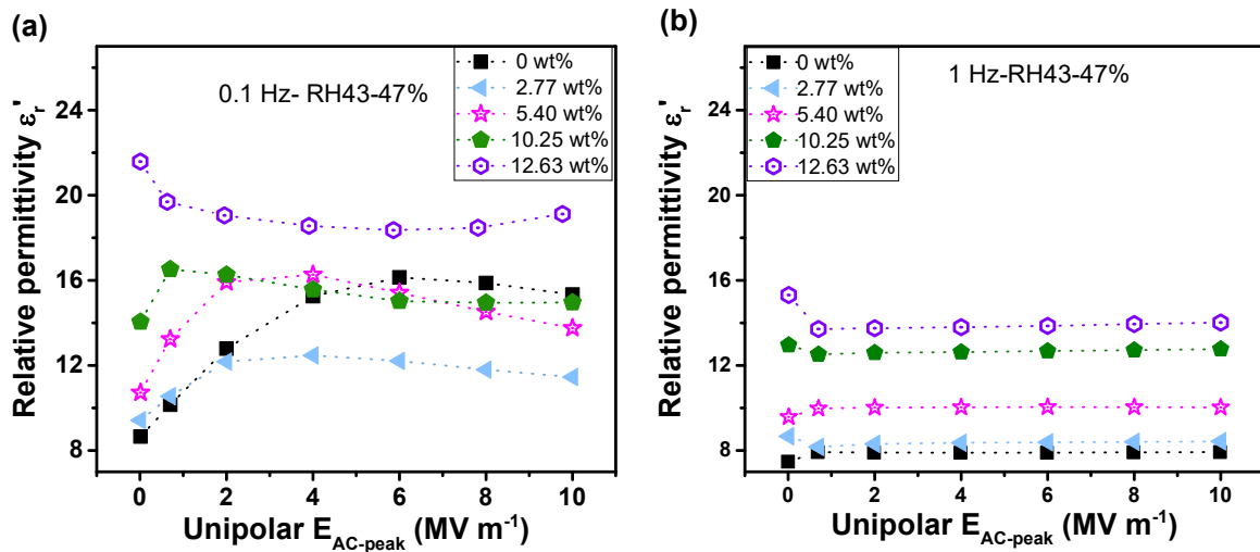
Fig. 5.2. Evolution of the permittivity of PU and PU/OFG composites versus electric field at RH 43%-47%: (a) 0.1 Hz, (b) 1 Hz (lines for guiding eyes).
