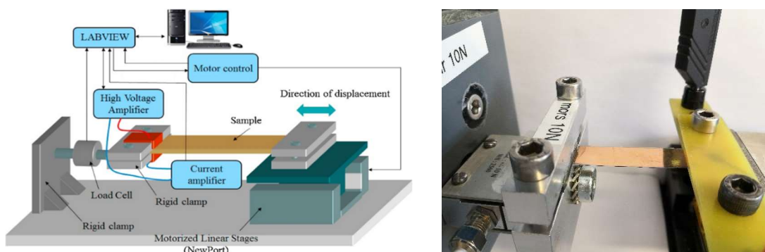
Fig. 2.10. Schematic 36 and photo of the mechanical characterization setup.
