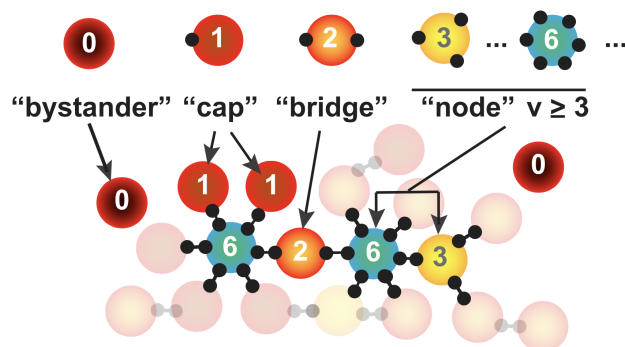
Figure 1.4 – Network-based classification of the droplet components. Valence ( v ) of the biocondensate member: v = 0 (bystander), v = 1 (cap); v = 2 (bridge), v > 2 (node) [185].
