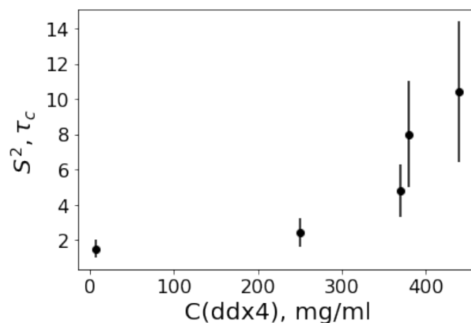
Figure 5.1 – The dependency of S^2\tau_C on a protein concentration in the sample. Values are taken from Table S1 [21]
