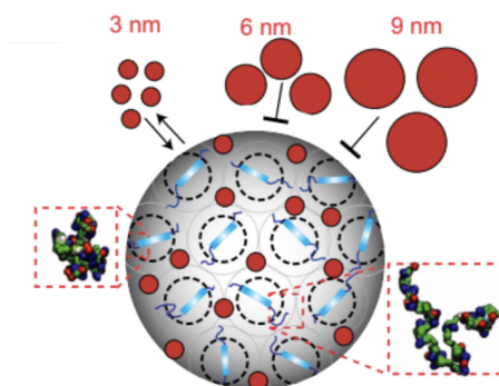
Figure 2.8 – Schematic illustration of the droplets probe-size-dependent permeability [212].
