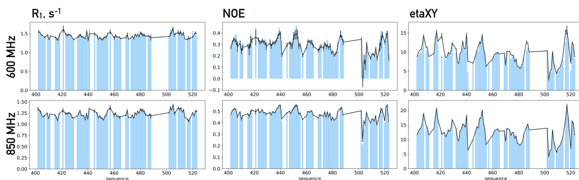
Figure 5.16 – Fitted relaxation rates of N_{tail} in a condensed state.
