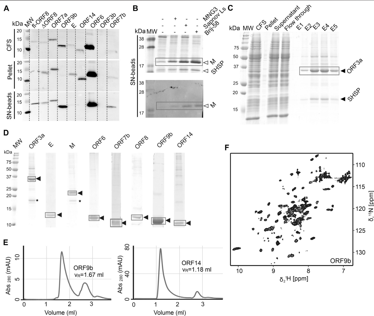
FIGURE 6 | Cell-free protein synthesis of accessory ORFs and structural proteins E and M. (A) Screening for expression and solubility of different ORFs using small-scale reactions. The total cell-free reaction (CFS), the pellet after centrifugation, and the supernatant (SN) captured on magnetic beads coated with Strep-Tactin were analyzed. All tested proteins were synthesized, with the exception of ORF3b. MW, MW standard. (B) Detergent solubilization tests using three different detergents, here at the example of the M protein, shown by SDS-PAGE and Western Blot. (C) Proteins are purified in a single step using a Strep-Tactin column. For ORF3a (and also for M), a small heat-shock protein of the HSP20 family is copurified, as identified by mass spectrometry (see also * in Panel D). (D) SDS-PAGE of the ^2\text{H} , ^{13}\text{C} , ^{15}\text{N} -labeled proteins used as NMR samples. Yields were between 0.2 and 1 mg protein per mL wheat-germ extract used. (E) SEC profiles for two ORFs. Left, ORF9b migrates as expected for a dimer. Right, ORF14 shows large assemblies corresponding to approximately 9 protein units and the DDM detergent micelle. (F) 2D ^{15}\text{N} , ^1\text{H} -BEST-TROSY spectrum of ORF9b, recorded at 900 MHz in 1 h at 298 K, on less than 1 mg of protein. See Supplementary Tables S113–S119 and Supplementary Tables S119, S120 for technical and experimental details regarding this figure.
