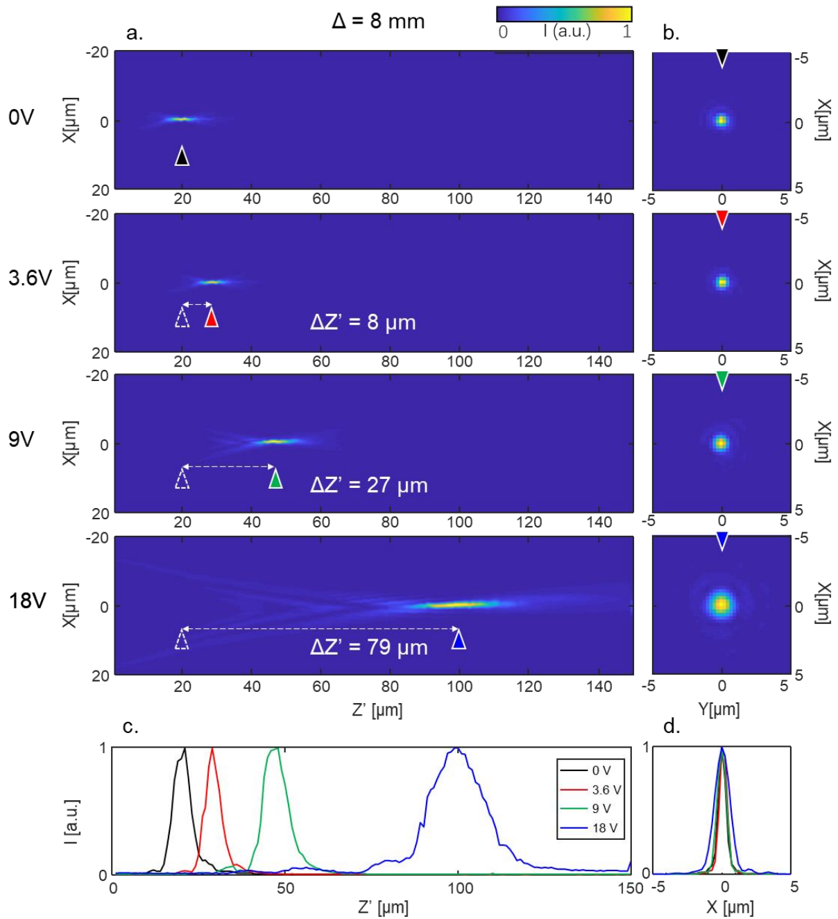
Figure 4.10 Defocused point source, with \Delta = 8\text{mm} , V = 0\text{V} , 3.6\text{V} , 9\text{V} and 18\text{V} . (a) XZ projection of the PSF defocused by SL with different voltages. (b) xy-projection of PSF on focus. (c) PSF profile along the optical axis (z-direction). (d) PSF profile along the x-direction. The excitation source is generated by 1 pixel on the DMD.
