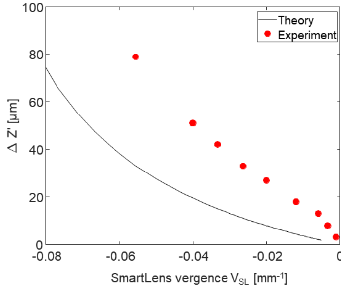
Figure 4.8 Theoretical and experimental relations between V_{SL} and \Delta Z' (with \Delta=8\text{mm} , the diameter of SL D_{SL}=540\mu\text{m} , f_3=125\mu\text{m} , M_{objective}=20 , f_{TL}=180\text{mm} ). f_{SL} is estimated from Figure 4.5(b) for each voltage.
