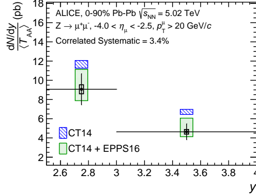
Figure 1.15: Z boson invariant yield as a function of rapidity in Pb–Pb collisions at \sqrt{s_{NN}} = 5.02 TeV. Figure taken from [95].
