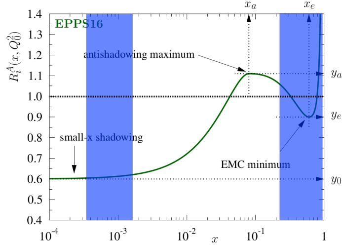
Figure 4.2: Nuclear modifications as a function of bjorken- x . The two blue bands indicate the bjorken- x probed simultaneously in Pb–Pb collisions at \sqrt{s_{NN}} = 5.02 TeV at 2.5 < y < 4.0 at ALICE. Figure adapted from [63].
