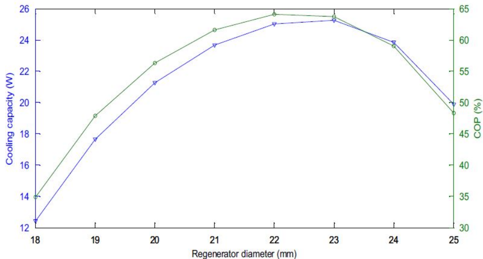
Figure 2.21: Stirling refrigerator performances versus regenerator diameter [130].
