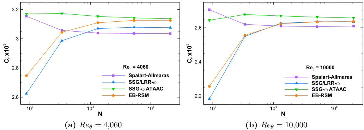
Figure 4.2: Mesh convergence for the flat plate
