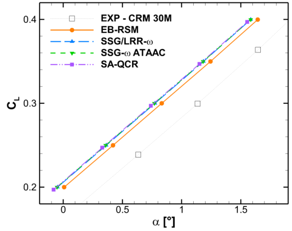
(a) Lift
