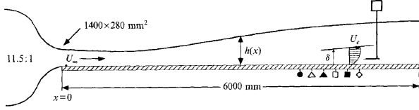
Figure 12: Skåre & Krogstad experiment configuration [14]
