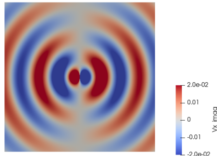
Figure 2.25: Analytical solution for u_x with the sources \mathbf{f} = \nabla \delta , \tilde{\mathbf{f}} = 0 .
