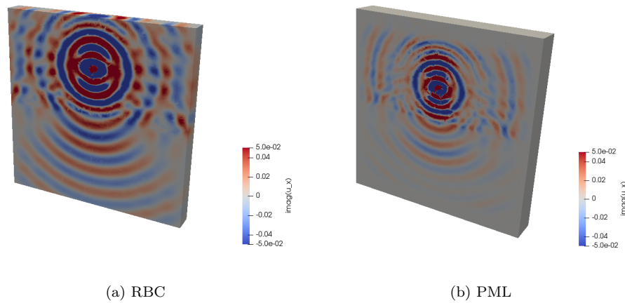
Figure 4.38: Horizontal component of solid velocity u_x on the layered domain for two types of artificial boundaries, for order of interpolation 3 at frequency f = 2\text{kHz} .
