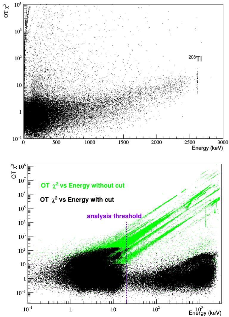
FIGURE 4.5: Top panel : distribution of OT \chi^2 as a function of energy for one channel in calibration data. Bottom panel distribution of OT \chi^2 as a function of energy for the 10 best channels in background data. The OT \chi^2 is represented without the cut in green and in black with the cut.
