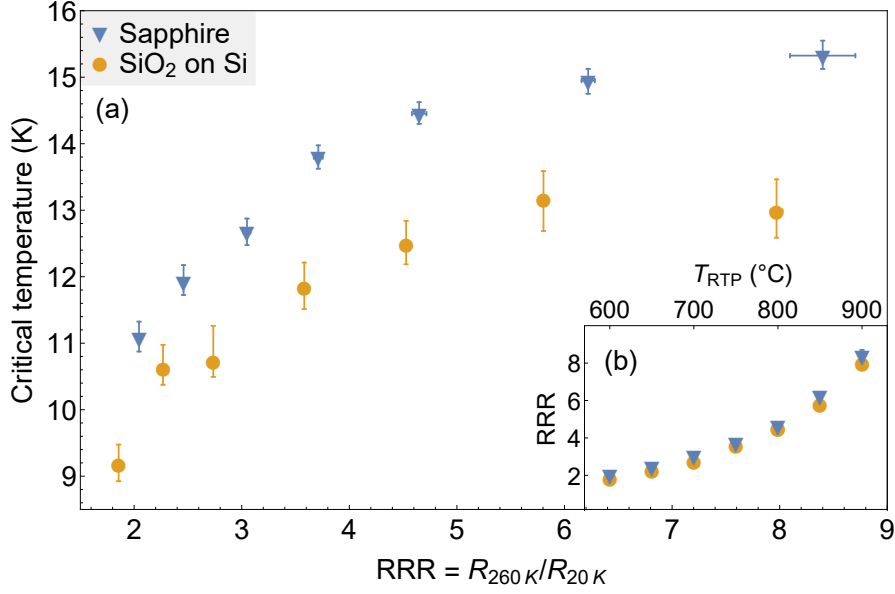
Figure 3.10: (a) The residual resistance ratio RRR = R_{260K}/R_{20K} is a measure of material quality, where any resistance that is residual after the thermal electron-phonon scatterings are suppressed, is assumed to be due to impurities and defects. For any given RRR, there is a large difference in T_c between the two substrates, indicating that it is affected by something other than the quality of the V 3 Si. (b) A near-perfect match between the RRRs measured on sapphire and silicon shows that the substrate has little influence on the quality of the V 3 Si film.
