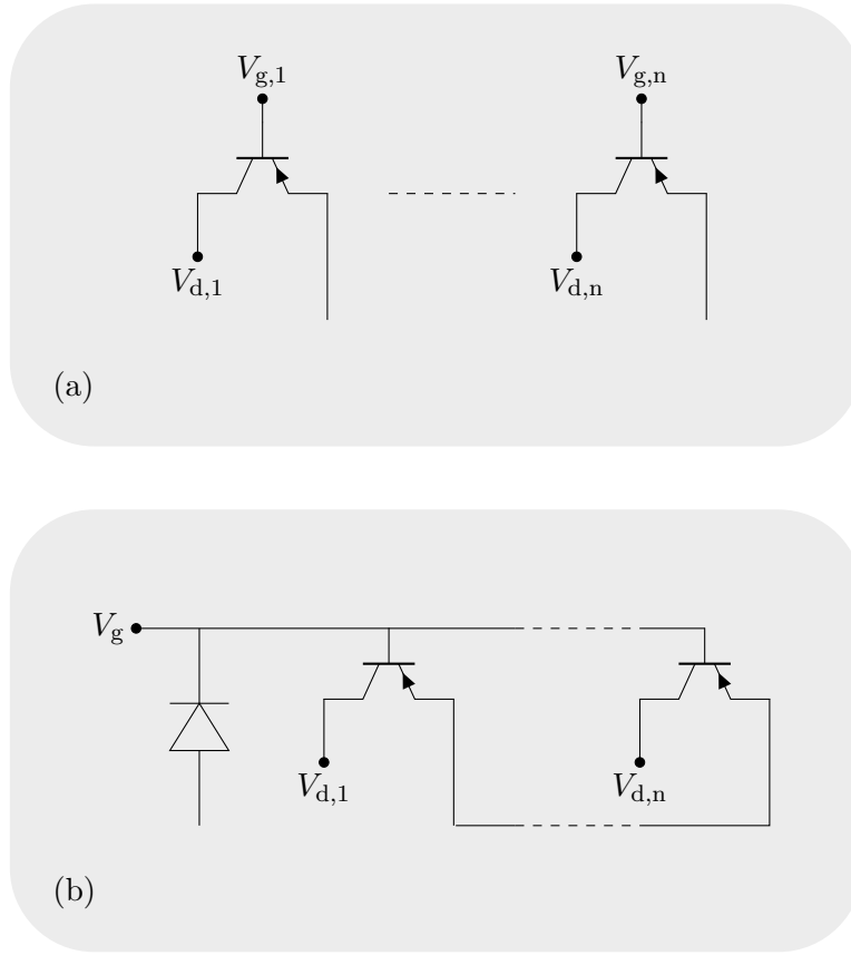
Figure B.4: (a) The separate PMOS transistors (all devices on E,F:19; drains 19–31 on E,F:22) each have their own source, drain and gate contact pads. A voltage was systematically applied to the drain, and the current measured from the source. (b) The connected PMOS transistors (drains 1–14 on E,F:22, all devices on E,F:23) share the source and the gate, each has its own drain contact. A parallel reverse biased ESD diode prevents large currents from flowing across the gate.
