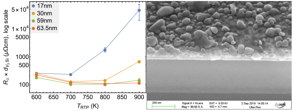
(a) Normalized sheet resistance vs T_{RTP} for selected thicknesses. (b) 30 nm V_3Si on 300 nm SiO_2 , T_{RTP} = 800^\circ\text{C} .
