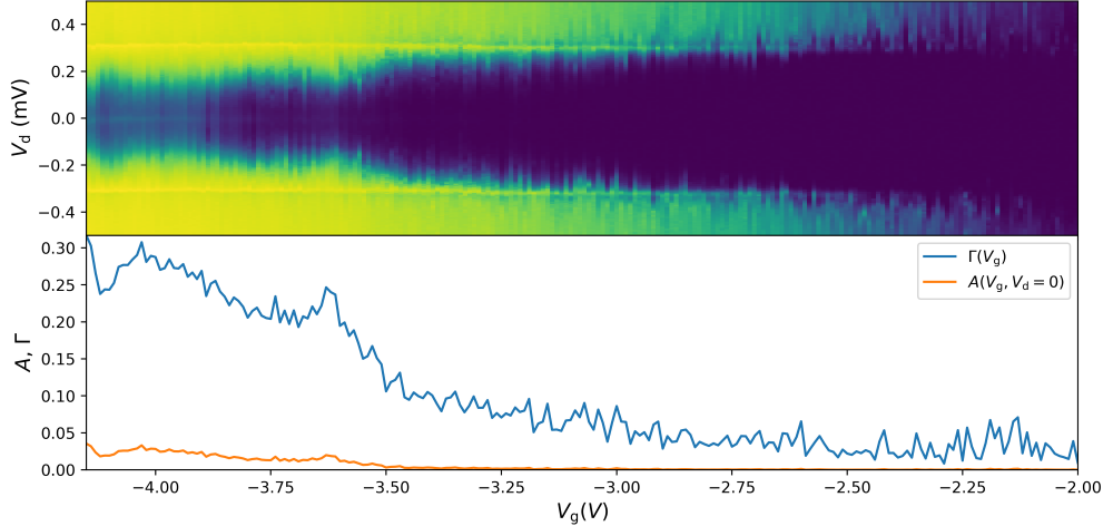
Figure 4.24: Data from device D61D04. (Top) The differential conductance of device D61D04 versus gate and drain voltage. On the left, around V_d = 0 , a zero-bias conductance peak (ZBCP) can be observed. (Bottom) Around the same range in V_g , the extracted A(E = 0) increases, consistent with this peak being due to the proximity effect.
