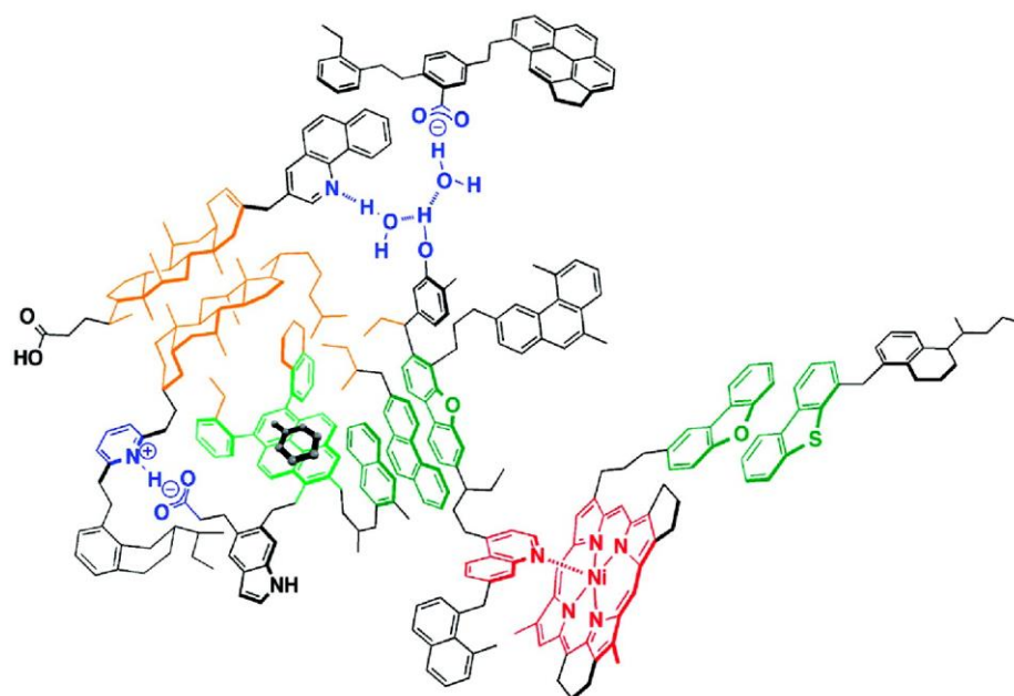
Figure 1.6 Supramolecular assembly model of asphaltene, proposed by Murray R. Gray 146
