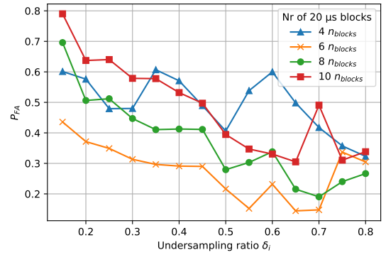
(f) Scenario 3, medium SNR (SNR= 6 dB).
