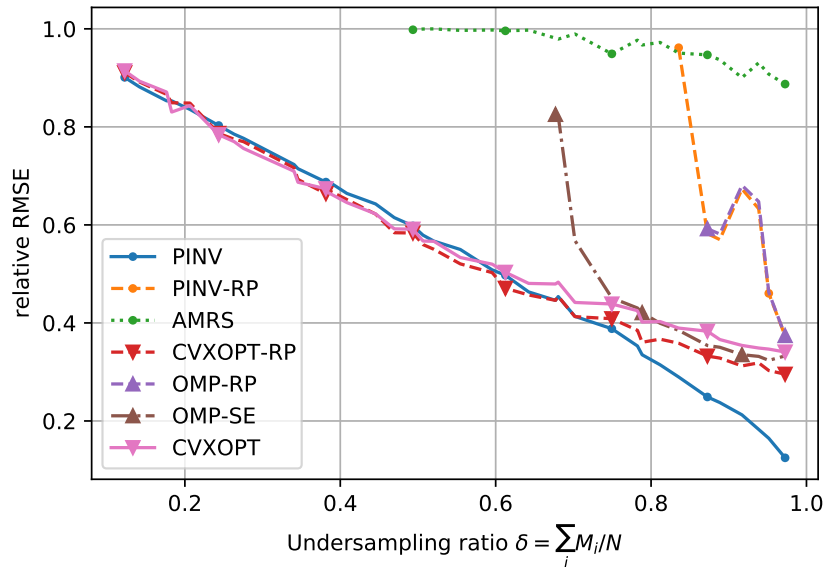
Figure 4.18: Relative RMSE versus undersampling ratio \delta for traffic scenario 3 (high traffic) in the medium SNR regime (SNR = 6 dB).
