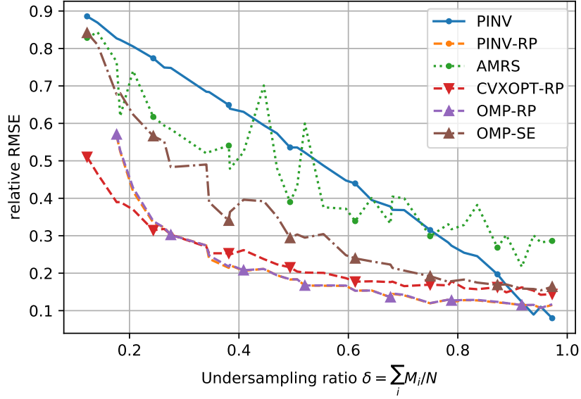
Figure 4.12: Relative RMSE versus undersampling ratio \delta for traffic scenario 2 (medium traffic) in the high SNR regime (SNR = 9 dB). Solvers use the actual signal support for USLE resolution (when applicable).
