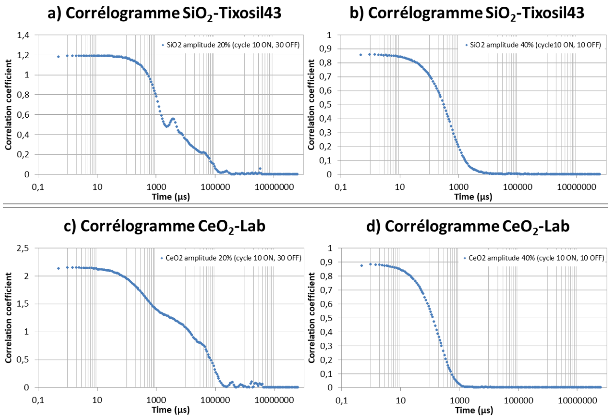
Figure S 3 : Corrélogrammes obtenus pour le a) SiO 2 -Tixosil43 à 20% (10s ON, 30s Off), b) SiO 2 -Tixosil43 à 40% (10s ON, 10s Off), c) CeO 2 -Lab 20% (10s ON, 30s Off) et d) CeO 2 -Lab 40% (10s ON, 10s Off)
