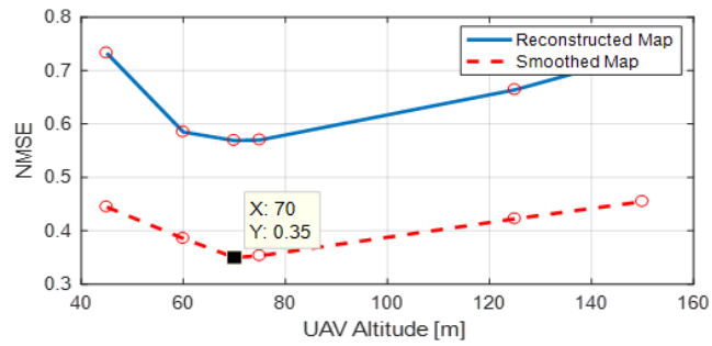
Figure 6.5 – Reconstruction normalised mean square error (NMSE) for both smoothed and rough map versus different UAV elevations.
