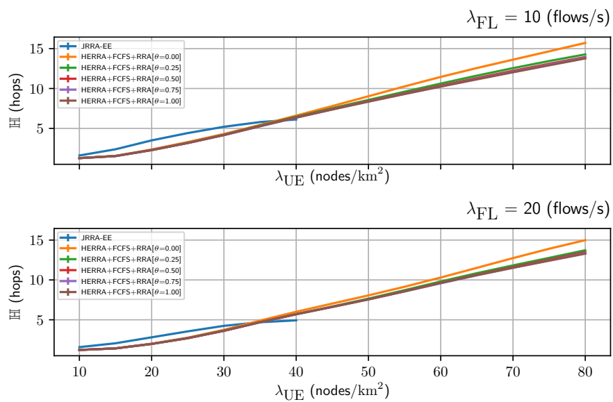
Figure 5.4 – Performance of HERRA with respect to the hop count \mathbb{H} .
