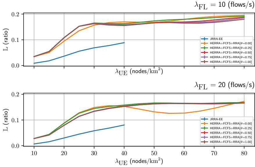
Figure 5.5 – Performance of HERRA with respect to the packet loss \mathbb{L} .
