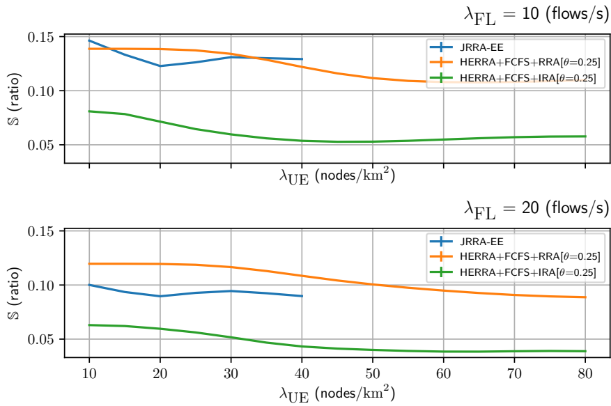
Figure 5.10 – Comparison between the strategies RRA and IRA with respect to the offloading ratio S .
