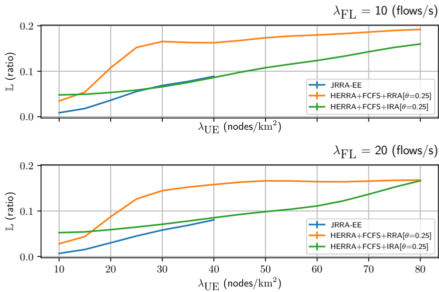
Figure 5.11 – Comparison between the strategies RRA and IRA with respect to the packet loss ratio L .
