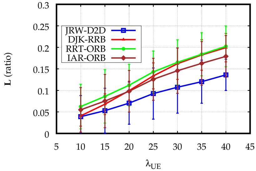
(a) \lambda_{FL} = 10
