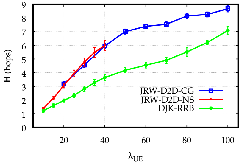
(b) \lambda_{FL} = 20
