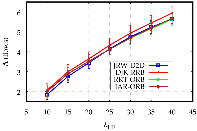
(b) \lambda_{FL} = 20
