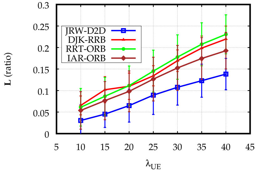
(b) \lambda_{FL} = 20
