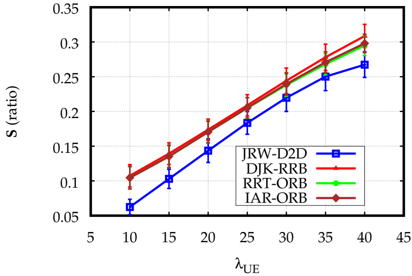
(b) \lambda_{FL} = 20
