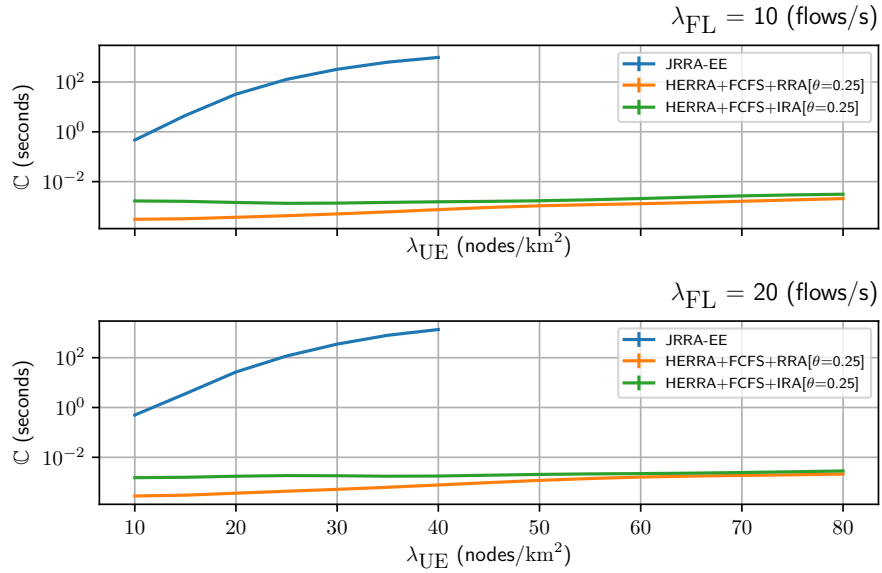
Figure 5.12 – Comparison between the offloading schemes time with regards to the computation time \mathbb{C} .
