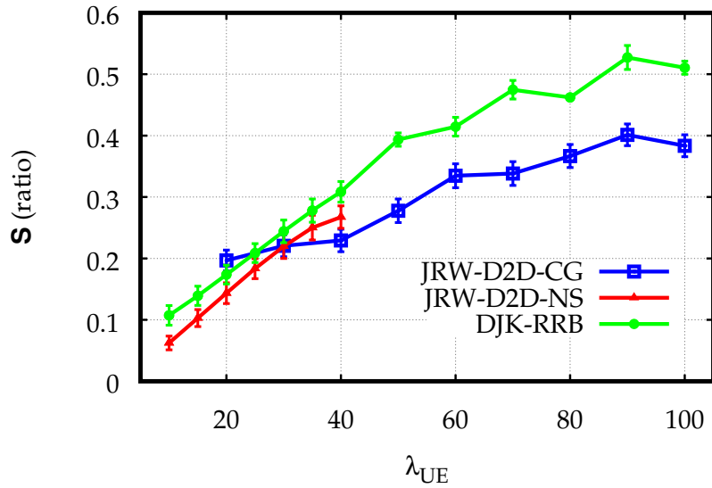
(b) \lambda_{FL} = 20
