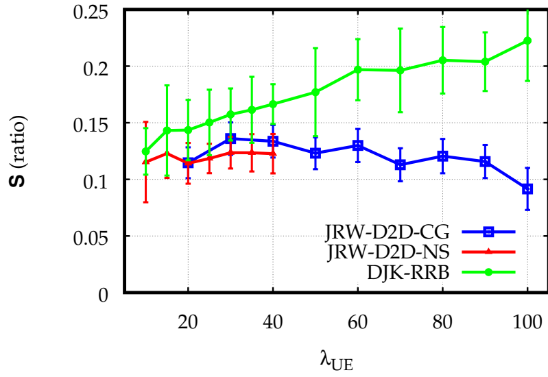
(a) \lambda_{FL} = 10
