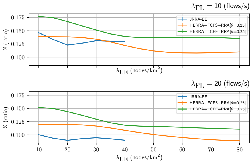
Figure 5.8 – Comparison between the strategies FCFS and LCFF with respect to the offloading ratio \mathbb{S} .
