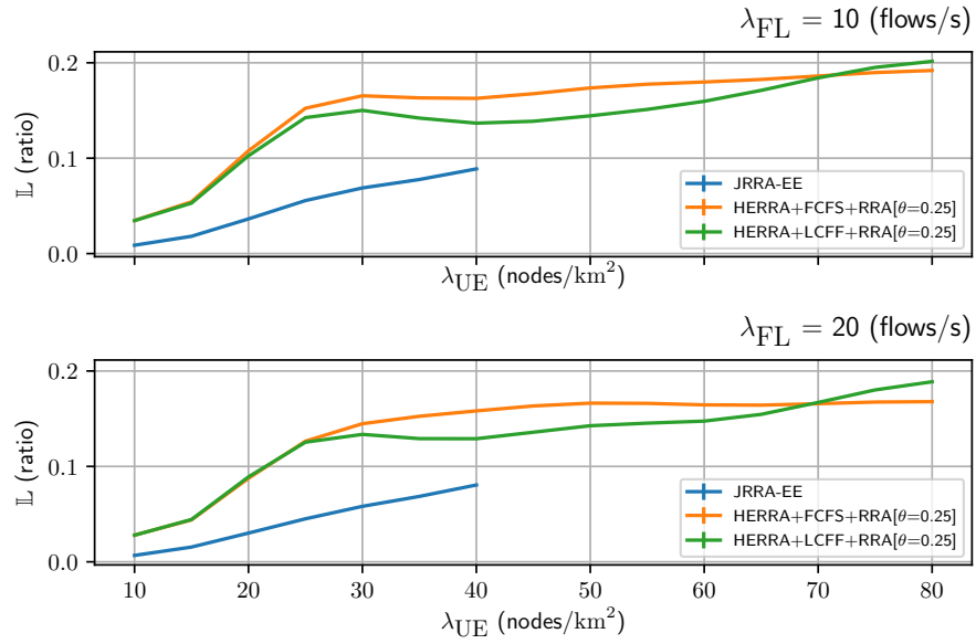
Figure 5.9 – Comparison between the strategies FCFS and LCFF with respect to the packet loss ratio \mathbb{L} .
