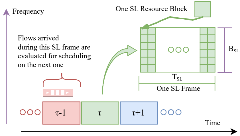
Figure 3.1 – Sidelink frame structure and scheduling
