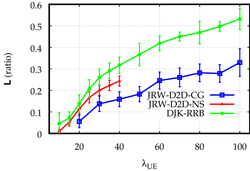
(a) \lambda_{FL} = 10
