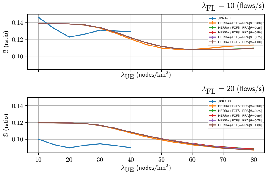
Figure 5.3 – Performance of HERRA with respect to the offloading ratio \mathbb{S} .
