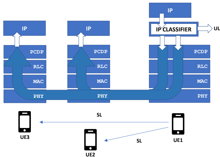
Figure 1.4 – LTE-D2D protocol stack for Direct Communications
