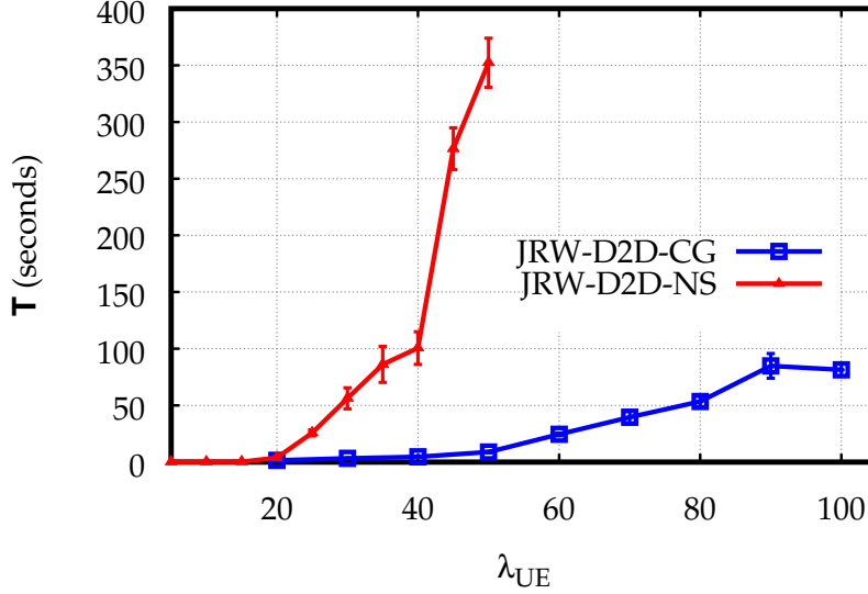
Figure 4.5 – The computation time metric T versus the nodes density \lambda_{UE} .
