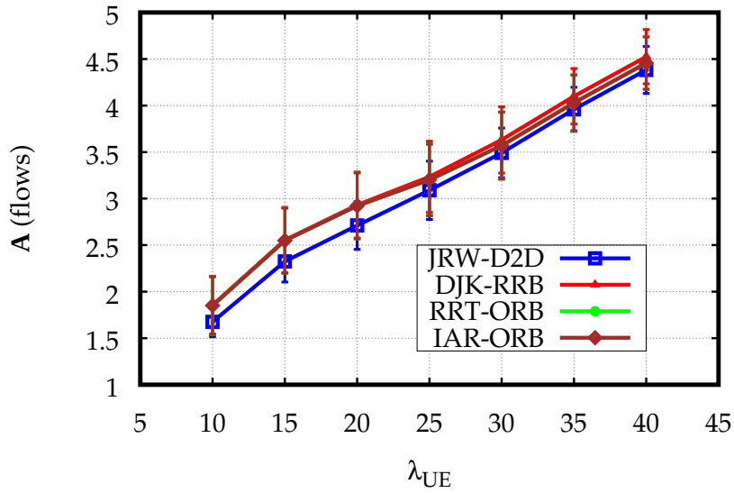
(a) \lambda_{FL} = 10
