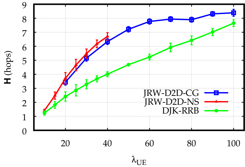
(a) \lambda_{FL} = 10
