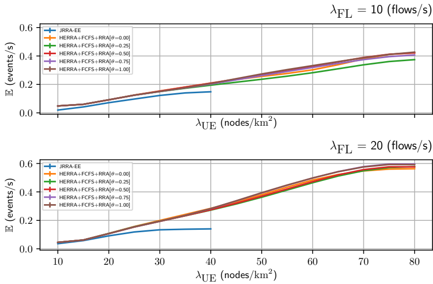
Figure 5.7 – Performance of HERRA with respect to the occurrence rate of the interruption event (node-exit) \mathbb{E} .
