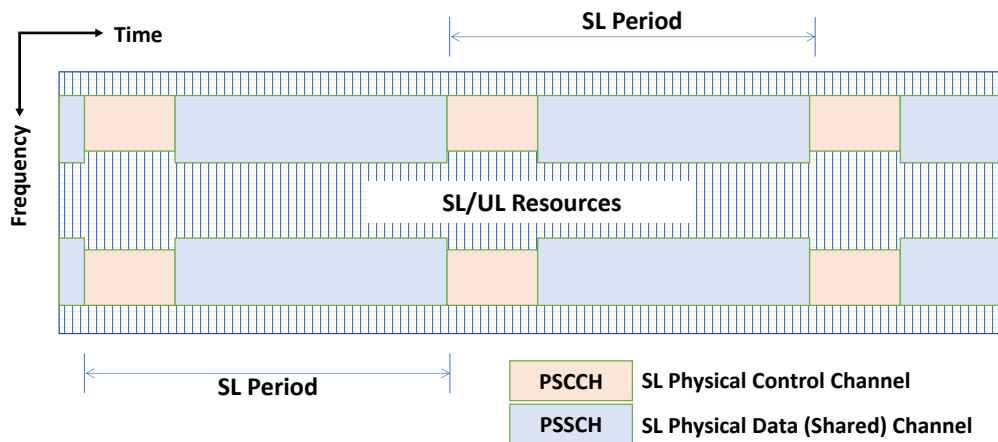
Figure 1.5 – SL channel structure in LTE-D2D (direct communications only)
