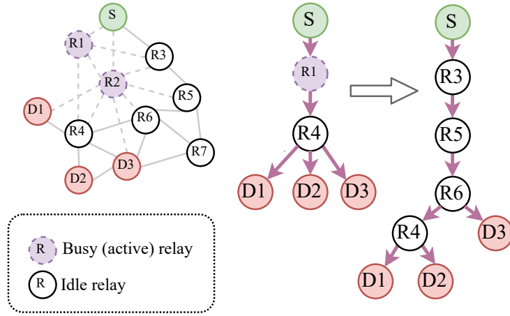
Figure 5.2 – Pre-routing tree formation and its deviation.
