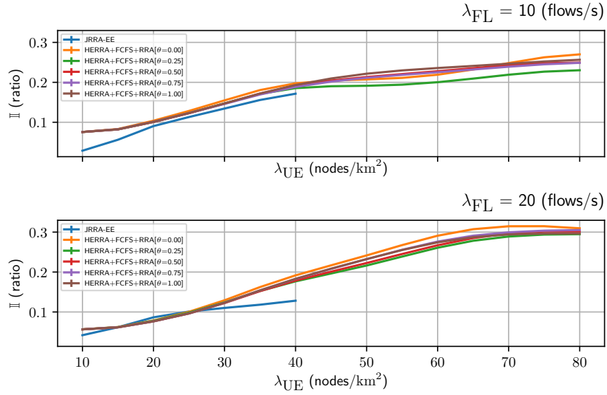
Figure 5.6 – Performance of HERRA with respect to the flow interruption ratio \ell .
