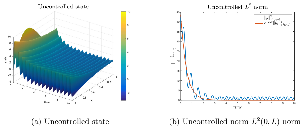
FIGURE 4.3: Uncontrolled state and its L^2 norm evolution.
