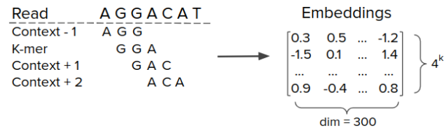
Fig. 3.3.: Left side represents a read cut into k-mers of length 3 with a window size of 2 and a padding size of 1. Right side corresponds to an embedding matrix of dimension 300 learnt with k-mers vocabulary of size 4^k = 4^3 = 64 .
