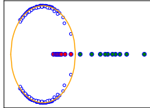
Spectrum of B for the football dataset [GN02]
