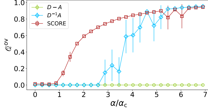
Figure 8.2: Overlap comparison as a function of the hardness of the detection of DCSBM-generated graphs with n = 10\,000 , c = 200 , k = 2 , \theta_i \sim [\mathcal{U}(3, 10)]^4 . Green dots correspond to SC as per [Fie73], light-blue diamonds as per [SMoo] and red dots as per [Jin+15]. Averages are taken over 10 samples.
