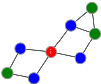
In red the node i , in blue its neighbours, in green the remaining nodes
