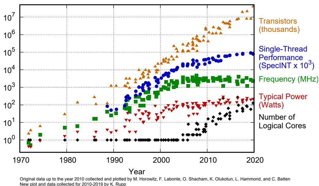
Figure 1.12: 42 years of microprocessor trend data [12].
