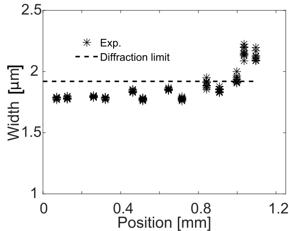
Figure 2.8: Width of the diffractive orders image according to the emitter position. Within an area of one millimeter in radius, the imaging system remains diffraction limited.
