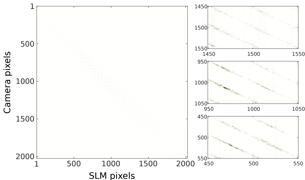
Figure 2.5: Recurrent neural network's coupling matrix \mathbf{W}^{\text{DOE}} established by the DOE. Each pixels of the SLM is coupled to its close neighbours. Due to the unfolding of 2D matrices of pixels into 1D vectors, the width of the diagonals corresponds to the coupling of nodes along the vertical axis, the vertical distance between the diagonals corresponds to the coupling along the horizontal axis. The three right insets are zooms into smaller regions. The intensity is normalized but is identical for the four panels.
