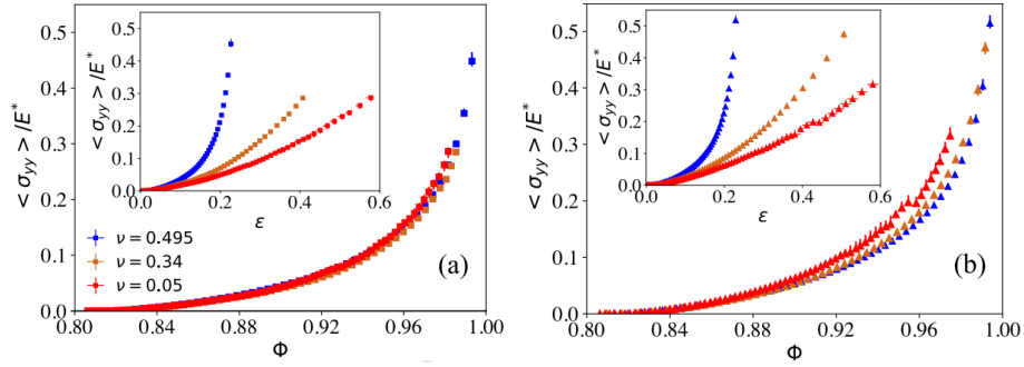
FIGURE 1.8. Stress in the y -direction scaled by the effective Young modulus of an oedometric compaction as a function of the packing fraction of particles with different Poisson ratios and friction coefficients equal to (a) \mu = 0.2 and (b) \mu = 0.8 [13].
