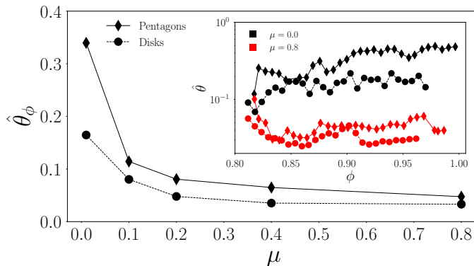
FIGURE 3.7. \hat{\theta}_\phi as a function of the friction coefficient for assemblies of pentagons (continuous line) and disks (dashed line). The inset shows the evolution of \hat{\theta} as a function of the packing fraction \phi for two different values of friction.
