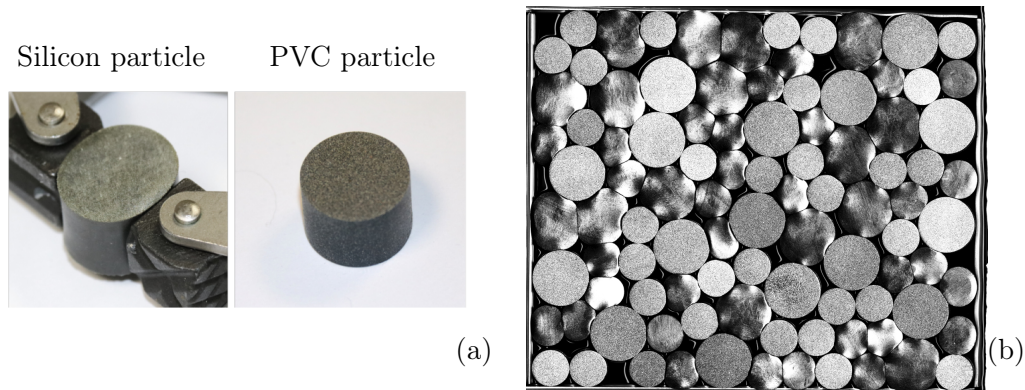
FIGURE 4.3. (a) Squeezed soft silicon particle and PVC particle used in the experiment. (b) Scan of a compressed random configuration of particles with soft/rigid mixture ratio \kappa = 0.5 .
