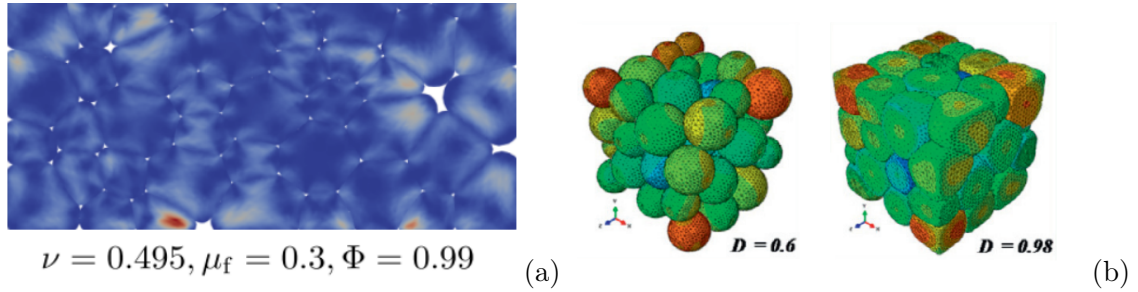
FIGURE 1.13. (a) Two-dimensional simulations of a frictional soft particle assembly under oedometric compression using NSCD. The color-intensity is related to the strain energy within the particles [20]. (b) Three-dimensional simulations of a soft particle assembly under oedometric compression using MPFEM [21]. In both cases, the color-intensity is related to the mean stress within the particles.
