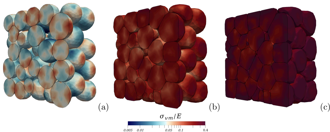
FIGURE 5.6. Three dimensional cross-section of the stress P_n at each node of the particles and for different packing fraction \phi = 0.66 (a), \phi = 0.86 (b) and \phi = 0.96 (c), respectively, in the assembly of 100 particles. The color intensity is proportional to the von Mises stress scale by the Young modulus, \sigma_{vm}/E .
