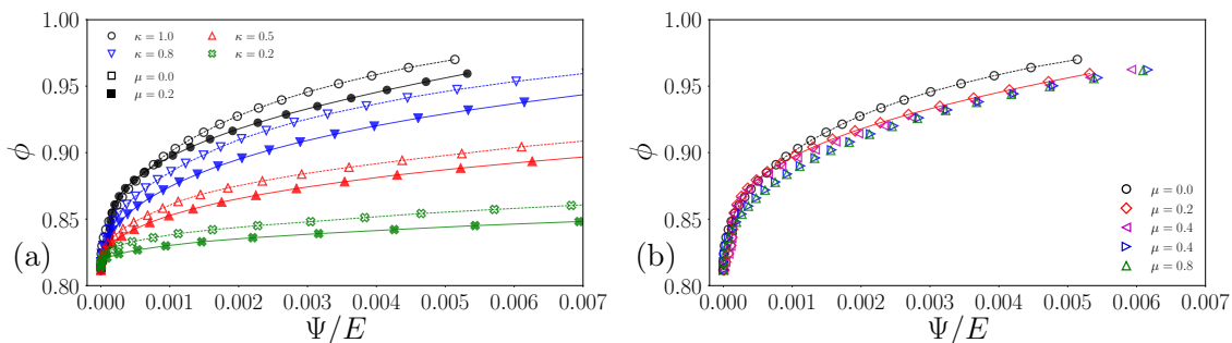
FIGURE 2.11. Packing fraction as a function of the mean strain energy density of the soft particles normalize by the Young modulus for (a) different mixture ratios with \mu = 0.0, 0.2, and for (b) different friction coefficient with \kappa = 1.0 .
