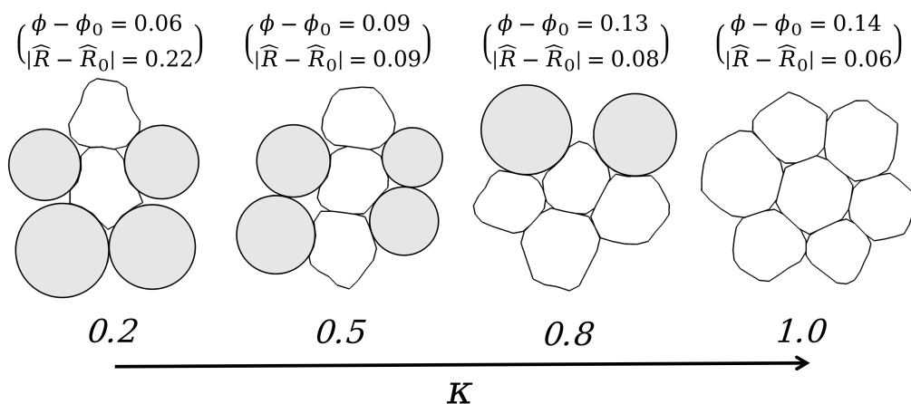
FIGURE 2.9. Group of particles extracted from the different mixture packings, showing the mean circularity value very close to the maximal packing fraction. The rigid particles are colored in gray.
