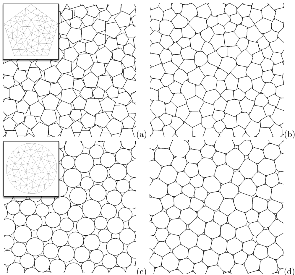
FIGURE 3.1. Close-up views of the assembly of pentagons (a,b) and disks (c,d) at \mu = 0 and for P/E = 0.025 (a,c) and P/E = 0.3 (b,d). The insets of (a) and (c) show the finite element mesh used for both pentagons and disks, respectively.
