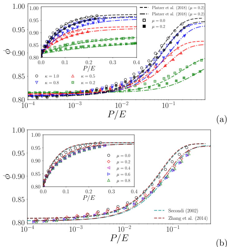
FIGURE 2.3. Evolution of the packing fraction \phi as a function of P/E for (a) rigid-deformable particles assemblies with \kappa \in [0.2, \dots, 1] and \mu \in \{0, 0.2\} , and for (b) completely deformable particle assemblies (i.e., \kappa = 1 ) with \mu \in \{0, 0.8\} . Main panels are in lin-log scale while insets show curves in lin-lin scale. Numerical data (symbols) are shown with fits of Platzer et al.'s model [16] for rigid-deformable particles and Secondi's model [11], and Zhang's model [24] for the fully deformable systems (dashed lines).
