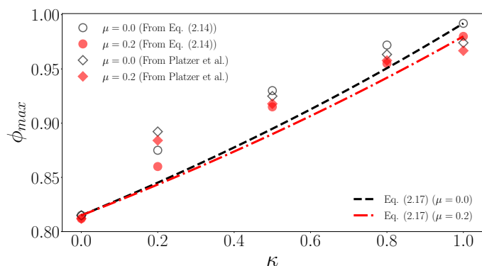
FIGURE 2.5. Values of \phi_{max} fitted with Platzer et al.'s model (diamond symbols) and with Eq. (2.14) (circular symbol, see Section 2.4 ) on the compaction curves of rigid-deformable particle assemblies shown in Fig. 2.3(a), for different \kappa and \mu \in \{0, 0.2\} . The dashed lines show the prediction given by Eq. (2.17).
