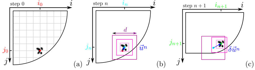
FIGURE 4.4. Schematic view of the digital image correlation algorithm for large deformations on an individual particle. On the initial image at step 0 (a), a regular grid is placed on the particle. The system is deformed from the step n and displacement field \mathbf{u}_i^n (b) to the step n + 1 (c) by a small \delta \mathbf{u}^n increment such that the new displacement field is \mathbf{u}_i^{n+1} = \mathbf{u}_i^n + \delta \mathbf{u}_i^n .
