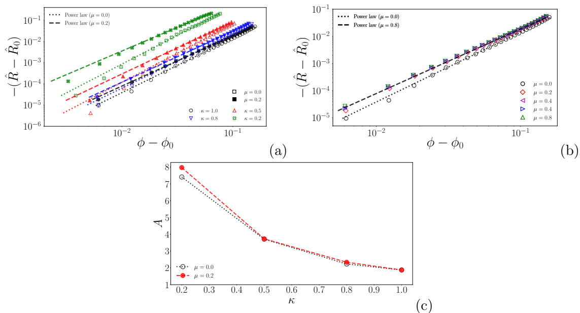
FIGURE 2.8. Evolution of (\hat{R} - \hat{R}_0) as a function of (\phi - \phi_0) for different values of (a) mixture ratio \kappa and (b) friction coefficient \mu for \kappa = 1.0 . The dotted and dashed line are the power-law fittings for \mu = 0.0 and \mu = 0.2 , respectively. (c) Power law's prefactor, A , as a function of the mixture ratio \kappa for coefficients of friction equal to 0.0 and 0.2.
