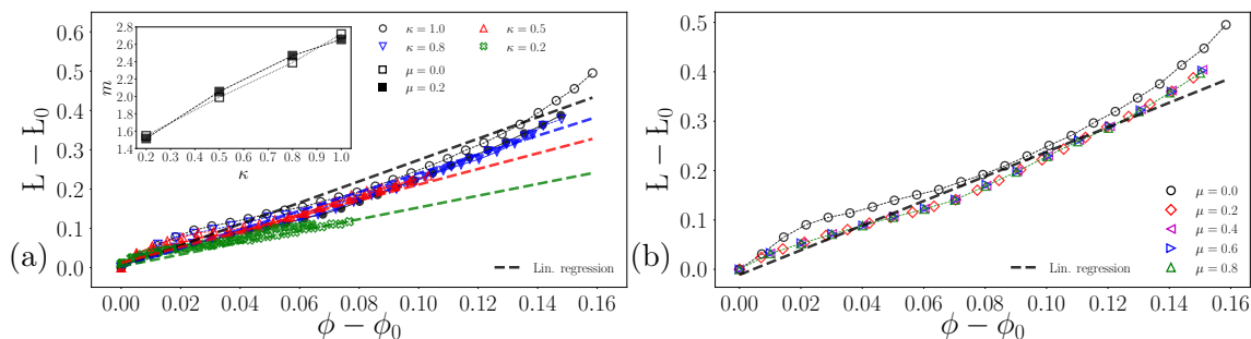
FIGURE 2.10. Evolution of the excess of the average contact length L - L_0 as a function of the excess packing fraction \phi - \phi_0 for different values of (a) mixture ratio \kappa and (b) friction coefficient \mu for \kappa = 1.0 . The dashed lines in both figures are linear fits of the evolution. The inset in (a) shows the slope m of the linear fits for the different mixture ratio \kappa . In (b) the linear fit has a slope \sim 2.6 .
