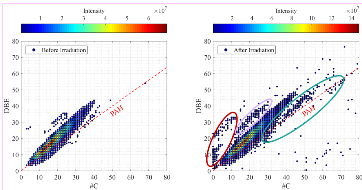
Figure VI.9: Double Bond Equivalent (DBE) as a function of number of C atoms ( \#C ) present in the molecules. The DBE gives an idea of the unsaturation level of the molecules. The color bar corresponds to the intensity of the molecules. The red dashed line corresponds to the theoretical DBE expected for a polymer purely composed of Poly-Aromatic Hydrocarbons (PAH). Left: Before SHI irradiation. Right: After irradiation with 75 MeV ^{136}\text{Xe} swift heavy ions at a fluence of 1 \times 10^{14} \text{ cm}^{-2} . The red, lavender color and turquoise circles indicate new molecules formed after SHI irradiation.
