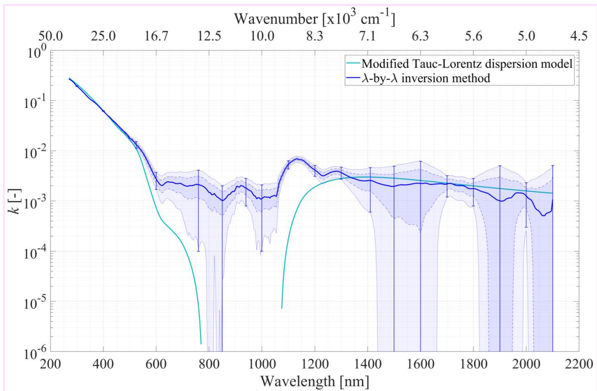
Figure V.2: Same as Figure V.1, but showing the imaginary part k of the complex refractive index. The 2\sigma error bars were experimentally determined for the “ \lambda -by- \lambda ” inversion method at different wavelengths. The uncertainties were then linearly interpolated between two error bars in order to obtain the envelope of 2\sigma uncertainty (in light blue). The envelope determined by dashed lines corresponds to 1\sigma uncertainty. Note that the y-axis was cropped at 10^{-6} , while the 2\sigma uncertainties of k -values reach 0 in the [800-850], [1,450-1,650] and [1,820-2,100] nm regions.
