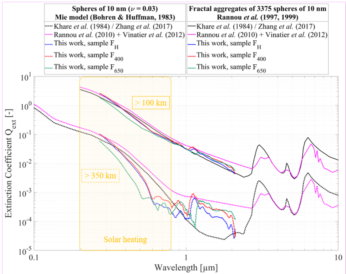
Figure V.8: Extinction coefficients Q_{\text{ext}} determined for spherical monomers of 10 nm radius (log-normal distribution, with effective variance \nu = 0.03 ) with a Mie model formalized in Bohren and Huffman (1983) (dotted curves) and for fractal aggregates of 3,375 monomers of 10 nm radius with the model developed by Rannou et al. (1997, 1999) (plain curves). The black curves were generated with the optical constants determined by Khare et al. (1984) for Titan tholins. Note that these Khare et al. (1984) optical constants were adopted in Zhang, Strobel and Imanaka (2017) study. The pink curves were generated with the optical constants determined by Rannou et al. (2010) and Vinatier et al. (2012) for Titan's aerosols. The blue, red and green curves were generated with the optical constants determined respectively for my samples F_H , F_{400} and F_{650} . The yellow rectangle indicates the region where solar heating dominates. The dotted curves (spherical monomers) give information on the radiative transfer in the upper layers of Pluto's atmosphere ( > 350 km of altitude), while the plain curves (fractal
