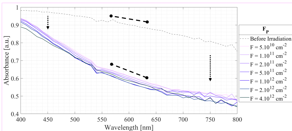
Figure VI.5: In situ monitoring of the spectrum in the visible spectral range of Pluto tholins F_P before (dashed grey curve) and after sequential irradiations with increasing fluences “F” (purple cameo curves) by 75 MeV ^{136}\text{Xe} swift heavy ions. The bold black dashed lines are indicative to the average slopes in the [570-630] nm region. The visible spectra were acquired with a Perkin Elmer Lambda 650 UV-Vis spectrometer.
