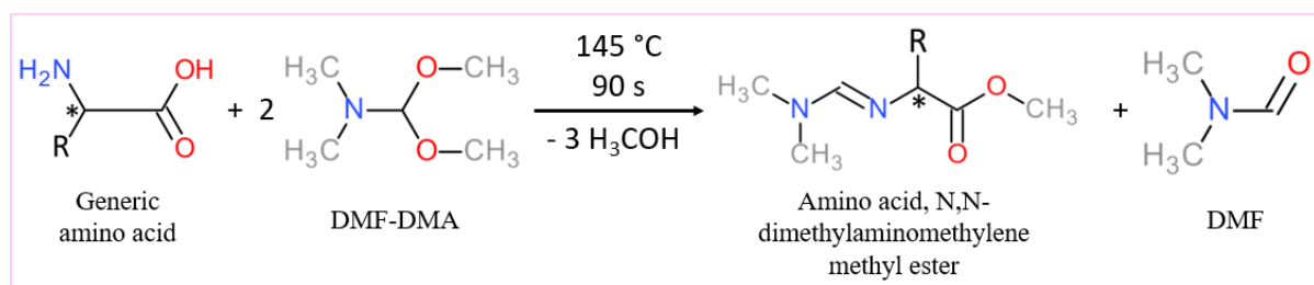
Figure II.22: Derivatization reaction between a generic amino acid and DMF-DMA. The asterisk (*) corresponds to a chiral center; if existing, then it is conserved.
